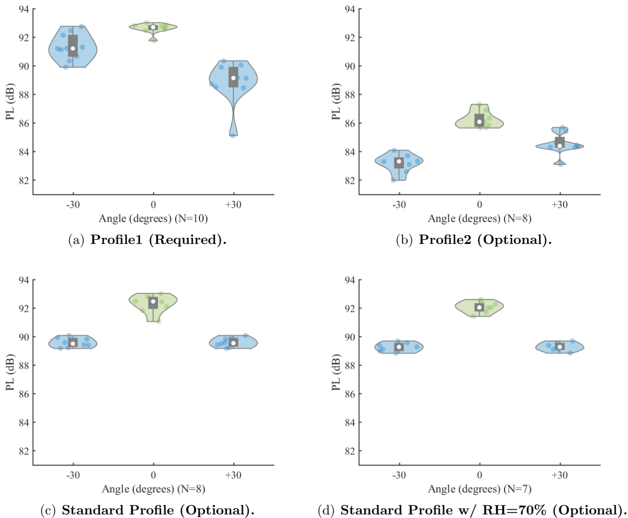
Figure 27. Violin plots of Perceived Level (PL) for LM1021 separated by atmospheric conditions and by angles.
