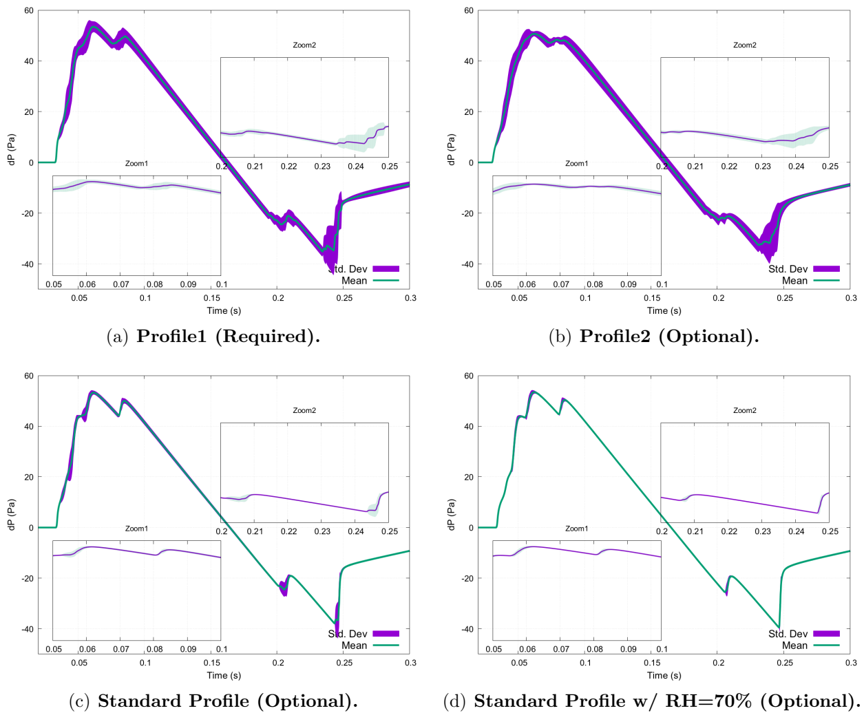
Figure 22. Mean and Standard deviation of Ground Signatures for LM1021 at Roll Angle = 0°
