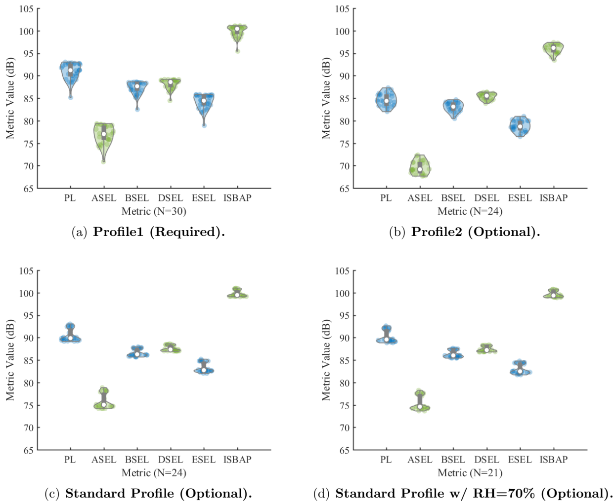
Figure 26. Violin plots of noise metrics for LM1021 separated by atmospheric conditions (all angles grouped together).
