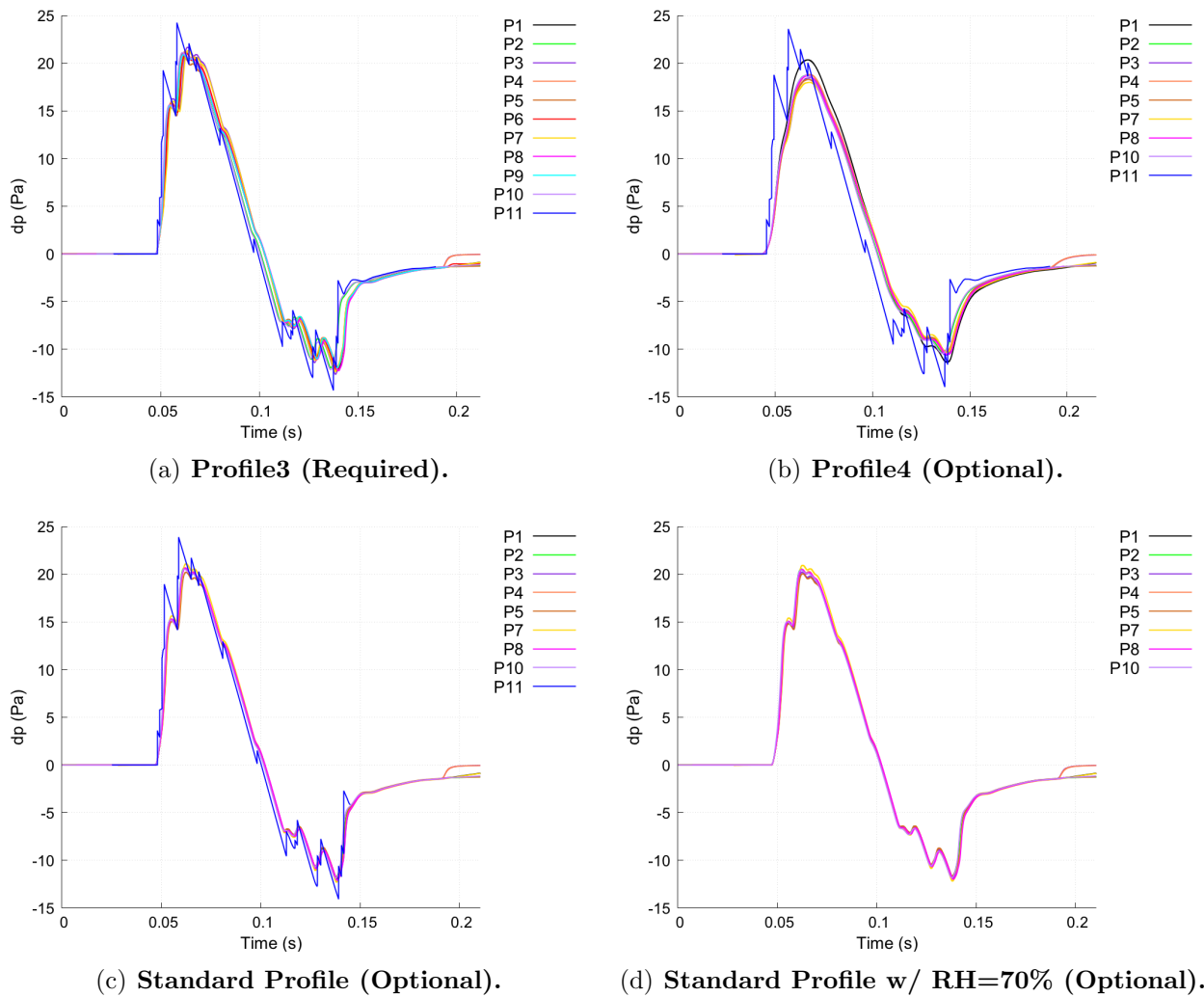
Figure 28. Ground Signatures for AXIBODY at Roll Angle = 0°
