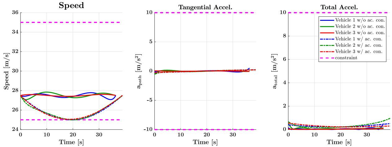
Fig. 3 Vehicle speed and acceleration as a function of mission time.
