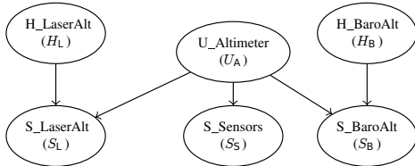
Fig. 2. Sensor failure detection BN from [6]
