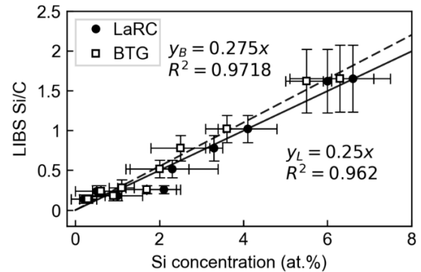
Figure 3. Analytical calibration curves with the Si/C ratio from the LIBS measurements and the Si concentration using XPS. The linear fits y_L (solid line) and y_B (dashed line) correspond to LaRC and BTG, respectively. (Reprinted from [8] with permission of SAGE Publishing)
