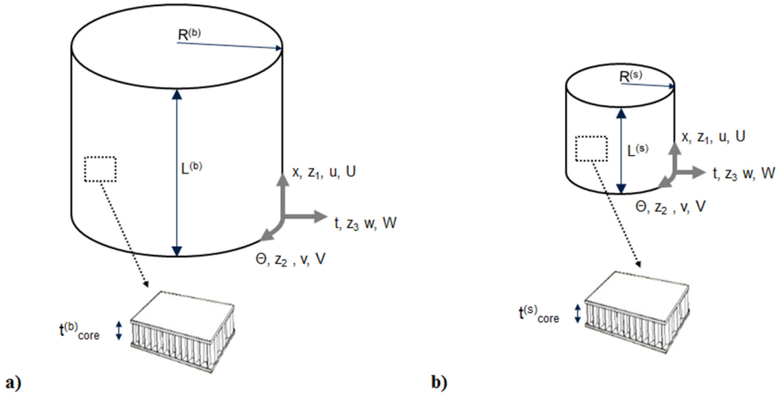
Fig. 1 Geometry and coordinate system: a) Baseline configuration and b) scaled configuration.
