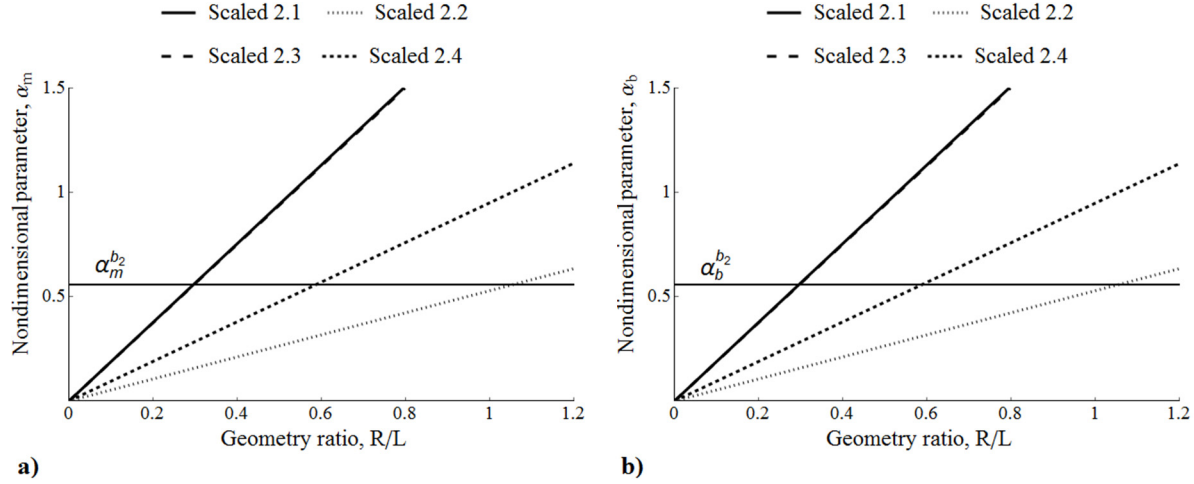
Fig. 5 Parameters: a) \alpha_m and b) \alpha_b versus R/L for scaled facesheet stacking sequences for Baseline 2 [30/-30/90/0] s .
