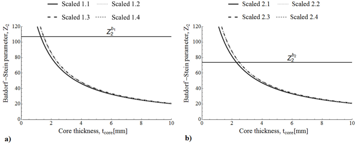
Fig. 6 Batdorf-Stein parameter Z_2 as function of core thickness t_{core} for a) Baseline 1 and b) Baseline 2
