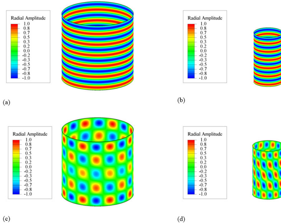
Fig. 7 First linear buckling mode: a) Baseline 1, b) Scaled 1.1, c) Baseline 2 and d) Scaled 2.1.
