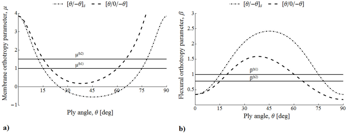
Fig. 2 Orthotropy parameters: a) Membrane, \mu , and b) flexural, \beta , versus ply angle \theta for scaled facesheet stacking sequences [\theta/-\theta]_s and [\theta/0/-\theta] .
