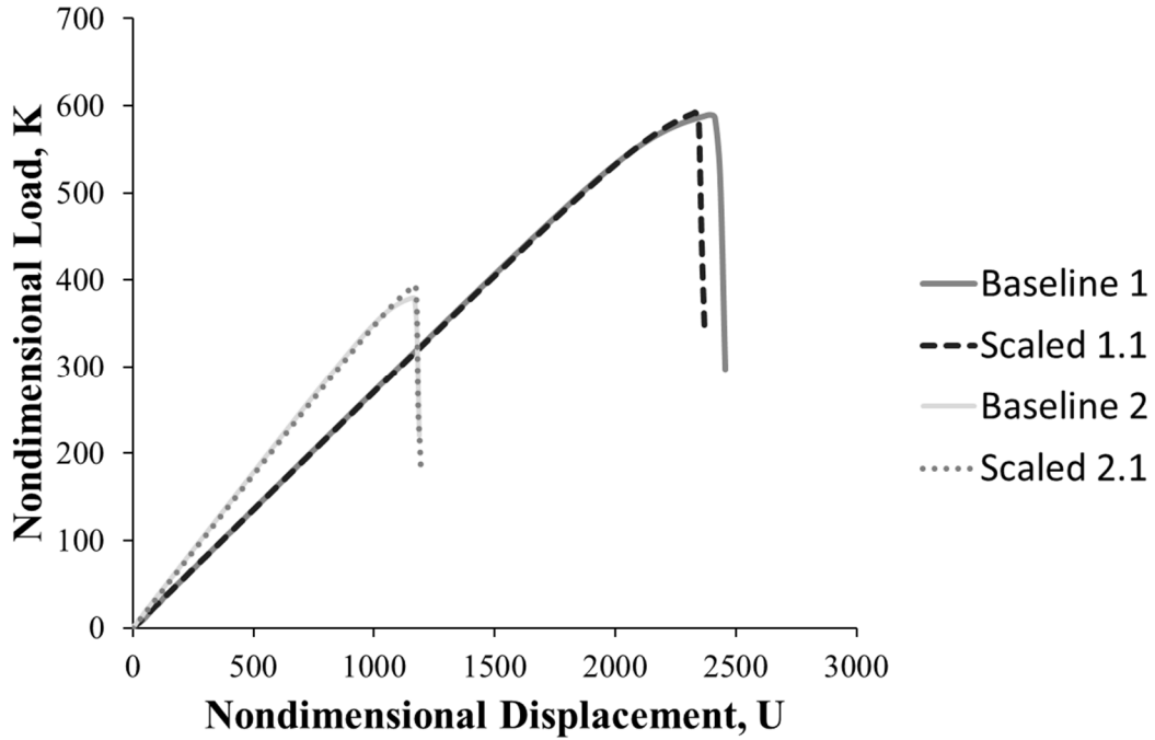
Fig. 9 Nondimensional load-displacement curves of baseline and scaled.
