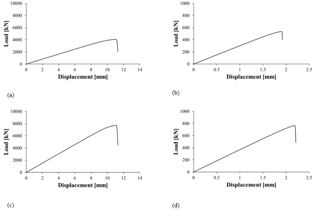
Fig. 8 Load-displacement curves from finite element analysis: a) Baseline 1, b) Scaled 1.1, c) Baseline 2 and d) Scaled 2.1.
