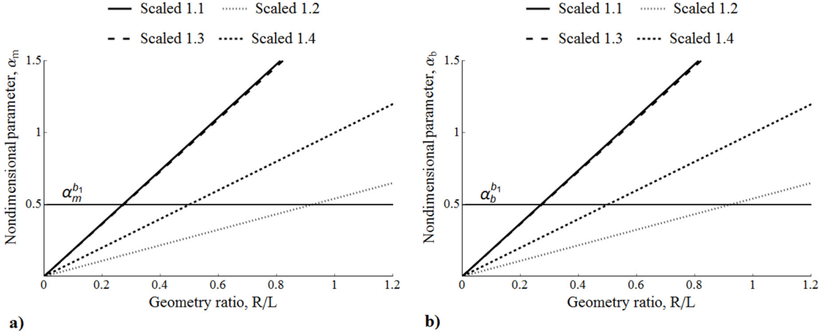
Fig. 4 Parameters: a) \alpha_m and b) \alpha_b versus R/L for scaled facesheet stacking sequences for Baseline 1 [60/-60/0]_s .
