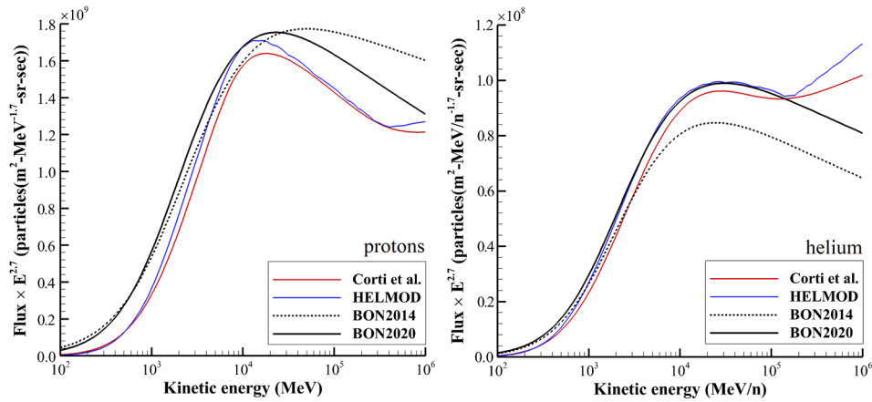
Figure 15. Comparison of LIS from BON2014, BON2020 and other parametric models for protons and helium.
