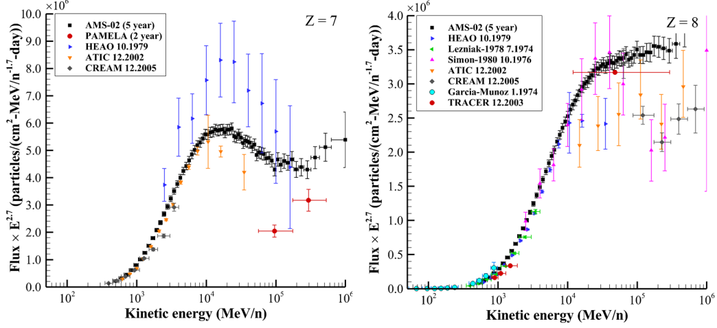
Figure 7. Z = 7 (left) and Z = 8 (right) measurement data.
