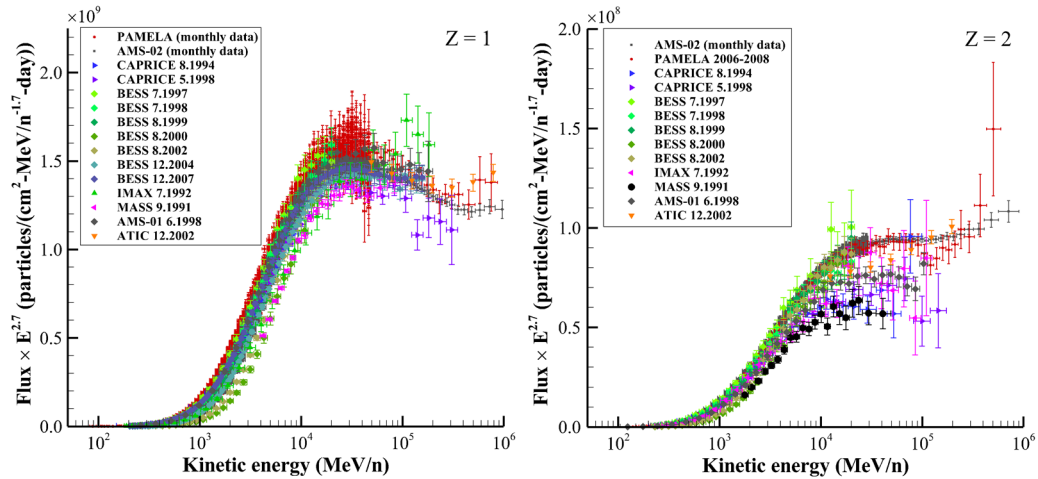
Figure 6. Z = 1 (left) and Z = 2 (right) measurement data.
