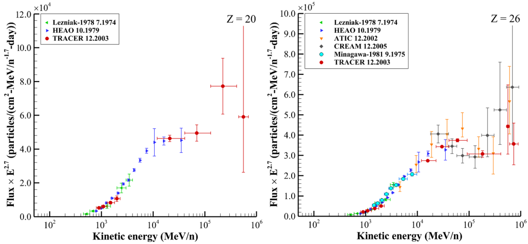
Figure 8. Z = 20 (left) and Z = 26 (right) measurement data.
