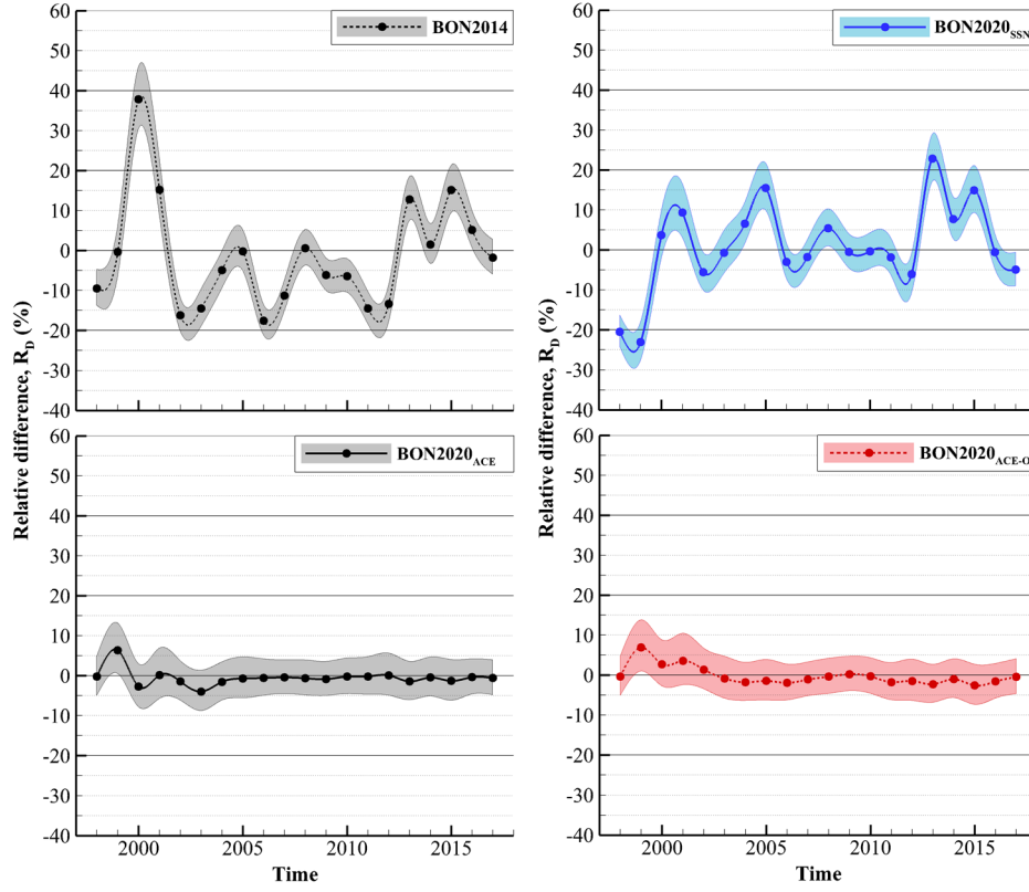
Figure 14. Average model relative differences compared to ACE/CRIS data for Z = 5 - 28 as a function of time. The shaded regions are closely related to measurement uncertainty.
