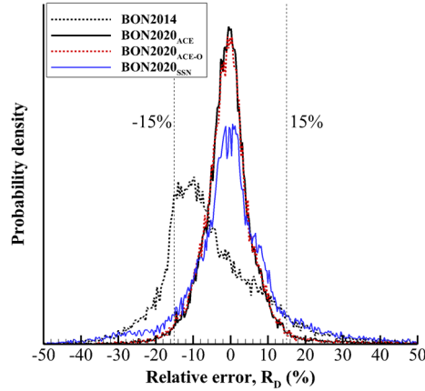
Figure 9. Distribution of model errors against all available measurements.
