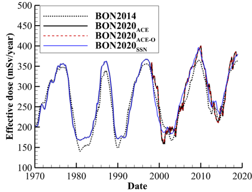
Figure 17. Female effective dose versus time behind 20 g/cm 2 aluminum shielding using different GCR models.
