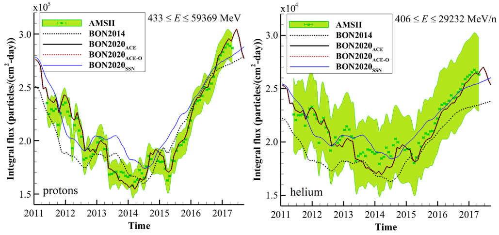
Figure 11. Model integral flux compared to AMS-02 measurements. The shaded region represents total measurement uncertainty.
