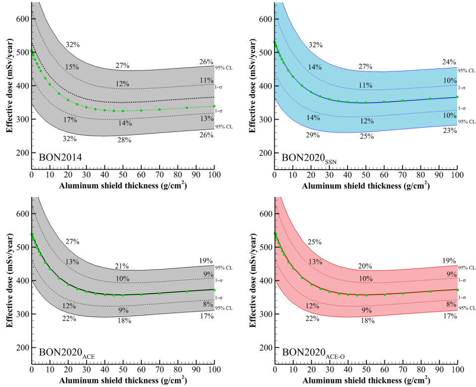
Figure 16. Female effective dose versus shield thickness for the June 1, 2009 – June 1, 2010 solar minimum. The green dashed line with circles is the nominal model result, while the shaded region indicates the distribution of effective doses resulting from uncertainty in the GCR model. Specific intervals of the distributions and relative differences at specific depths are shown.
