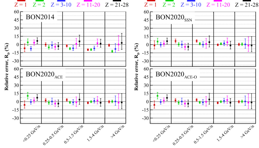
Figure 10. Average model relative error separated into energy groups indicated on the horizontal axes and charge groups indicated with different colored symbols. The error bars are closely related to measurement uncertainty.
