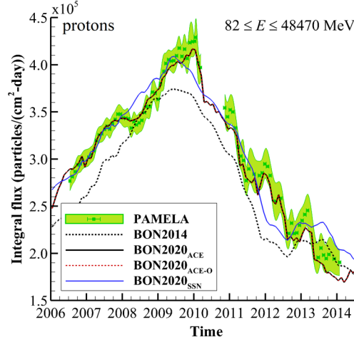
Figure 13. Model integral flux compared to PAMELA measurements. The shaded region represents total measurement uncertainty.
