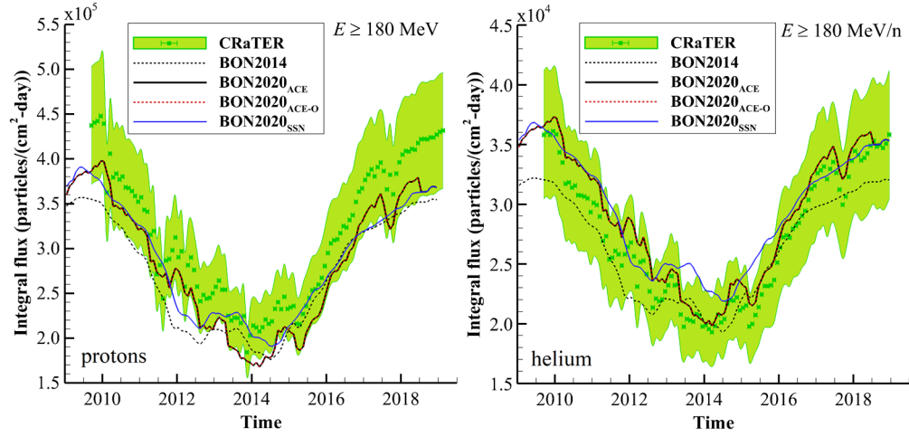
Figure 12. Model integral flux compared to CRaTER measurements. The shaded region represents total measurement uncertainty.
