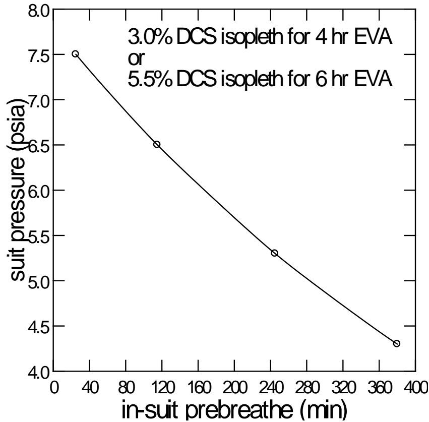
Fig. 12. Relationship between suit pressure and in-suit prebreathe time to achieve P(\text{DCS}) isopleths after 4 and 6 hours of simulated ambulatory EVA. Note: you must add 30 minutes to the in-suit prebreathe time to account for the additional prebreathe on going from 14.7 psia to final suit pressure.
