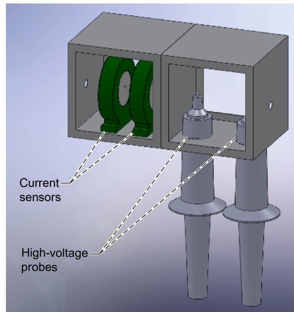
Figure 28.—Anode voltage and current probe arrangement.
