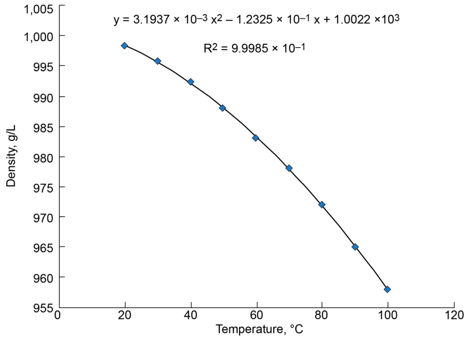
Figure 33.—Water density from 20 to 100 °C. u|\text{density}| = (-6.387 \times 10^3 T - 0.12325) uT where T = ^\circ\text{C} and uT = \pm^\circ\text{C} .
