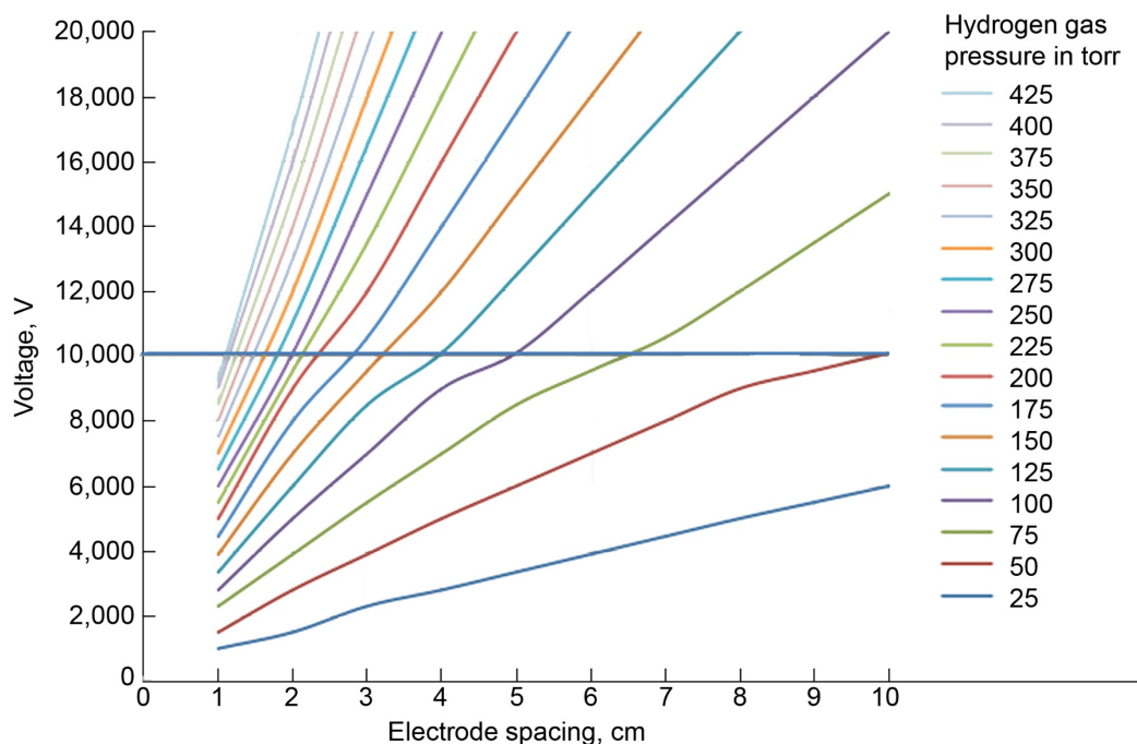
Figure 3.—Required breakdown voltage for hydrogen at different pressures.
