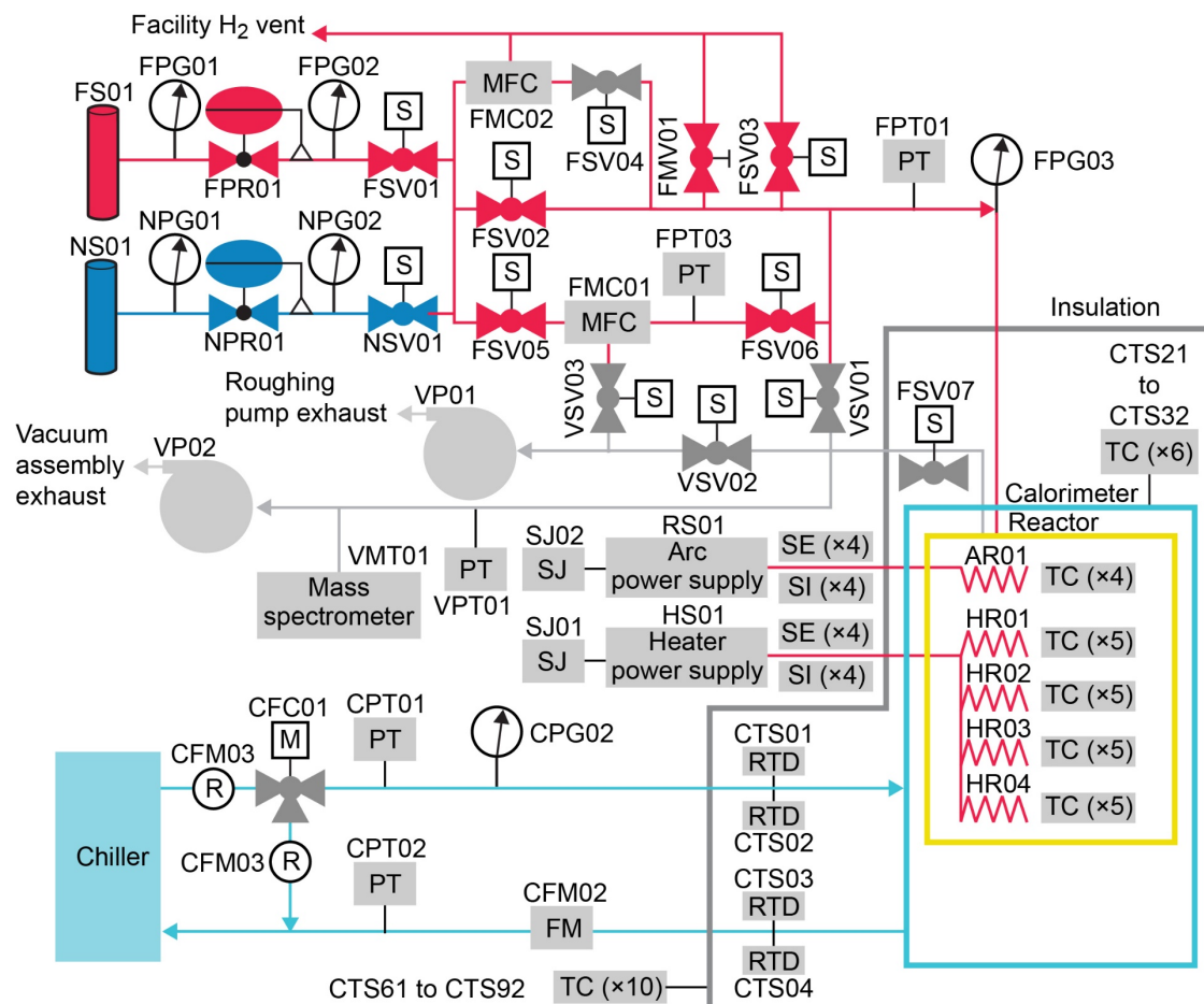
Figure C.1.—Plasma II reactor test rig, revision H.
