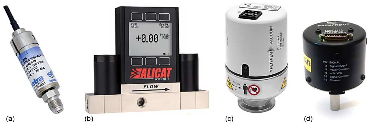
Figure 31.—Pressures sensors, gauge, and controller. (a) Setra® 225 pressure sensor. (b) Alicat Scientific PCD pressure controller. (c) Pfeiffer Vacuum PKR 251 FullRange™ Pirani/Cold Cathode Gauge. (d) MKS Instruments Baratron® Type 122A pressure transducer.
