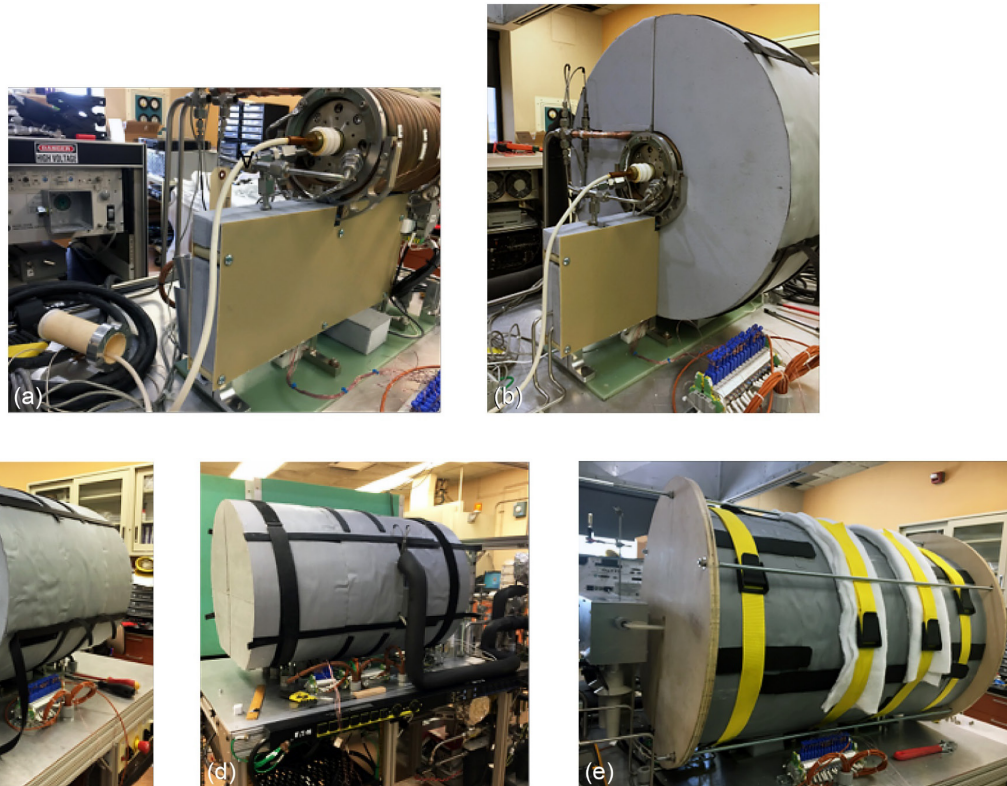
Figure 66.—Reactor insulation wrap steps. (a) Insulation wrap around frame. (b) Insulation wrap around central body of reactor. (c) Velcro® straps securing center insulation. (d) Endcap insulation and securing Velcro® straps. (e) Completed and secured insulation.
