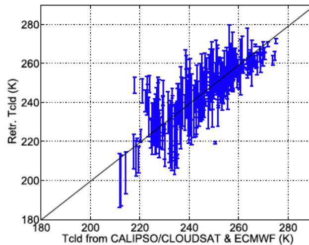
Cloud top Temp. retrieval validation using IASI + CALIOP/CLOUDSAT/ECMWF
