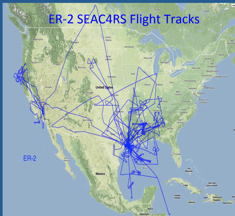
ER-2 Flight Tracks
