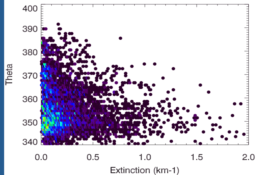
CALIOP Extinctions - Marine
