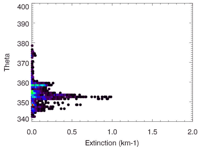
FCDP Extinctions - Marine
