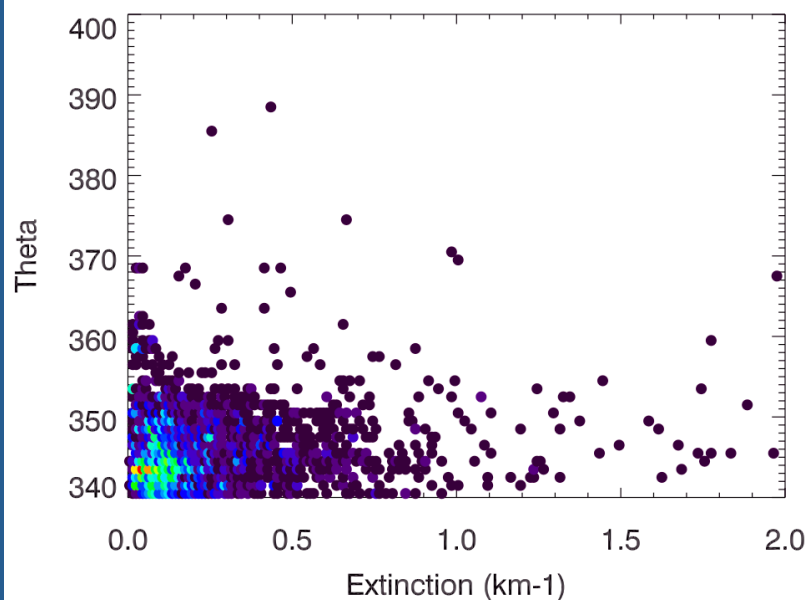
CALIOP Extinctions - Land
