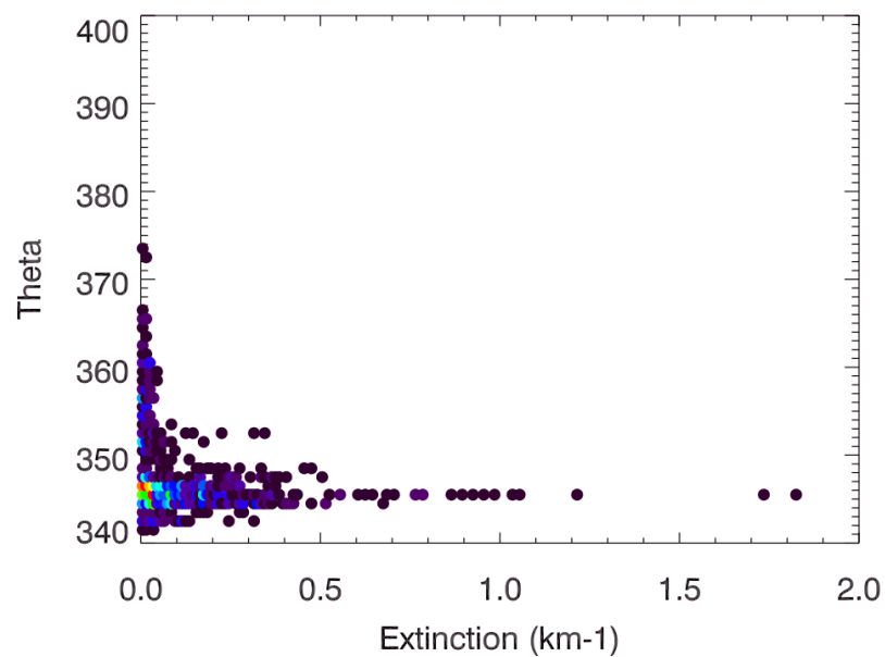
FCDP Extinctions - Land
