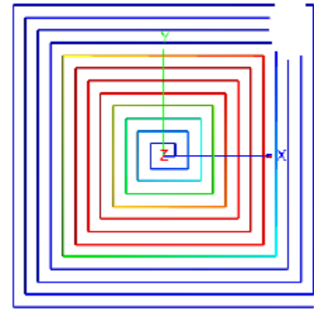
Damaged Sensor Current Distribution
