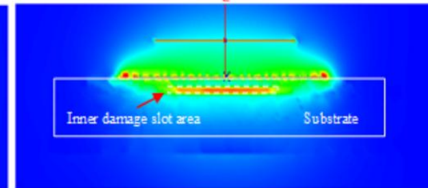
Electric field distribution With Damage ( \epsilon_r=3 )
