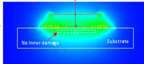
Electric field distribution No Damage ( \epsilon_r=3 )
