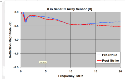
(B) Sensor B upper right quadrant.
