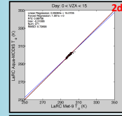
Figs 2d, 2e, 2f, 2g, 2h, and 2i) Same as Fig 2c , except limited to solar zenith angles less than 80^\circ , and stratified in VZA groupings of 0 < \text{VZA} < 15^\circ , 15 < \text{VZA} < 30^\circ , 30 < \text{VZA} < 40^\circ , 40 < \text{VZA} < 50^\circ , 50 < \text{VZA} < 60^\circ , and \text{VZA} > 60^\circ . The unbiased scheme ( Fig 2c ) is used rather than the true relationship ( Fig 2a ) because the correction model should be solely dependent on varying viewing and illumination conditions, and should not be influenced by biases introduced by small differences in skill owed to subtle changes between the GEO and LEO skin temperature retrieval methodologies.
