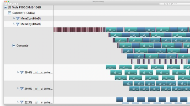
Fig. 8. Execution timeline of SP-MZ Class C on Cori as seen on the profiler
