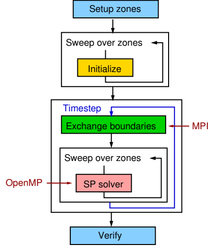
Fig. 1. Execution flow of the SP-MZ Benchmark
