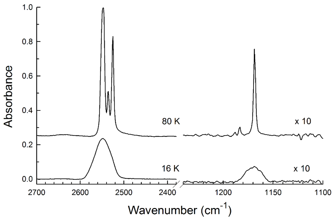
Figure 2. The stretching (left) and bending (right) regions of the IR spectrum of amorphous (lower) and crystalline (upper) H 2 S. The ice's thickness was about 4 μm..
