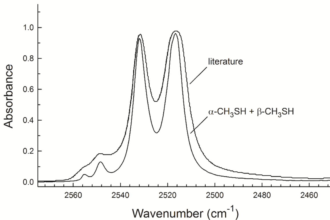
Figure 9. Comparison of a recently published IR spectrum of crystalline CH 3 SH (Pavithraa et al. 2017b) to a combination of our spectra of the \alpha - and \beta -crystalline phases of CH 3 SH (Hudson 2016). The fractional contributions are about \alpha = 0.55 and \beta = 0.45 .
