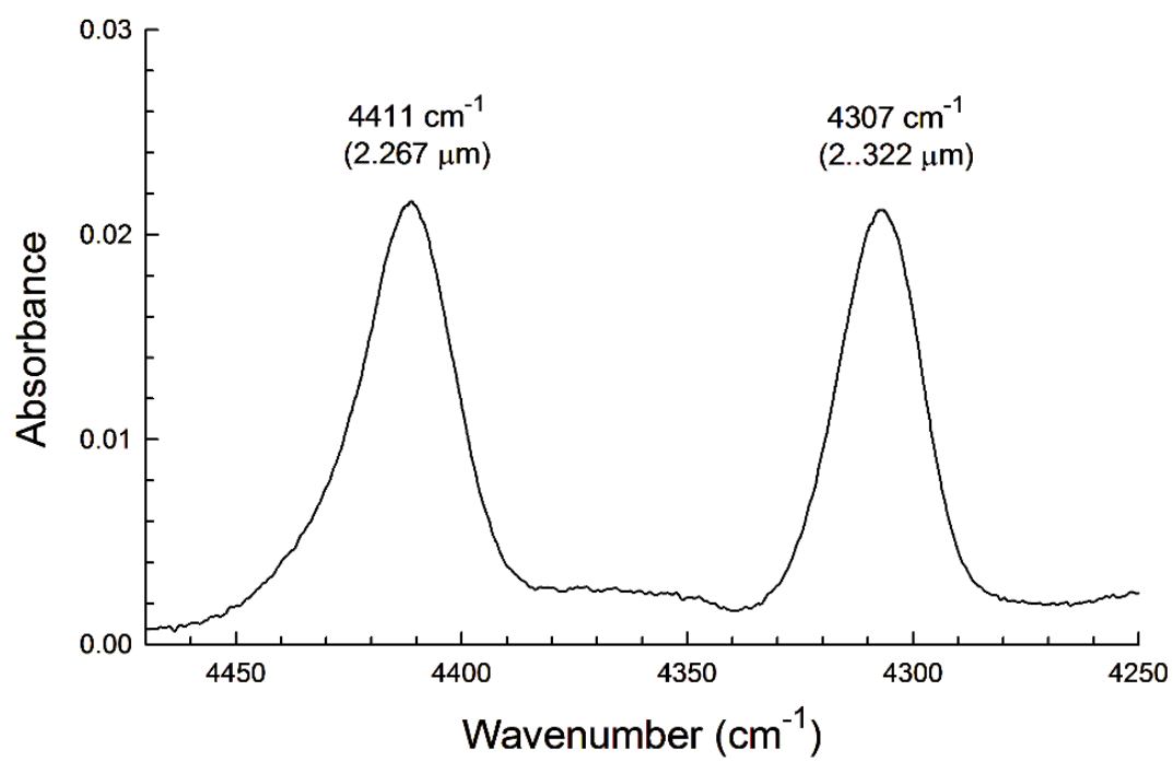
Figure 7. Two near-IR bands of amorphous CH 3 SH deposited at 10 K. The sample's thickness was about 3.8 μm.
