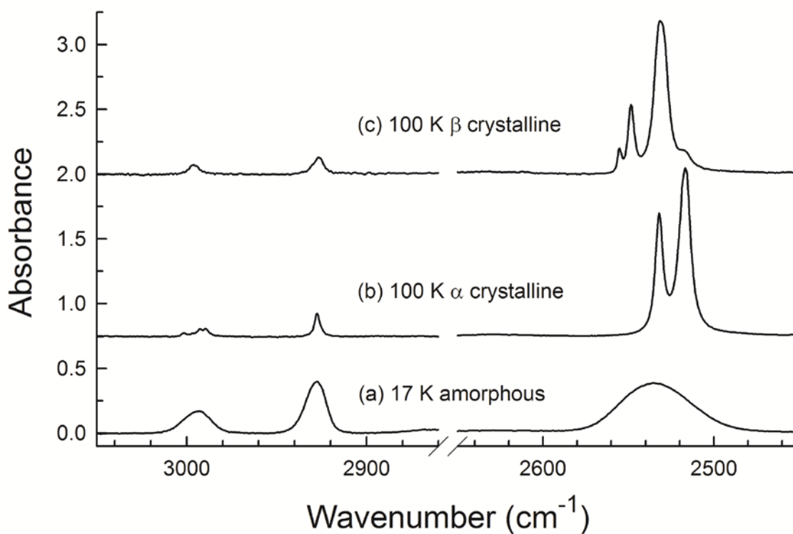
Figure 3. The C-H (left) and S-H (right) stretching regions of the IR spectra of solid CH 3 SH at 17 K for the amorphous phase and at 100 K for the \alpha - and \beta -crystalline phases. The thickness of the amorphous ice was about 7 \mu\text{m} . See Hudson (2016) for details of crystalline-CH 3 SH band strengths. Spectra are offset vertically for clarity.
