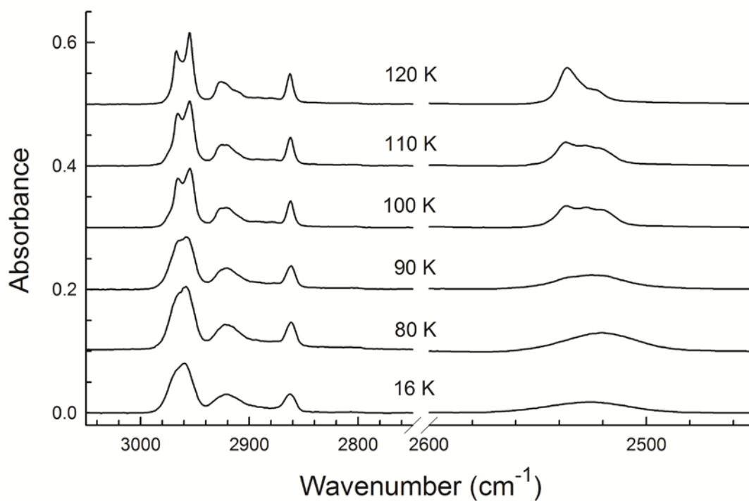
Figure 6. The C-H and S-H stretching regions of the IR spectra of solid (CH 3 ) 2 CH(SH) deposited at 16 K and then warmed to the temperatures indicated. The sample's original thickness was about 4.5 μm. Spectra are offset vertically for clarity.
