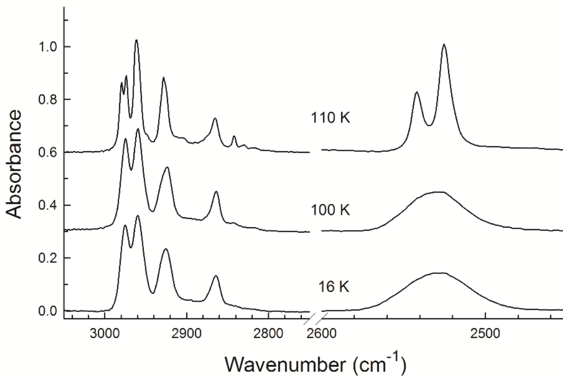
Figure 4. The C-H (left) and S-H (right) stretching regions of the IR spectra of solid \text{CH}_3\text{CH}_2\text{SH} deposited at 16 K and warmed to 100 and 110 K. The sample's original thickness was about 4.4 \mu\text{m} . Spectra are offset vertically for clarity.
