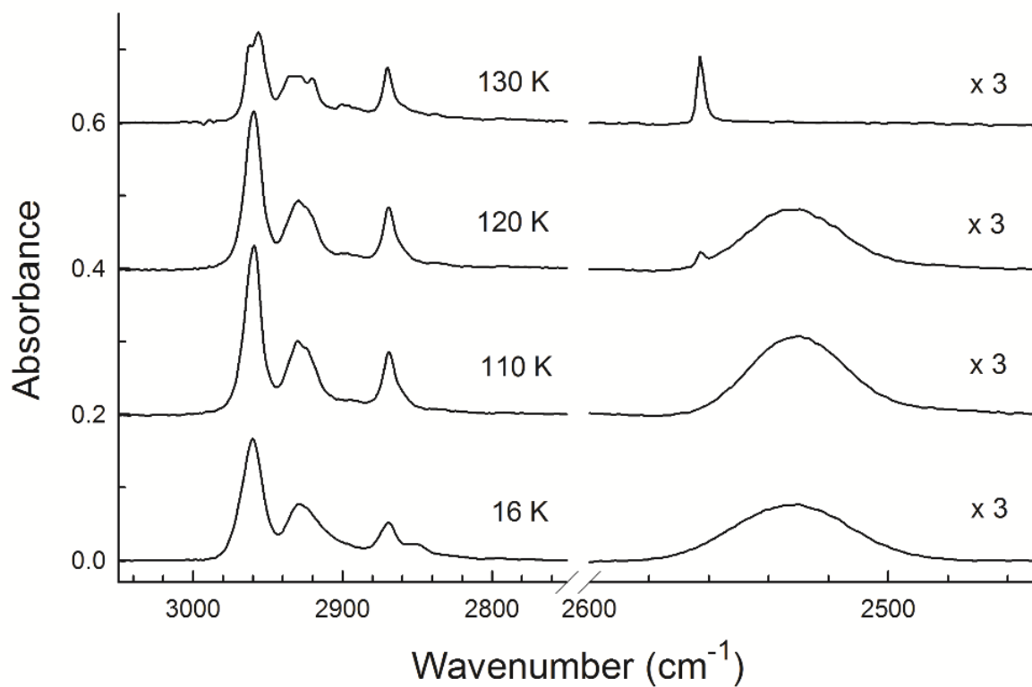
Figure 5. The C-H and S-H stretching regions of the IR spectrum of solid \text{CH}_3\text{CH}_2\text{CH}_2\text{SH} deposited at 16 K and warmed to 110, 120, and 130 K. The sample's original thickness was about 4.5 \mu\text{m} . Spectra are offset vertically for clarity and the right-hand side has been expanded by a factor of 3 (vertically).
