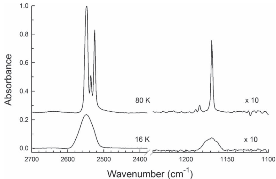
Figure 2. Stretching (left) and bending (right) regions of the IR spectrum of amorphous (lower) and crystalline (upper) \text{H}_2\text{S} . The ice's thickness was about 4\ \mu\text{m} .
