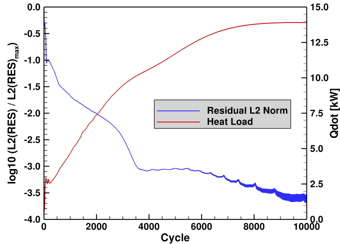
Figure 8: Convergence history for the backward facing step problem.
