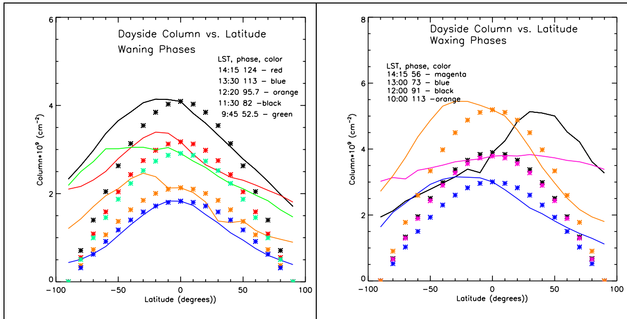
Figure 4. Zenith column abundances from the surface for waning phases (left) and waxing phases (right). There is no obvious variation in column abundance with time of day. Column abundances at the equator vary from about 1.5 \times 10^9 \text{ cm}^{-2} to \sim 5.5 \times 10^9 \text{ cm}^{-2} .
