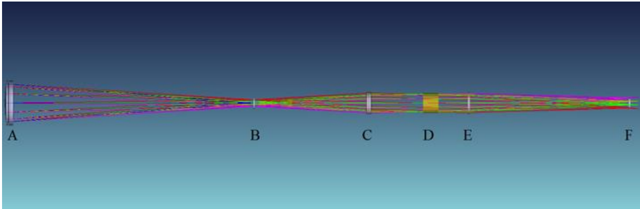
Figure A1. Optical path for the coronagraph. A. Objective Lens; B. Field lens with occulting disk; C. Collimating lens; D. Filter; E. Reimaging lens F. CCD Detector.
