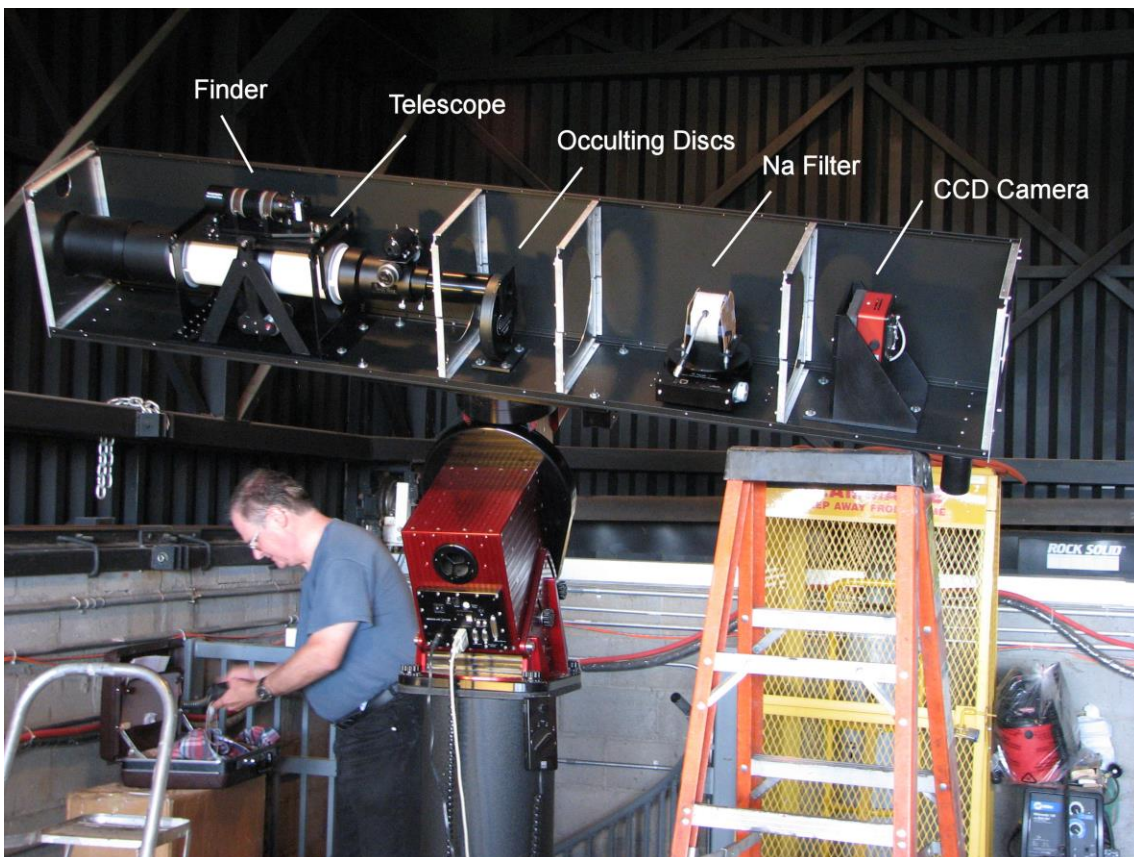
Figure A2. Coronagraph with cover removed showing the layout. Roy Tucker is shown assembling the coronagraph.
