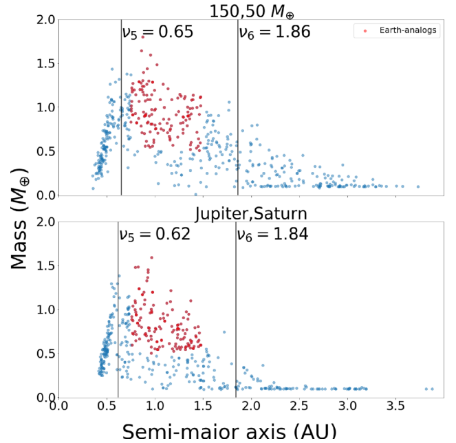
Figure 10. Remaining embryo mass ( M_\oplus ) and semimajor axis (au) for the Jupiter and Saturn, and 150 and 50 M_\oplus systems after \sim 500 Myr. The \nu_5 secular resonance induced by the planet at Jupiter’s orbit and \nu_6 secular resonance induced by the planet at Saturn’s orbit are shown in solid black lines. The red dots are the Earth analogues. We find a similar distribution of the Earth analogues between the two systems.
