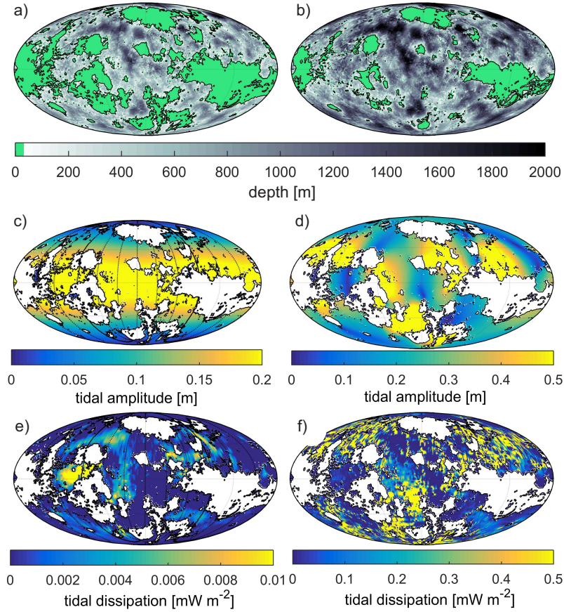
Figure 1. a)–b) The ocean bathymetry (depth in m; land is green) for the two configurations. a) shallow; b) deep. Note that the depth scale saturates in the deep oceans – in the shallow simulation the deepest point is 2340m. c) Solar tidal amplitudes (in meters) in a present day ocean on Venus from the shallow simulation. d) As in c) but for the simulation with an 8-earth day prograde rotation rate. Note the different color scales between panels. e–f) As in panels c–d, but showing the tidal dissipation rate in \text{mW m}^{-2} .
