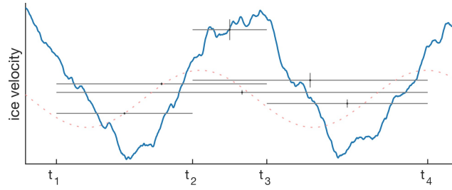
Figure 1. Example scenario: For a true continuous ice velocity time series like the one shown in blue, feature tracking measures velocity as the total displacement that occurs between satellite images of the flowing ice. Here, four images taken at times t_1 through t_4 provide six unique combinations of image pairs that yield six velocity measurements, which are depicted as horizontal gray lines connecting the acquisition times of each image pair. Vertical gray lines show measurement uncertainty and a black dot is placed at the center times of each image pair for visual clarity. The pink dashed sinusoid is fit to velocity measurements at the center times of each image pair to highlight the inadequacy of fitting directly to velocity data to determine the amplitude or phase of seasonal variability. This paper describes an alternate, exact approach, wherein sinusoids are fit to accumulated displacements rather than velocity time series.
