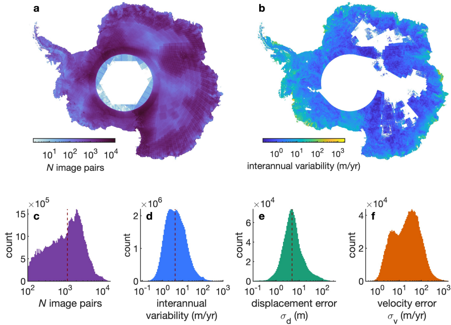
Figure 3. ITS_LIVE velocity data statistics. Maps of a : the number of image pairs that contribute to each 240×240 m pixel in the ITS_LIVE summary velocity mosaic and b : the standard deviation of annual velocity mosaics from 2013 to 2018. Histograms in panels c and d show only the values from a and b that correspond to grid cells with at least 100 contributing image pairs and whose mean velocity is at least 15 m yr -1 . Displacement errors \sigma_d shown in panel e result from satellite image georegistration error, and when divided by values of \Delta t corresponding to each image pair results in the velocity errors \sigma_v shown in panel f . Because displacement errors are distributed symmetrically, the bimodal distribution of velocity errors roughly correspond to the two peaks of \Delta t values over which velocity is measured (shown in Fig. 2). Vertical lines in panels c – e indicate median values of 1153 image pairs per grid cell, 4.2 m yr -1 interannual variability, and 4.9 m displacement error.
