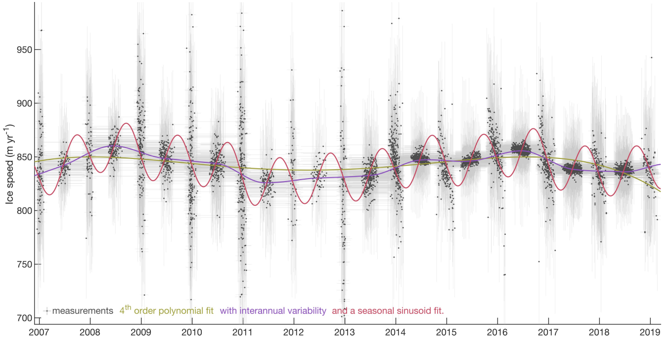
Figure 4. Velocity time series for an ITS_LIVE pixel. The cluster of these 14,208 measurements taken near the grounding line of Byrd Glacier typifies ITS_LIVE image pair data, with short delta time measurements providing direct, but noisy observations of velocity during the dark, winter months. Light gray horizontal bars connect the acquisition times of each image pair and vertical bars show \pm 1\sigma_v uncertainty. Center dates t_m are shown as dark gray dots for visual clarity.
