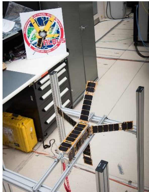
Figure 22: Fully Integrated Flight System SYSTEM GROUND TESTING
