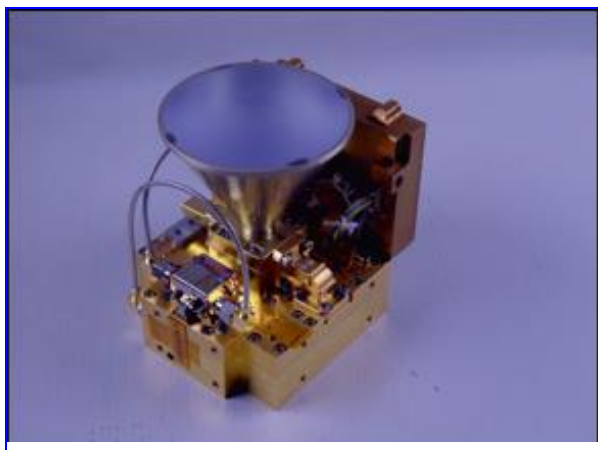
Figure 7 Astro Digital DVB-S2 Communications System
