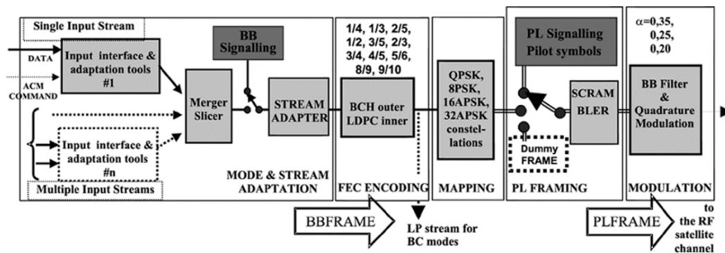
Figure 2 DVB-S2 Transmission System Block Structure
