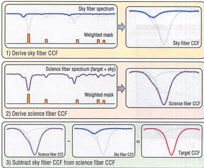
Figure 5. Overview of the direct sky fiber cross-correlation CCF subtraction technique, as described in Section 3.1. The CCF of the sky fiber is computed by cross-correlation with a numerical mask (top) and subtracted from the CCF of the science fiber spectrum (middle). The final target RV is derived from the resultant corrected target CCF (bottom). This technique has the advantage of simplicity, although it does inherently rely on the sky and science fiber PSFs being similar. Note that the spectrum and CCF continuum levels are matched for illustrative purposes only; in reality, the sky fiber has a much lower flux level.
