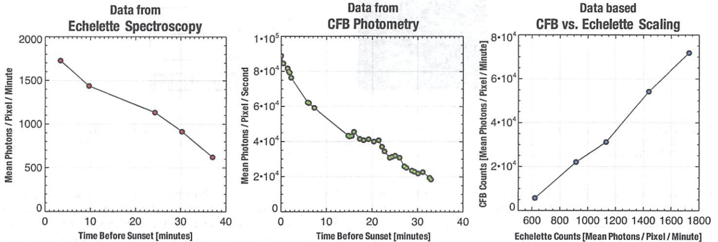
Figure 10. On-sky proof of concept that a relationship can be established between the sky fiber spectrum and broadband images from the CFB, as predicted in Figure 9. Data were taken as the Sun set to collect exposures at different sky brightnesses. Left: mean photons per extracted pixel in the echelette sky spectrum; all exposures have been scaled to 1 minute. Middle: number of photons per pixel in a CFB V-band image of the sky; all exposures are scaled to 1 second. Right: relation between the flux in the spectrum and the broadband CFB image, proving a clean linear scaling that can be extended to fainter skies. Note that the CFB counts are binned to 1 minute for direct comparison.
