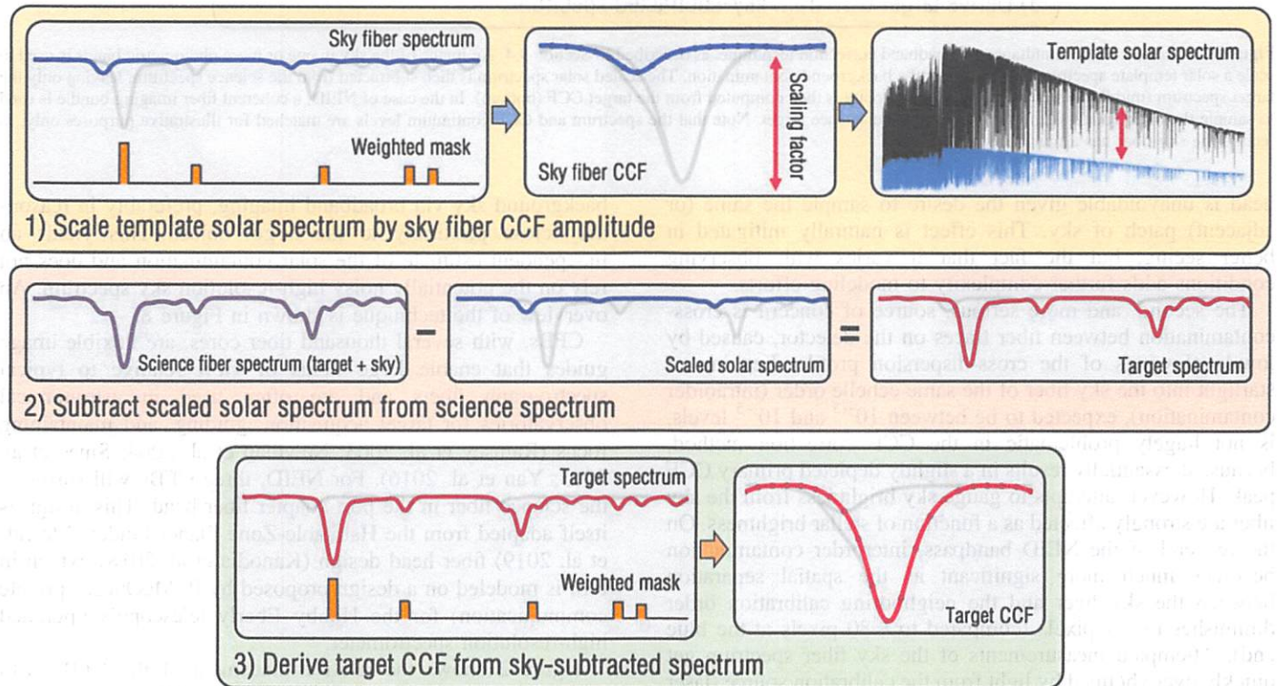
Figure 7. Overview of the model sky subtraction technique, as described in Section 3.2. The CCF of the sky fiber is computed using a numerical mask and used to scale a synthetic or high-S/N solar spectrum to the estimated sky brightness (top). The scaled spectrum is then subtracted from the science spectrum, leaving only the target spectrum (middle). The final target radial velocity is then computed from the target CCF (bottom). Note that the spectrum and CCF continuum levels are matched for illustrative purposes only; in reality, the sky fiber has a much lower flux level.
