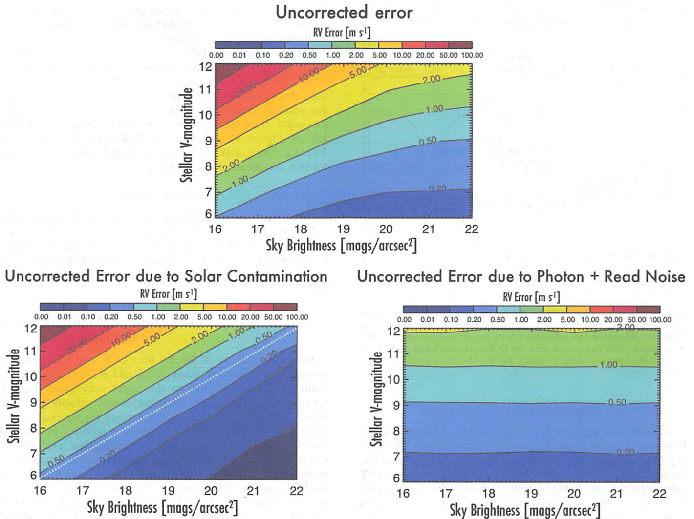
Figure 4. Uncorrected radial-velocity errors introduced by the presence of contaminating moonlight or scattered sunlight, for a range of stellar V-band magnitudes and sky brightness levels. Note that these are worst-case errors, calculated at the velocity separation between the star and the sky that causes maximum RV displacement. Top: simulations with realistic noise, including photon noise, read noise, and solar contamination, showing the full measured RV error. The full uncorrected error is separated into two categories in the bottom panels. Bottom left: isolating the error due to solar contamination. The dashed white line illustrates the error incurred following the traditional practice of observing when the sky is \sim 10 magnitudes fainter than the target. Bottom right: contribution of all other error sources, illustrating the achievable noise limit for each stellar brightness.
