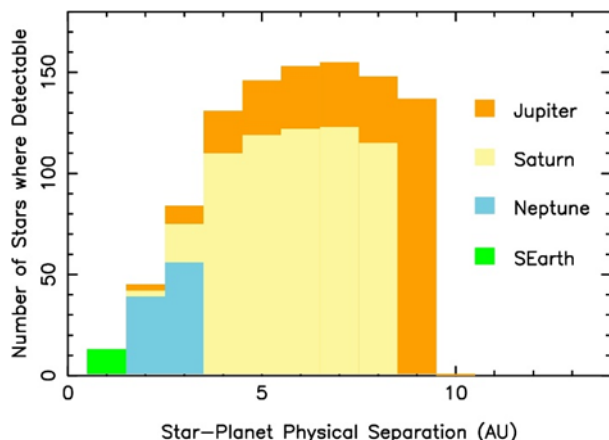
Figure 5. Exo-C exoplanetary search space in 48 hour broadband integrations for nearby stars, as a function of planet size and orbit.
