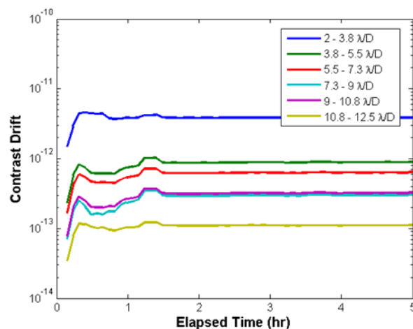
Figure 7 Modeled contrast evolution in six radial zones in the coronagraphic image plane after the telescope was rolled by 30^\circ about the line of sight. Even at the inner working angle of 2 \lambda/D , the contrast drift is below the 10^{-11} level, showing that the Exo-C design meets its stringent wavefront stability requirements.
