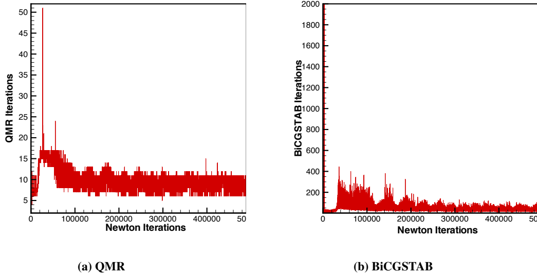
Fig. 3 Number of linear iterations against number of Newton iterations
