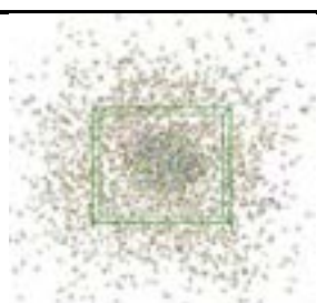
Figure 7a. Molecular Dynamics Simulations simulation with solvent outside the PBC
