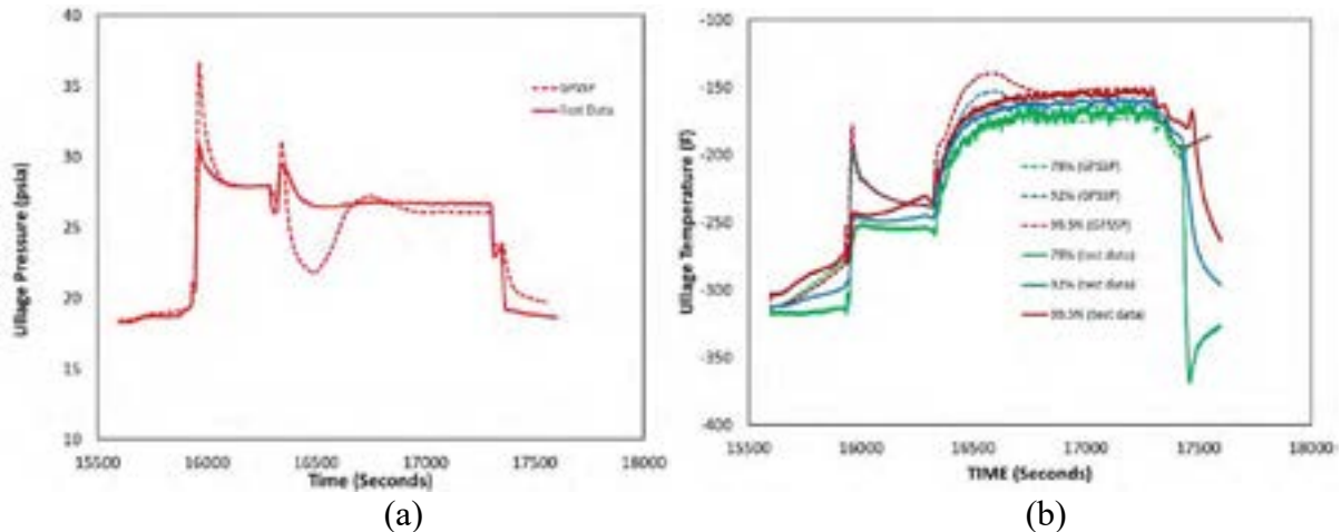
Figure 9. Comparison of computed data with test data for (a) ullage pressure and (b) ullage temperature.
