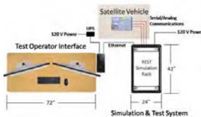
Figure 1: REST Lab Configuration (Hunt, 2019)
