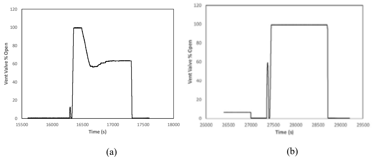
Figure 3. Vent Valve percentage Open with time.
