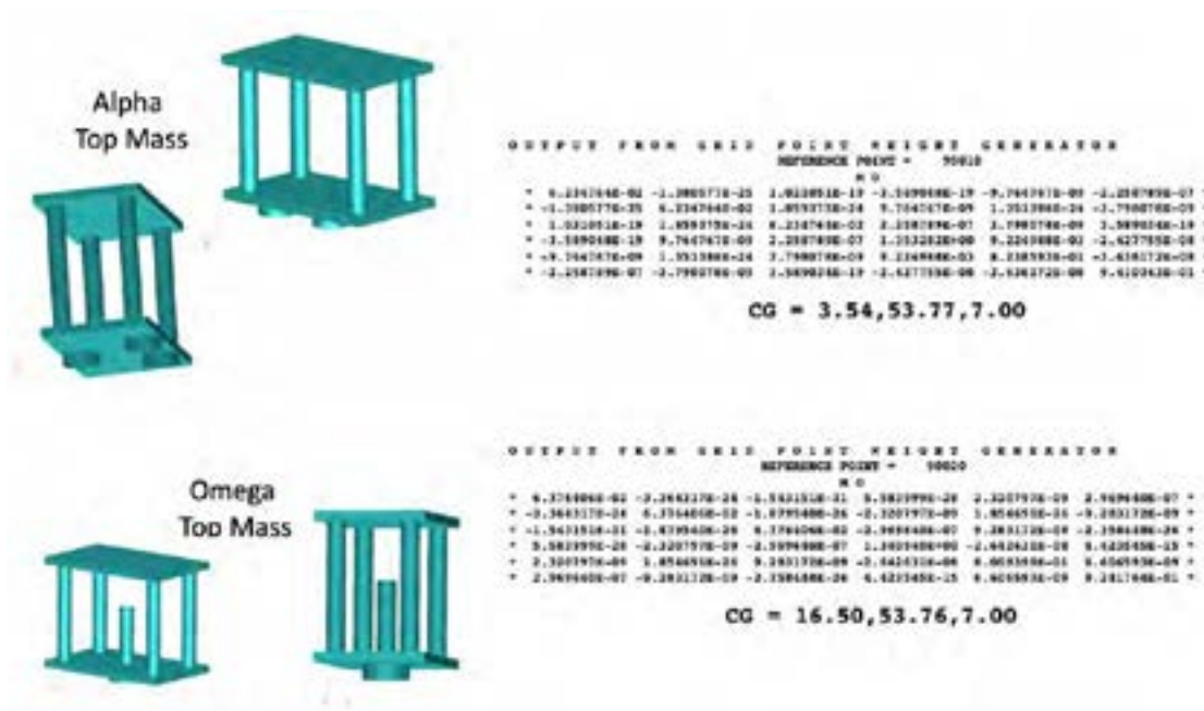
Figure 11. Top mass FEM representations and calculated mass properties.
