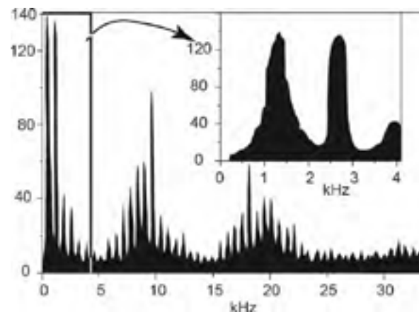
Figure 10. Signal-to-noise-variation ratio For a PZT-based AT23S sensor, up to the Nyquist frequency ( \sim 39 kHz) data in a laboratory experiment. Usable frequencies reach \sim 5 kHz.
