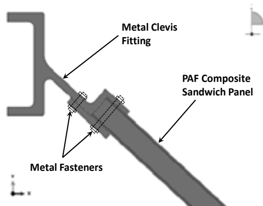
Figure 2. Metal clevis fitting.
