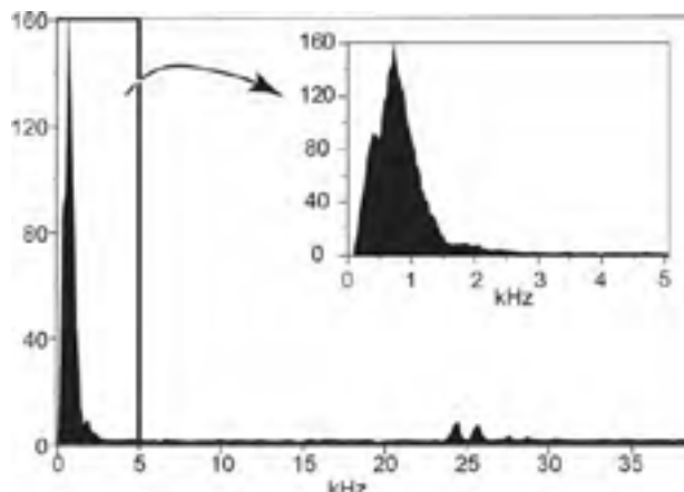
Figure 9. Signal-to-noise-variation ratio for a polymer-based ACH-01 sensor, up to the Nyquist frequency ( \sim 39 kHz), in a laboratory experiment. Usable frequencies reach \sim 5 kHz at most.
