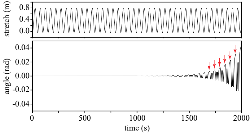
Fig. 6 (above) Stretch of a single tether as a function of time. (below) Relative angle of the corresponding pod with respect to the hub. Arrows mark times at which the stretch is negative (i.e., slack in the tether).
