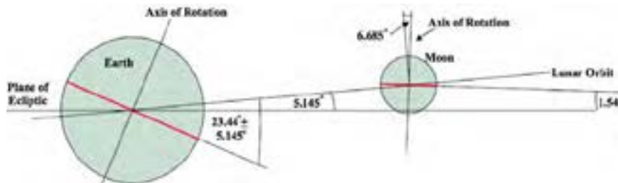
Figure 1. Orientation of the Lunar Orbit Relative to Earth's Equator and the Ecliptic Plane.
