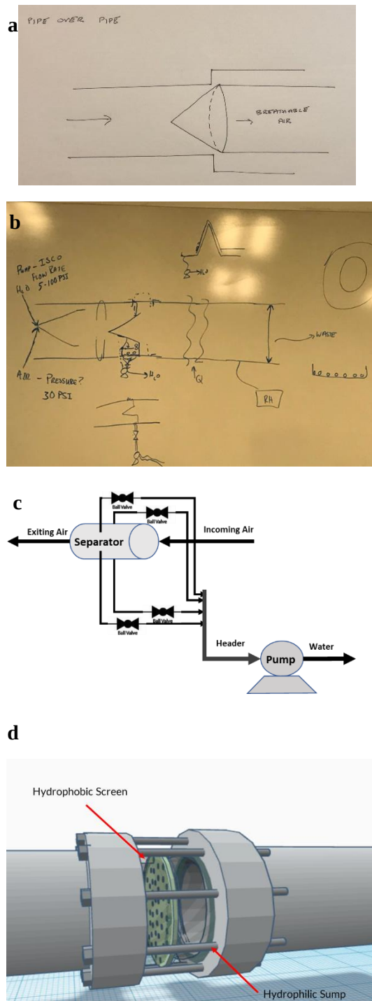
Figure 3. (a) Initial student design based on Figure 2 (b) refined student design (c) system sump design (d) detailed sump design based on a rupture disk.
