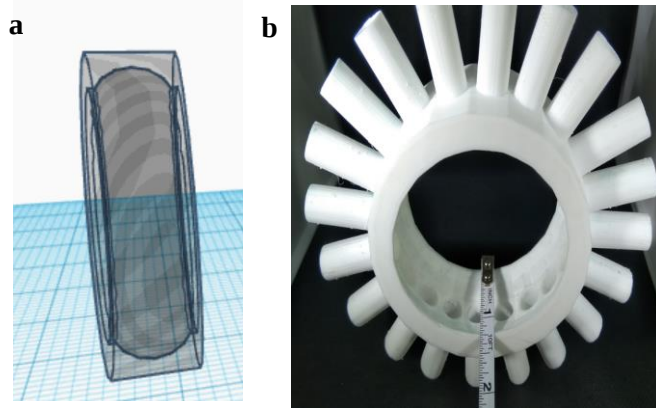
Figure 4. (a) Initial ring like rupture disk in CAD (b) resulting 3D printed part after adding pipes to basic rupture disk
