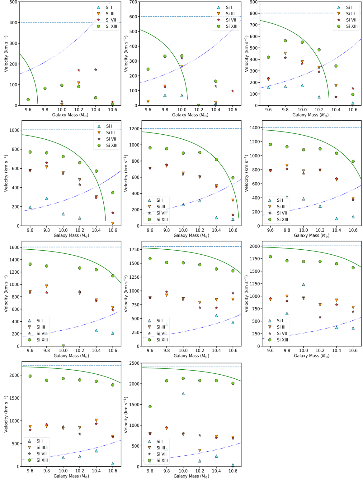
Figure 6. As for Figure 1 I plot outflow velocity vs. galaxy mass. Outflow velocities are measured by Si I (upward triangles), Si III (downward triangles), Si VII (stars), and Si XIII (circles). In each panel the blue dashed line indicates the CC85 model velocity ranging from 400 km s -1 (top left) to 2400 km s -1 (bottom center). The solid green curve is the CC85 model velocity modified to include the gravitational potential, and the dotted purple curve is the escape velocity for gas in the galactic nucleus.
