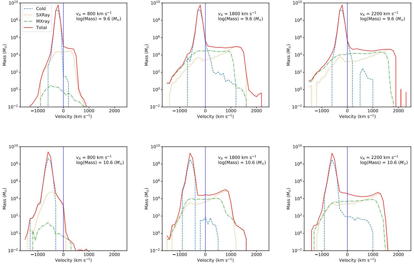
Figure 2. Example mass distributions binned according to v_{out} for two galaxy masses (top row 10^{9.6} M_{\odot} , bottom 10^{10.6} M_{\odot} ) and CC85 model velocities 800 \text{ km s}^{-1} , 1800 \text{ km s}^{-1} , and 2200 \text{ km s}^{-1} left to right. v = 0 \text{ km s}^{-1} = v_{escape} is the vertical blue line; gas to its left is bound by gravity, to right escapes. The solid red curves trace the total mass per velocity bin. The dotted orange curve and the dot-dashed green curve show mass with temperatures in the Soft X-ray and Mid X-ray regimes respectively. The blue dashed curve shows cold mass at < 100 \text{ K} .
