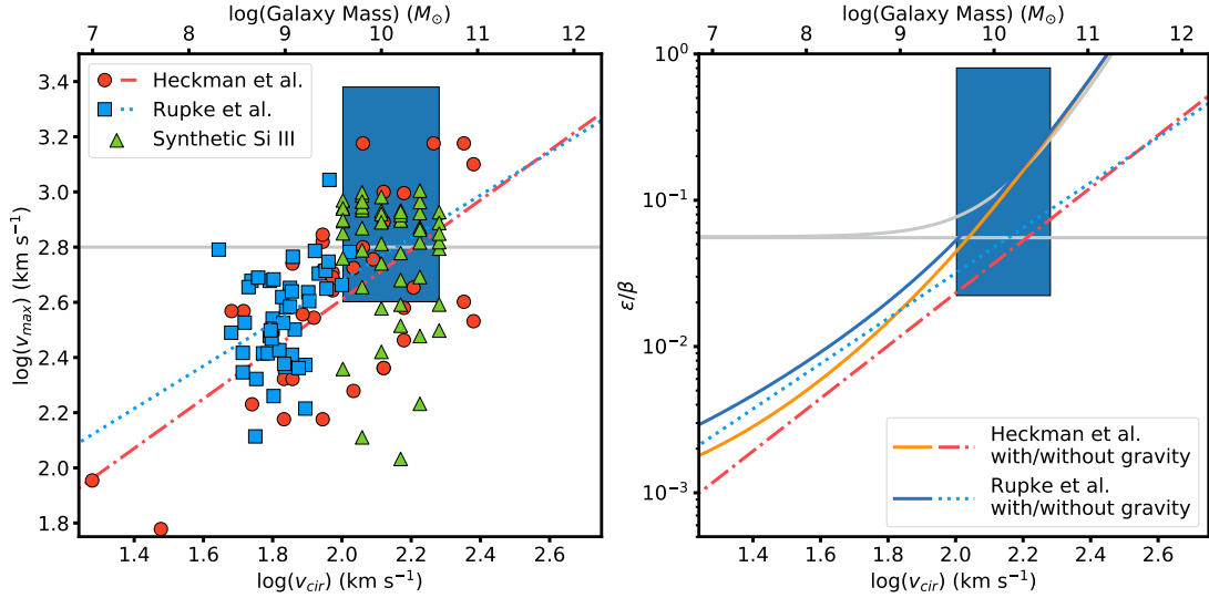
Figure 5. The left panel plots maximum outflow velocity vs. circular velocity. Red circles are data from Heckman & Borthakur (2016). Blue squares are data from Rupke et al. (2005). Lines show fits for both datasets. Green triangles show velocities from my simulations of the Si III lines. In both panels the blue rectangle shows the parameter space of my simulations. I have included a fit (grey line) at a constant v_{\max} for all v_{\text{cir}} . In the CC85 model this corresponds to constant \epsilon/\beta . At right I convert the best fits of Heckman et al. and Rupke et al. into \epsilon/\beta values using the JA71 and CC85 models (with and without gravity, respectively). The two grey lines show \epsilon/\beta for the constant v_{\max} as computed using the JA71 and CC85 models.
