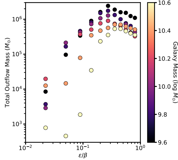
Figure 4. The same total masses from Figure 3 plotted with respect to \epsilon/\beta of each simulation using Equation 7. The outflow velocity for the simulations increases from left to right. Circle coloring indicates the galactic mass for each simulation.
