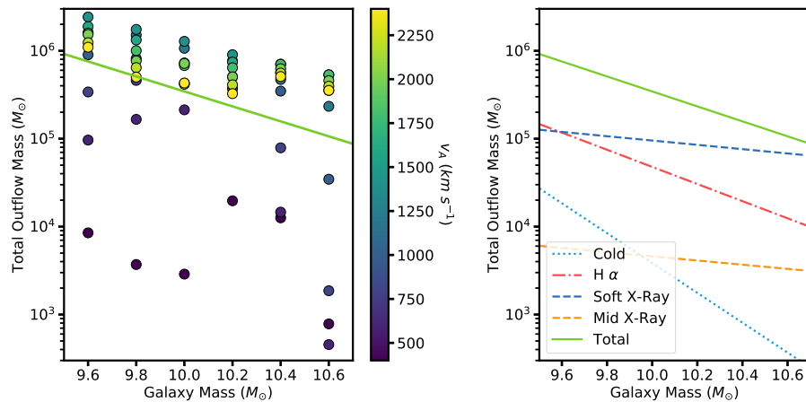
Figure 3. Left plots the total mass above the escape velocity (everything to the right of the vertical lines in Figure 2) with respect to galactic mass. All 66 simulations are plotted, and each dot is colored according to the CC85 model velocity. In solid green is the linear fit to the data with slope -0.85. At right I show the total mass in various gas temperature regimes from my simulations and their linear fits (fitted slopes given in Table 1).
