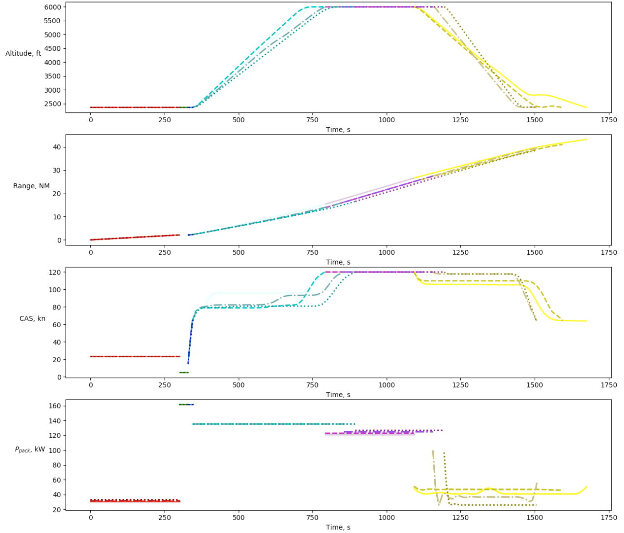
Fig. 3 Optimal Flight Profiles for Varying Battery Pack Sizes. (See Fig 2 Legend)
