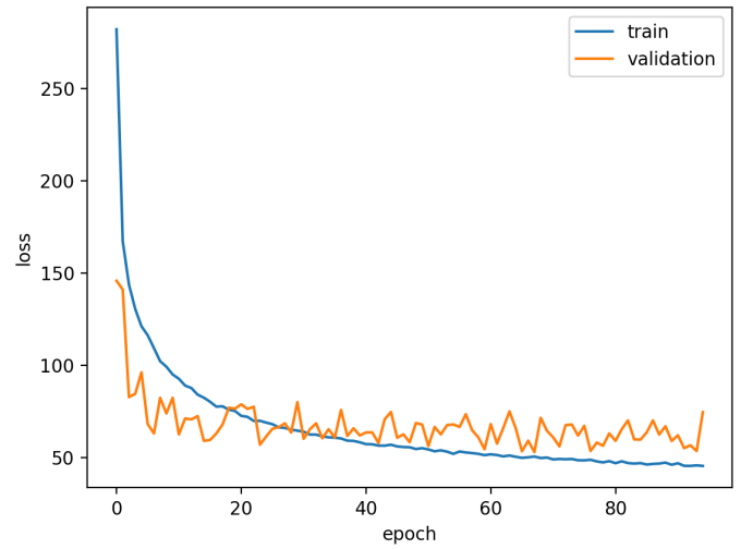
Fig. 4: Training accuracy: model loss mean squared error
