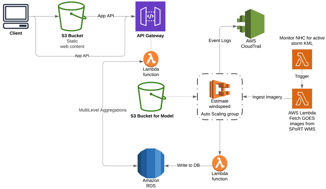
Fig. 10: Architecture of the production system
