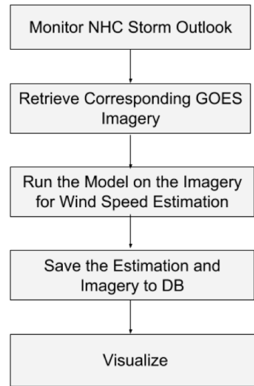
Fig. 9: Event-based workflow for production system
