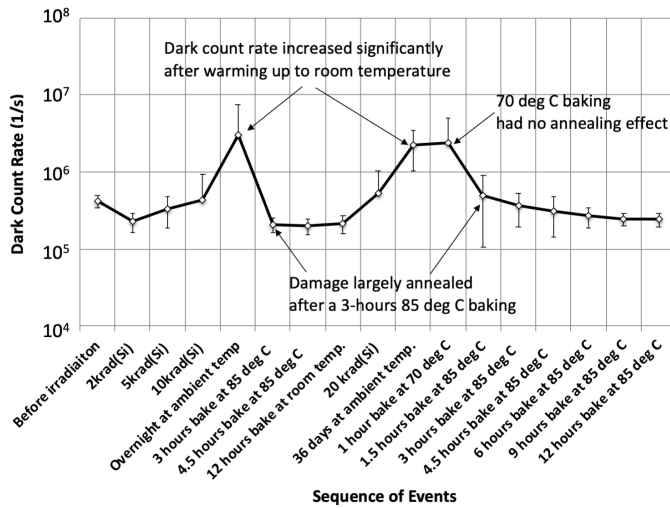
Fig. 10. The 2x8 pixel HgCdTe APD median dark count rates at a threshold setting of 100 mV through the sequence of events of proton irradiation and annealing. The data are from the Hg-vacancy doped device [33].
