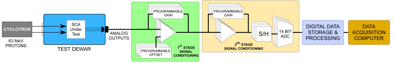
Fig. 2. Block diagram of the test setup of the proton irradiation of the HgCdTe APD arrays and performance monitoring by AFRL at CNL.
