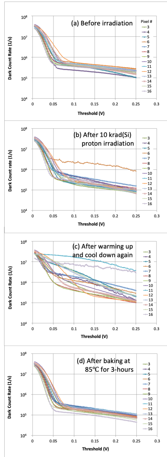
Fig. 9. HgCdTe APD dark count rates vs. threshold from the Cu-Hg doped device, (a) before proton irradiation, (b) after 10 krad(Si) proton irradiation, (c) after warming up to room temperature overnight, and (d) after a 3-hour 85 °C bake. The data were from the Hg-vacancy doped device. The Cu-Hg doped device showed similar behavior. The
