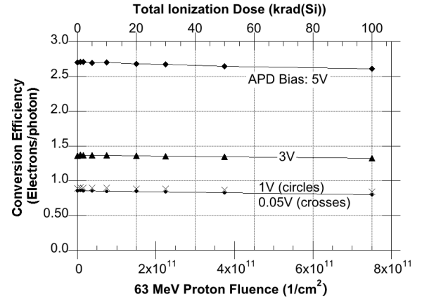
Fig. 4. APD photon to electron conversion efficiency (quantum efficiency times the gain) vs. proton fluence of the HgCdTe APD, Pixel (3,4), at several APD biases.
