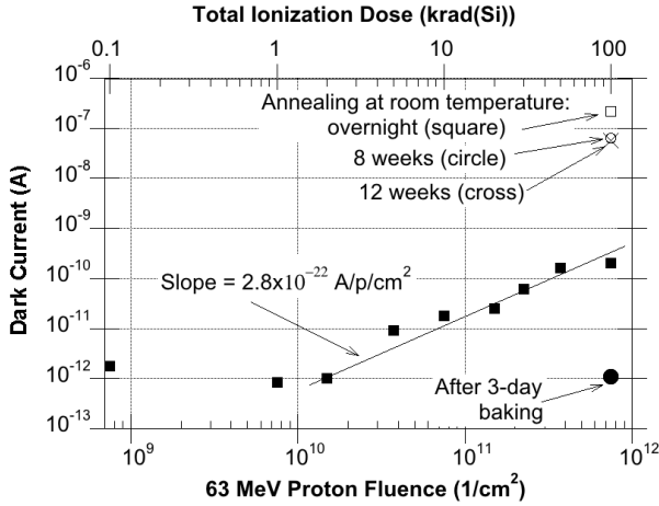
Fig. 3. Dark current vs. proton fluence of the HgCdTe APD, Pixel (3,4) at 12 V APD bias.
