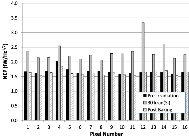
Fig. 6. NEPs of the HgCdTe APD before and after a 30 krad(Si) proton irradiation. The NEPs returned to the pre-irradiation levels after a 72-hour 90 °C bake out.
