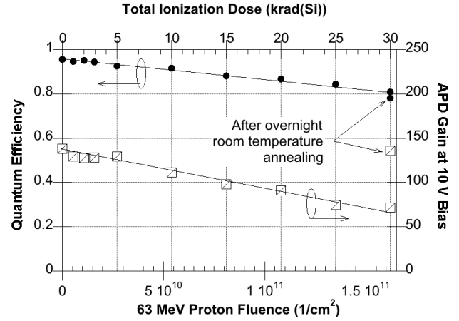
Fig. 5. APD median quantum efficiency and gain vs. proton dose up to 30 krad(Si) at 10 V APD bias (APD gain ~120). Note the near complete recovery of the APD gain after annealing at room temperature overnight.
