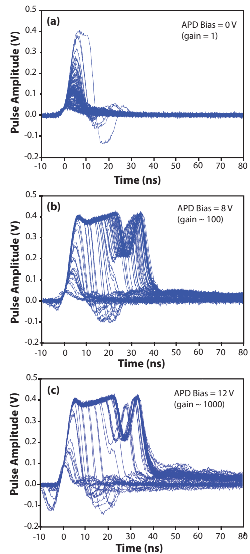
Fig. 7. Sample HgCdTe APD output pulse waveforms in response to proton hits with the APD biased at 0, 8, and 12 V [33].
