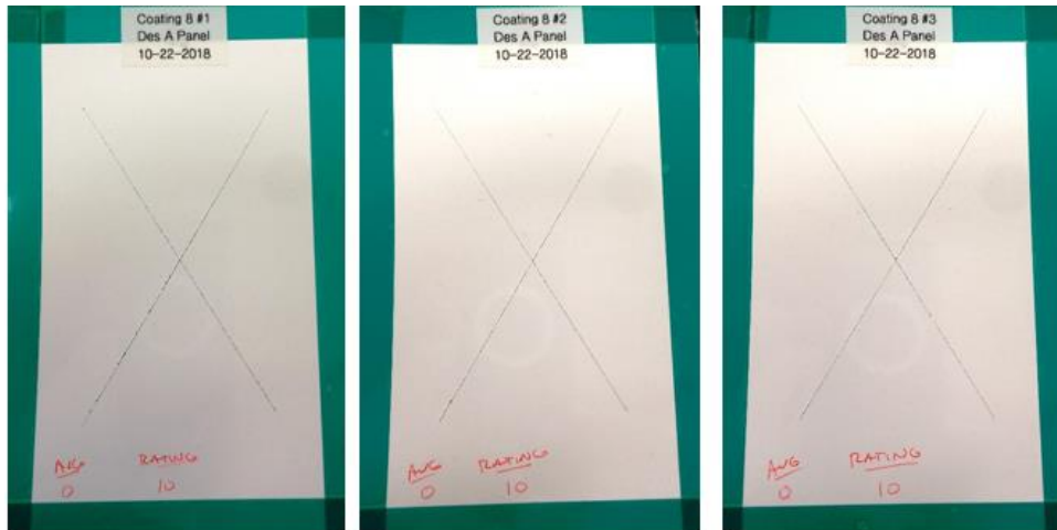
Figure 27. Coating 8 on AA2024-T3 test panels with Alodine pretreatment and CA 8201 polyurethane topcoat after 2000 hours of salt fog exposure showing ASTM D1654 average rating of 10.
