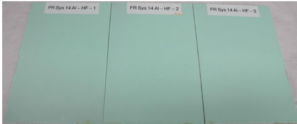
Figure 47. Coating 14 on Alodine pretreated AA2024-T3 panels after MIL-PRF-23377 hydraulic fluid resistance testing.
