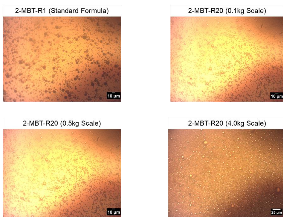
Figure 15. Optical microscopy images of 2-MBT micro particles obtained with reaction conditions labeled as 2-MBT-R1, 2-MBT-R20 (0.1 kg scale), 2-MBT-R20 (0.5 scale), and 2-MBT-R20 (4.0 kg scale) on Table 20.
