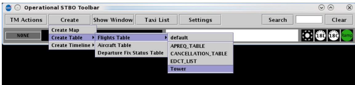
Figure 5.22. Create a Flights Table using a saved configuration (in this example, “Tower”).
