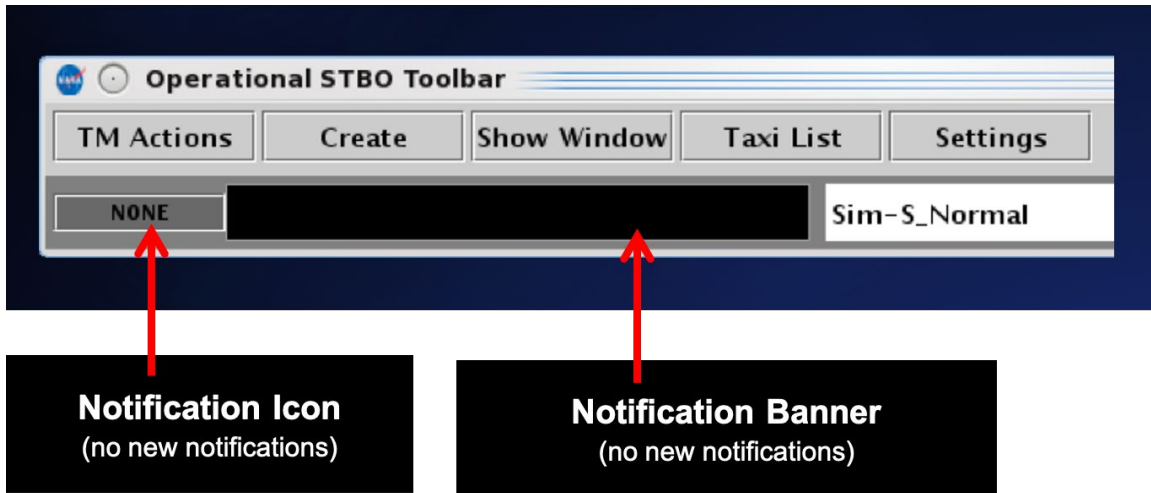
Figure 3.96. Notification Icon and Notification Banner after notifications are acknowledged.
