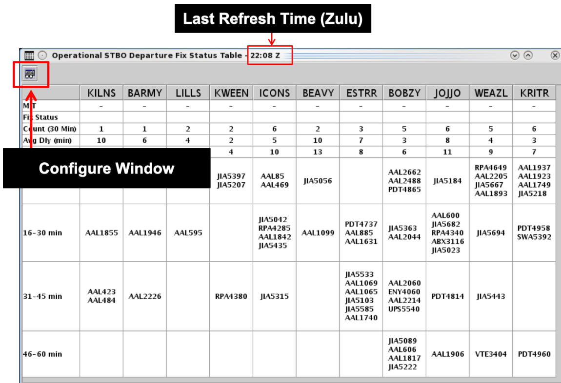
Figure 5.26. Departure Fix Status Table.
