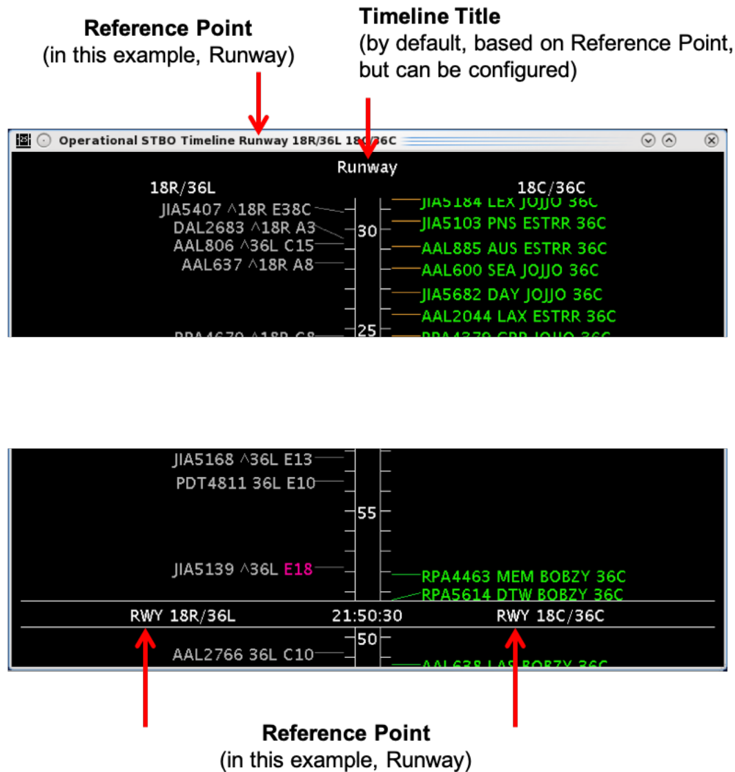
Figure 6.22. Timeline: In this example, “Runway” is the selected Reference Point.
