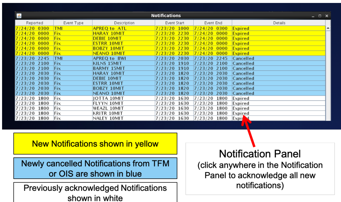
Figure 3.94. Notification Panel: New notifications (yellow), new cancellation notifications (blue), and previously acknowledged notifications (white).
