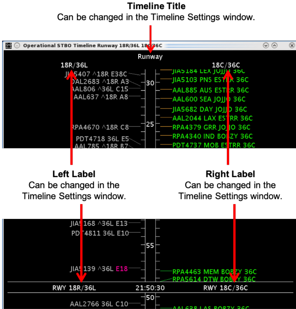
Figure 6.24. Timeline Settings window: Title and Left/Right Label fields.
