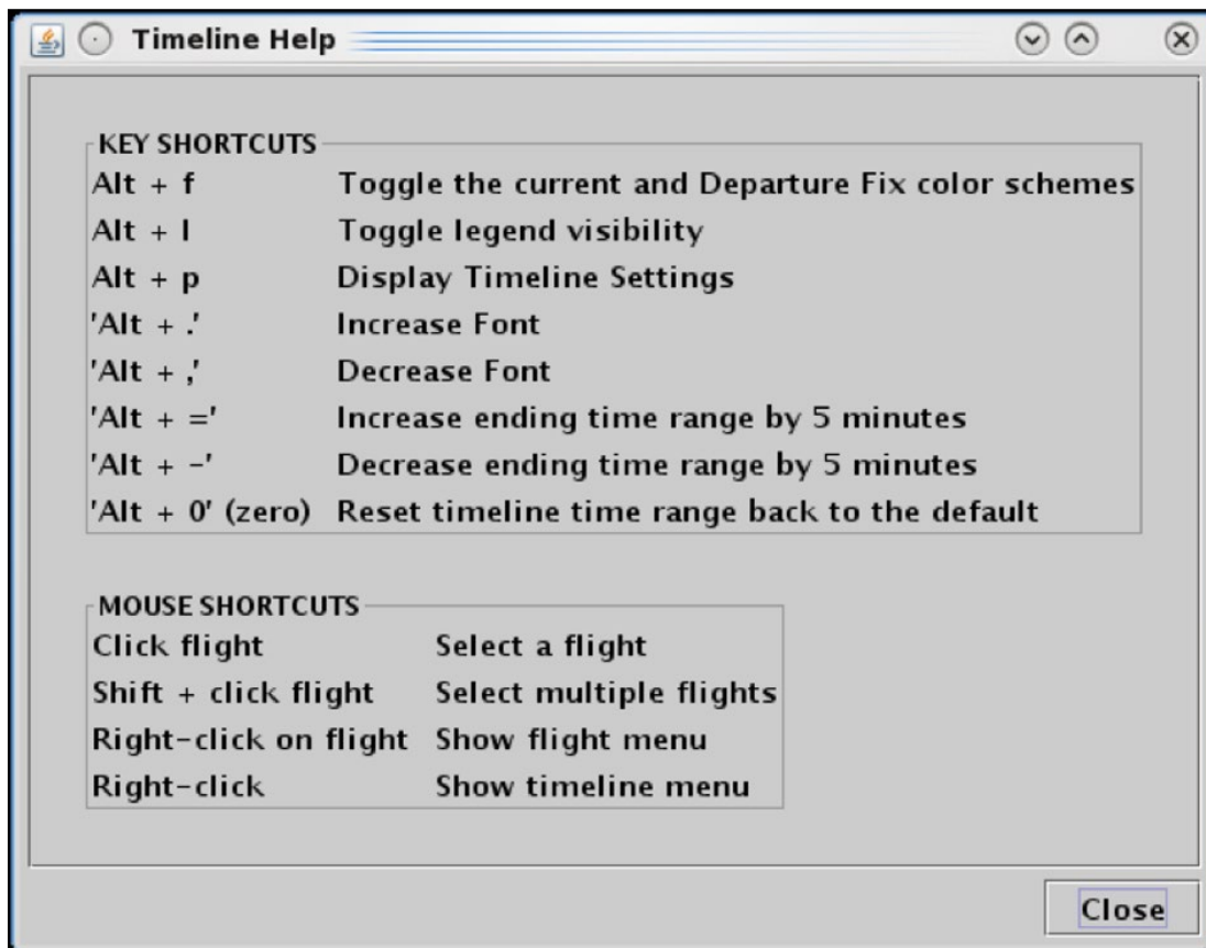
Figure 4.40. Timeline Help.
