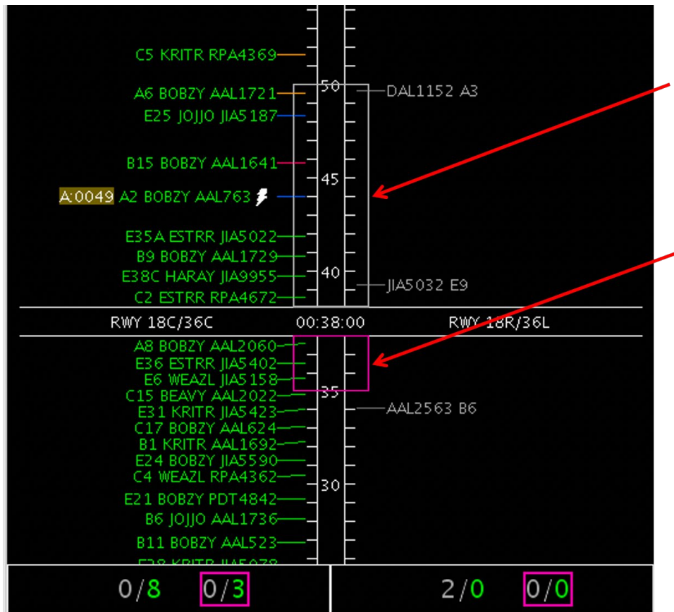
Figure 6.14. Flight Plan Demand with a Fixed Time Period (0035 to 0050 UTC, in this example). Above “Now” time, the window is outlined in white; below “Now” time, the window is outlined in magenta.
