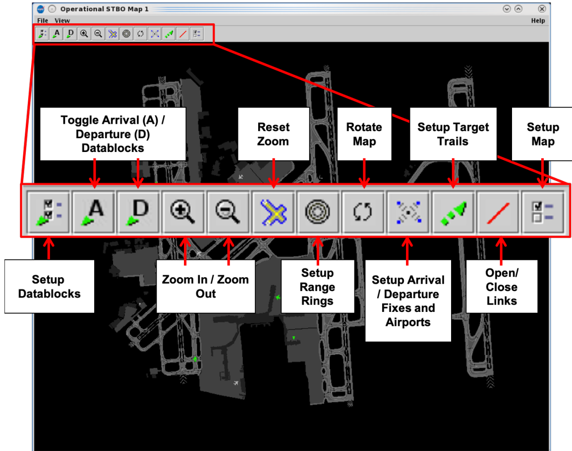
Figure 4.41. Map: Toolbar.
