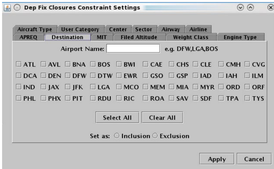
Figure 3.53. Constraint: Destination.
