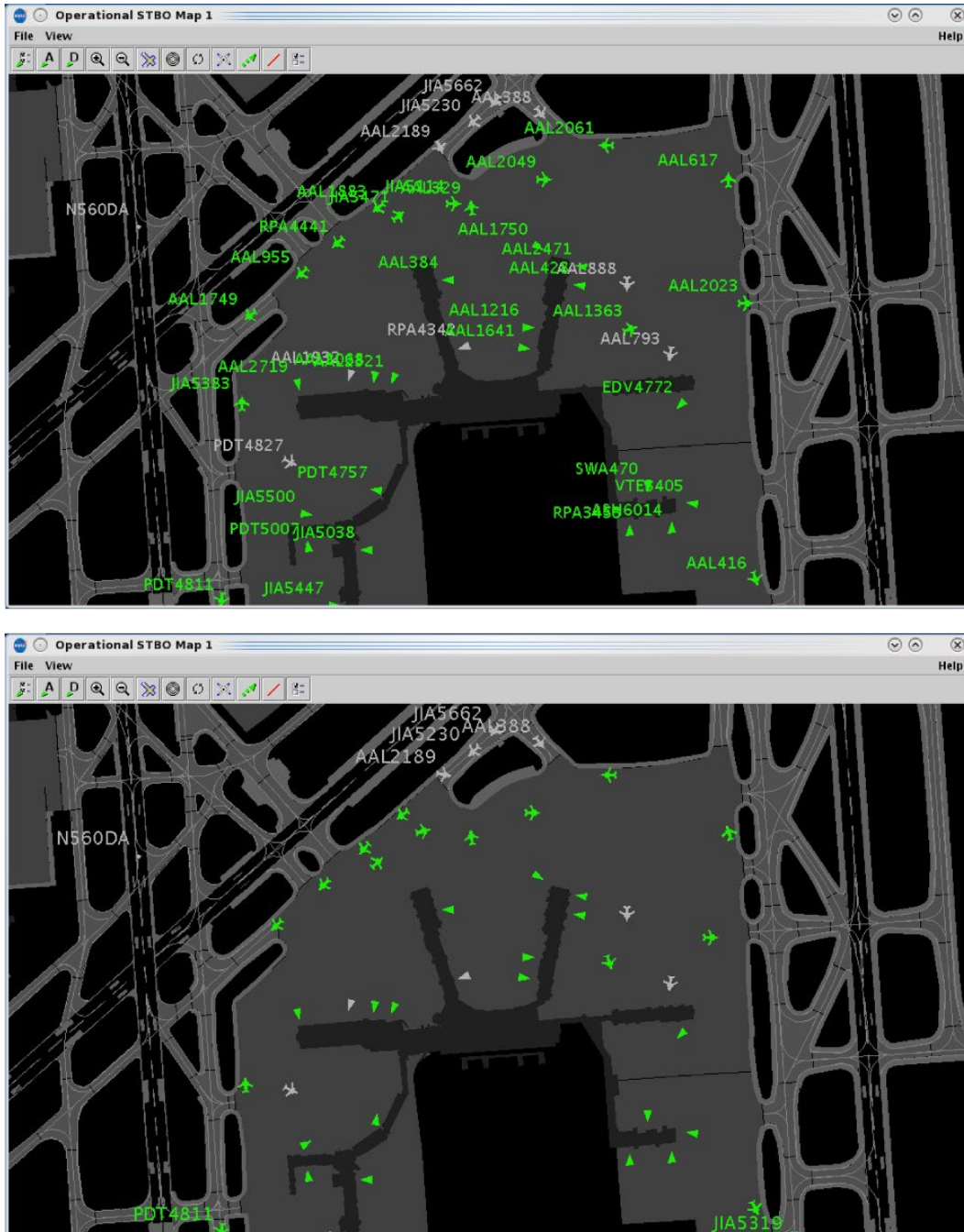
Figure 4.26. Airport Settings: Deselect “AMA Only Datablocks” to display datablocks in the Ramp Area (top) or select this option to hide datablocks while in the Ramp Area (bottom).
