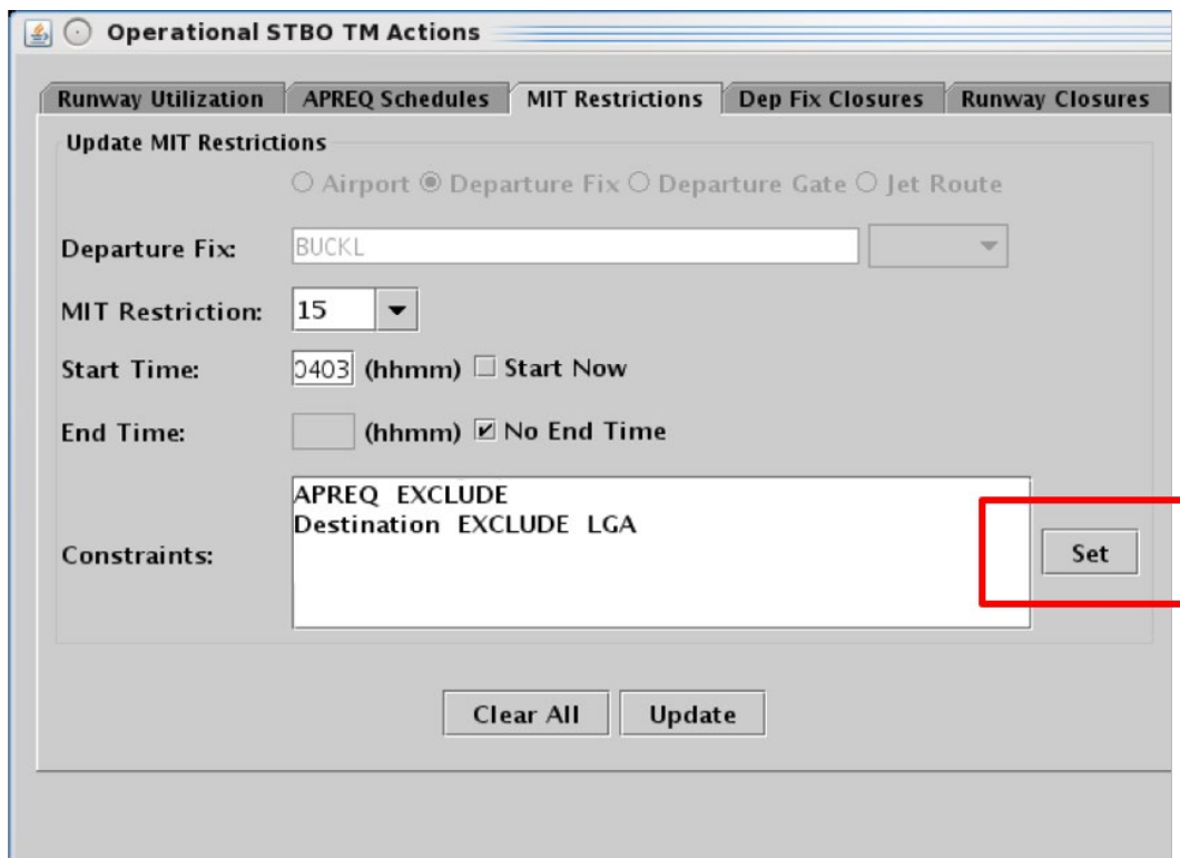
Figure 3.37. Select the “Set” button to open the Constraint Settings window.
