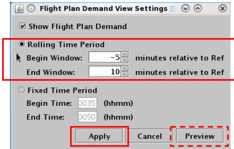
Figure 6.11. Flight Plan Demand View Settings: Rolling Time Period.
