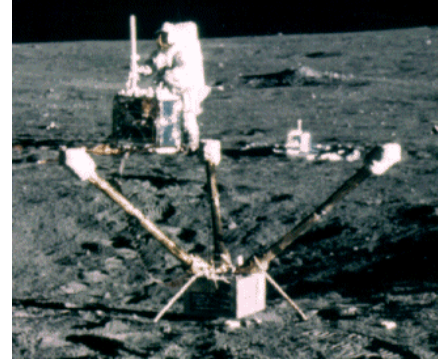
Fig. 1. Apollo 12 astronaut Pete Conrad works at the ALSEP central station. The Lunar Surface Magnetometer (LSM) is in the foreground. AS12-47-6921.
