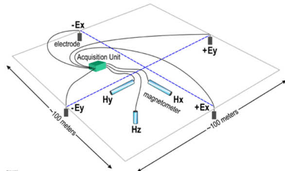
Fig. 2. Schematic magnetotelluric (MT) experiment. Magnetometer(s) are centralized (like LSM), but electric field is measured using orthogonal voltage probes (electrodes) on large baselines. CLPS Lunar Magnetotelluric Sounder (LMS) ballistically deploys electrodes to ~20 m, but astronaut deployment to 100 m would be robust and yield larger signals.
