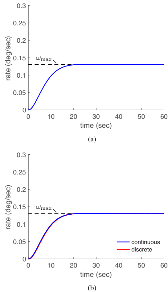
Figure 10. Continuous-time slew rate response from simulation of the attitude control system using: (a) proposed interpolation filter and (b) sample-and-hold at the ACS rate (Figure 4b repeated).
