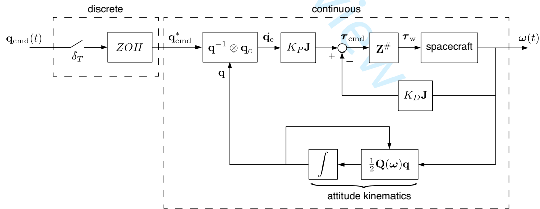
Figure 2. Block diagram of discrete-continuous time attitude control system.
