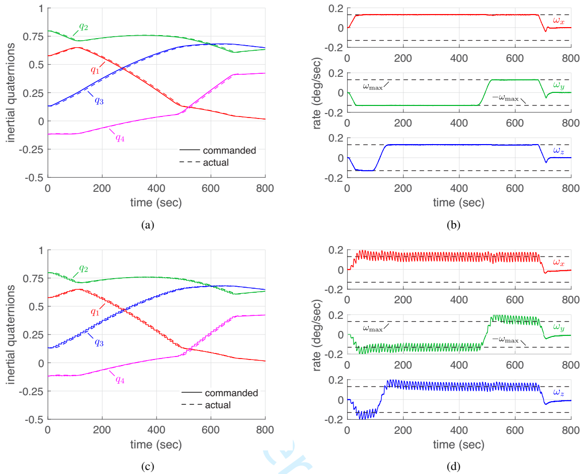
Figure 1. Simulation of a fast attitude maneuver designed for the Lunar Reconnaissance Orbiter: (a) attitude quaternions for waypoint sampling at the ACS frequency (5 Hz); (b) body rates for waypoint sampling at the ACS frequency (5 Hz); (c) attitude quaternions for downsampled waypoints (0.1 Hz); (d) body rates for downsampled waypoints (0.1 Hz).
