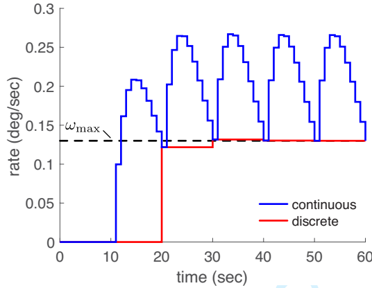
Figure 6. Reconstruction of continuous-time slew rate response using time-shifted samples for downsample-and-hold at T = 10\text{sec} .
