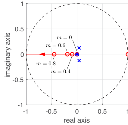
Figure 7. Pole-zero pattern of \omega(z, m)/\Phi_{\text{cmd}}(z) showing locus of additional zero for various values of m for downsample-and-hold at T = 10\text{ sec} .
