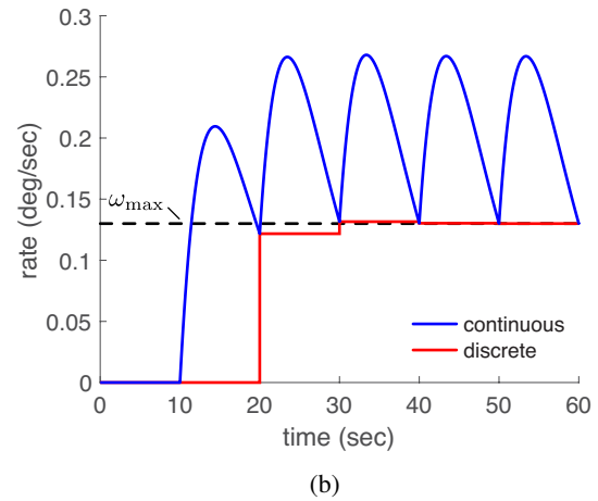
Figure 4. Slew rate response from simulation of the discrete time attitude control system (13): (a) sample-and-hold at T = 0.2 sec and (b) downsample-and-hold at T = 10 sec.
