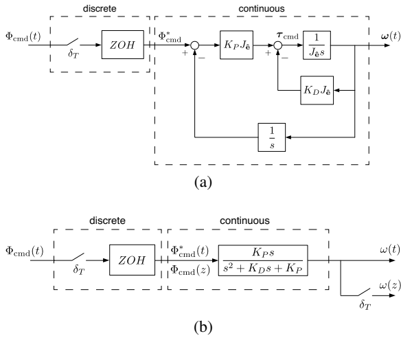
Figure 3. Block diagram of discrete-continuous time attitude control system: (a) as a second-order system; (b) reduced for z -transformation.
