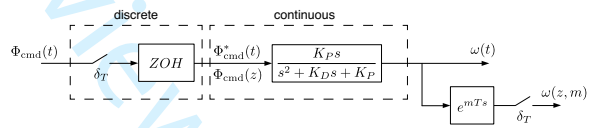
Figure 5. Block diagram of time-shifted discrete-continuous time attitude control system.
