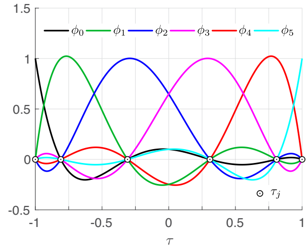
Figure 9. Sixth-order Lagrange polynomials.
