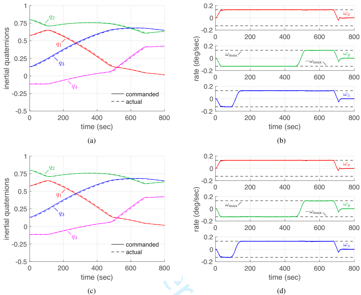
Figure 11. Simulation of a fast attitude maneuver designed for the Lunar Reconnaissance Orbiter: (a) attitude quaternions for waypoint sample-and-hold at the ACS rate; (b) body rates for waypoint sample-and-hold at the ACS rate; (c) attitude quaternions using interpolation filter; (d) body rates using interpolation filter.
