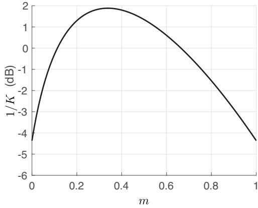
Figure 8. Gain factor of \omega(z, m)/\Phi_{\text{cmd}}(z) for various values of m for downsample-and-hold at T = 10 sec.
