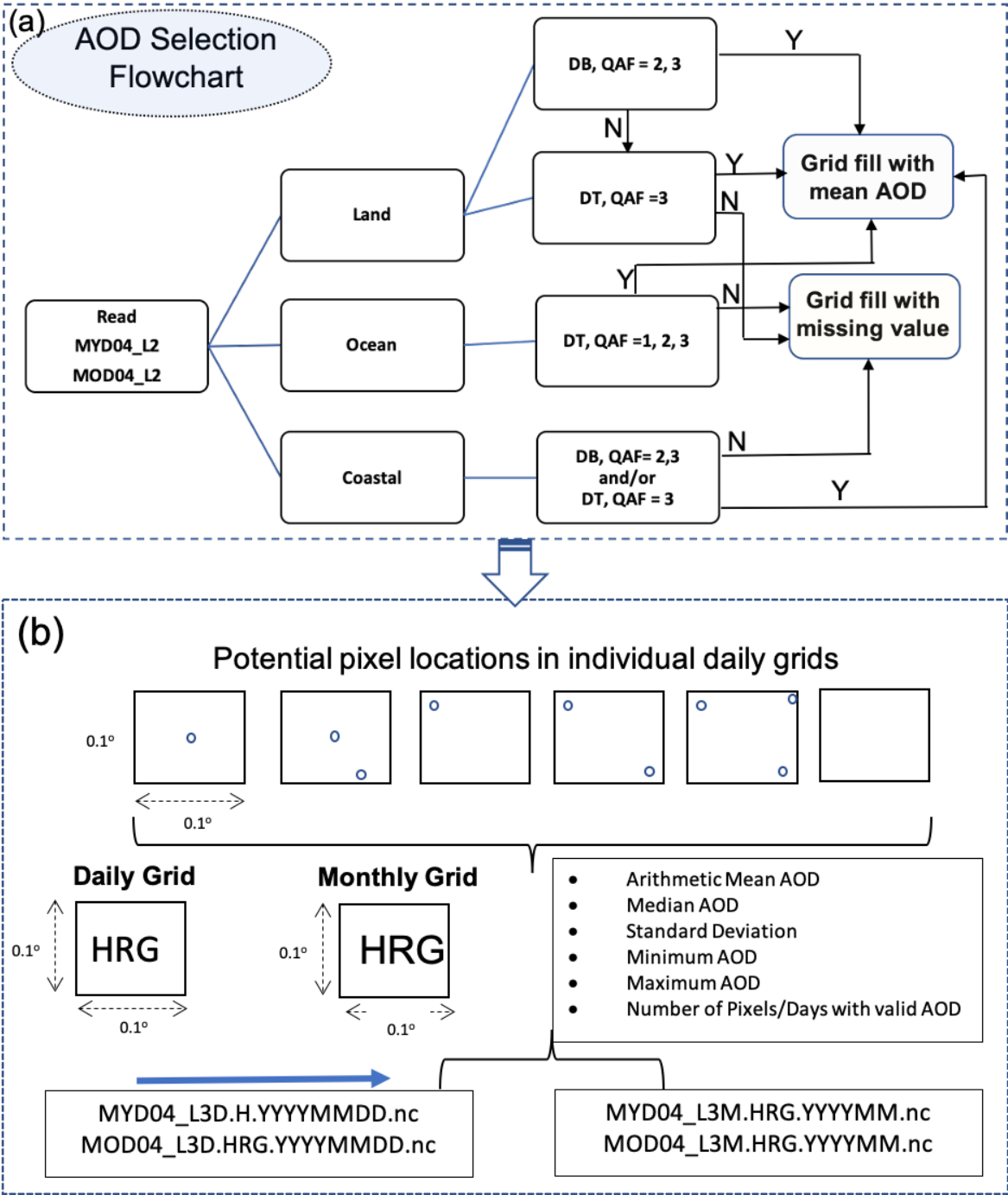
Figure 1. Flowchart showing data processing sequence, pixel, and grid orientations and list of output variables and filenames for daily and monthly data.
