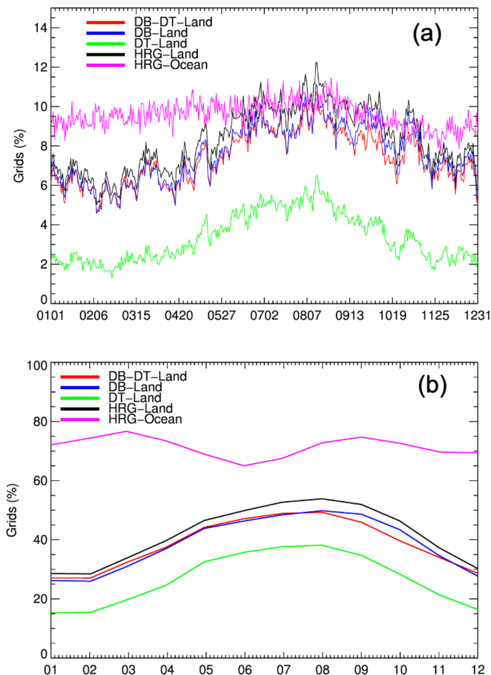
Figure 4. Daily (a) and monthly (b) distribution of the number of grids in percentage with valid AODs data from MODIS-Aqua for the year 2010. Grid percentage represents available valid AODs grids out of total land (or ocean) grids for the global regions at 0.1x0.1-degree resolution.
