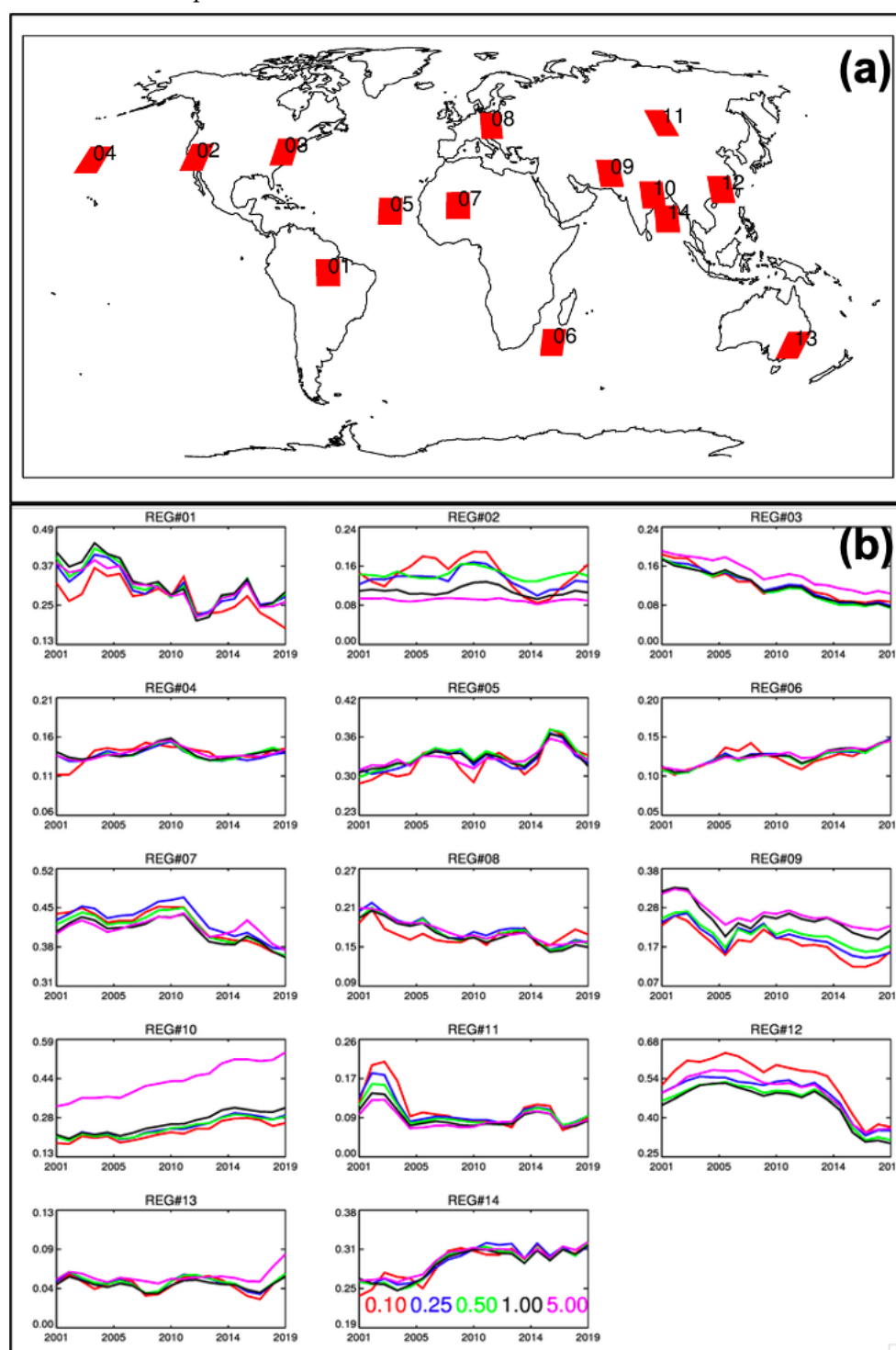
Figure 11. Timeseries of annual mean aerosol optical depth from MODIS-Terra for 14 selected regions around the globe. The top panel (a) shows the location of regions of the 5x5 degree box. The bottom panels (b) show the timeseries for each region, as shown on the map. The different colors on the
