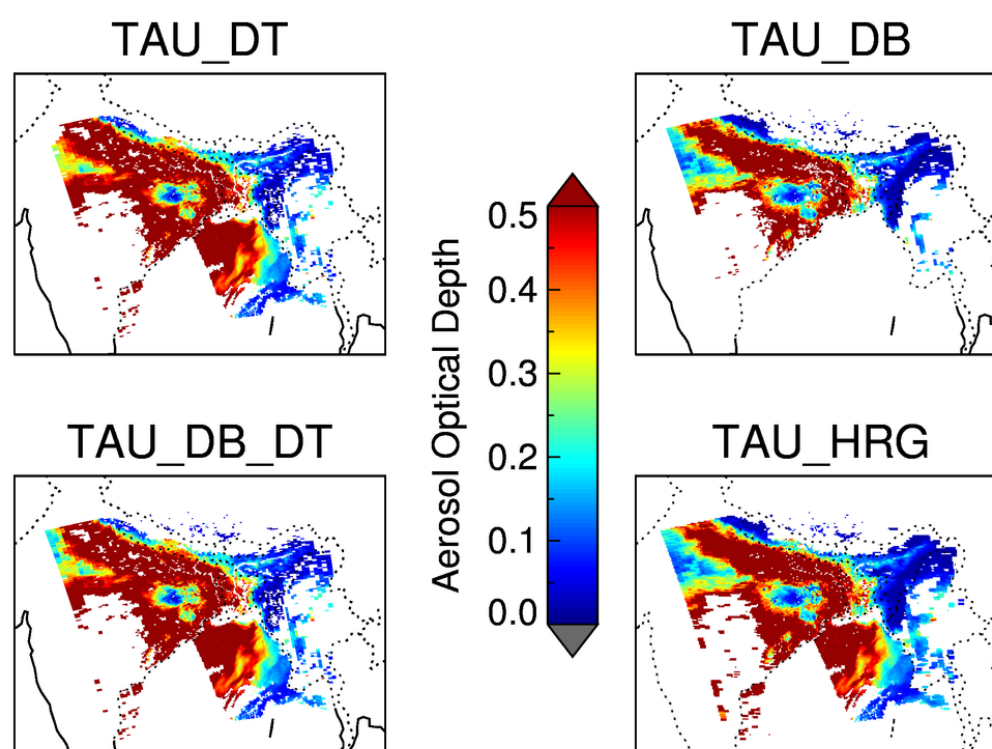
Figure 3. Aerosol optical depth (550 nm) from MODIS-Aqua over Asia on December 9, 2018, at 07:30 UTC. The AOD data are mapped to show: TAU_DT: AOD retrieved using DT algorithm; TAU_DB: AOD retrieved using DB algorithm; TAU_DB_DT: operational DT-DB combined parameter; and TAU_HRG: high resolution gridded data combining TAU_DT and TAU_DB with spatial filling while taking pixel size in the account.
