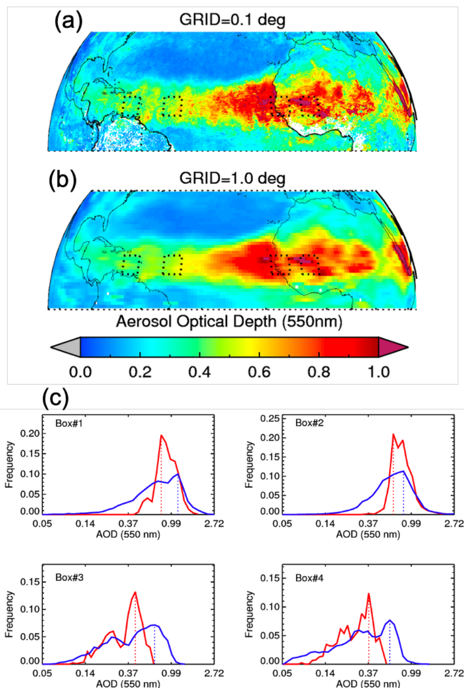
Figure 10. Application of HRG AOD to monitor dust transport across the Atlantic Ocean during June 2018. a) map shows mean HRG AOD from both MODIS-Aqua and MODIS-Terra from June 18 to July 3, 2018, b) same as (a) but at the reduced spatial resolution of 1×1 degree (CRG), and c) The four histograms represented four 10×10 degree boxes on the path of dust plume as it originates over North Africa and transport over the Atlantic Ocean and finally reached to American continents. The Red line on the histogram is using CRG, whereas blue is from HRG AOD data.
