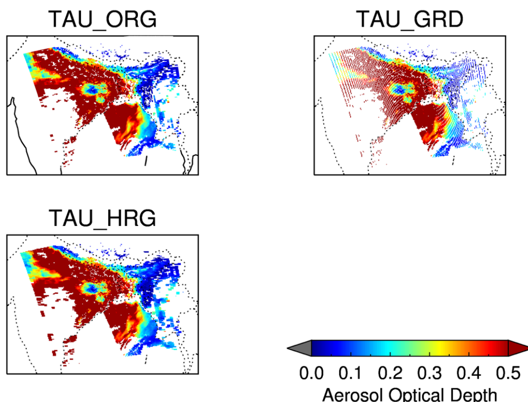
Figure 2. Aerosol optical depth (550 nm) from MODIS-Aqua over Asia on December 9, 2018, at 07:30 UTC. The AOD data are mapped to show: TAU_ORG: original data considering varying pixel size; TAU_GRD: high resolution gridded data with no filling of empty grids; and TAU_HRG: high resolution gridded data with spatial filling at the edge of the swath.
