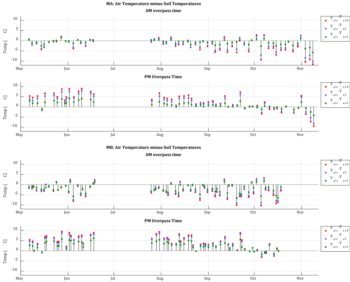
Figure S2. Temperature gradients at the experiment sites measured by the different sensors of the temporary networks during the SMAP overpasses. The bars show the differences between the air temperature measured at 1.5 m aboveground ( T_{air} ) and the temperature measured by the different soil moisture sensors. The top two plots show the differences for the MA sites during AM and PM overpasses and the bottom two plots show the difference for the MB sites during the AM and PM overpasses. T_{s10} refers to the temperature measured by the soil moisture sensor at 10 cm depth, T_{s5} refers to the temperature measured by the soil moisture sensor at 5 cm depth, and T_{sv5} refers to the temperature measured by the vertically installed soil moisture sensor. The difference is always largest for T_{s10} , second largest for T_{s5} and smallest for T_{sv5} .
