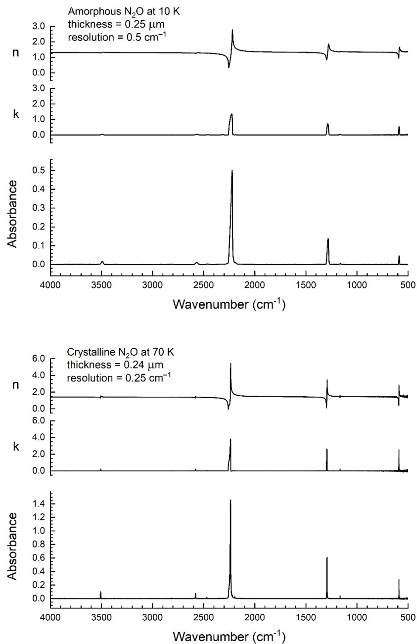
Figure 7. Top panel: Measured IR absorbance, and calculated values of n and k for amorphous \text{N}_2\text{O} at 10 K. Absorbance shown is for a sample thickness of 0.25\ \mu\text{m} , measured with a resolution of 0.5\ \text{cm}^{-1} from 4000 to 500\ \text{cm}^{-1} . Bottom panel: Crystalline \text{N}_2\text{O} at 70 K, with a thickness of 0.24\ \mu\text{m} , measured with a resolution of 0.25\ \text{cm}^{-1} from 4000 to 500\ \text{cm}^{-1} .
