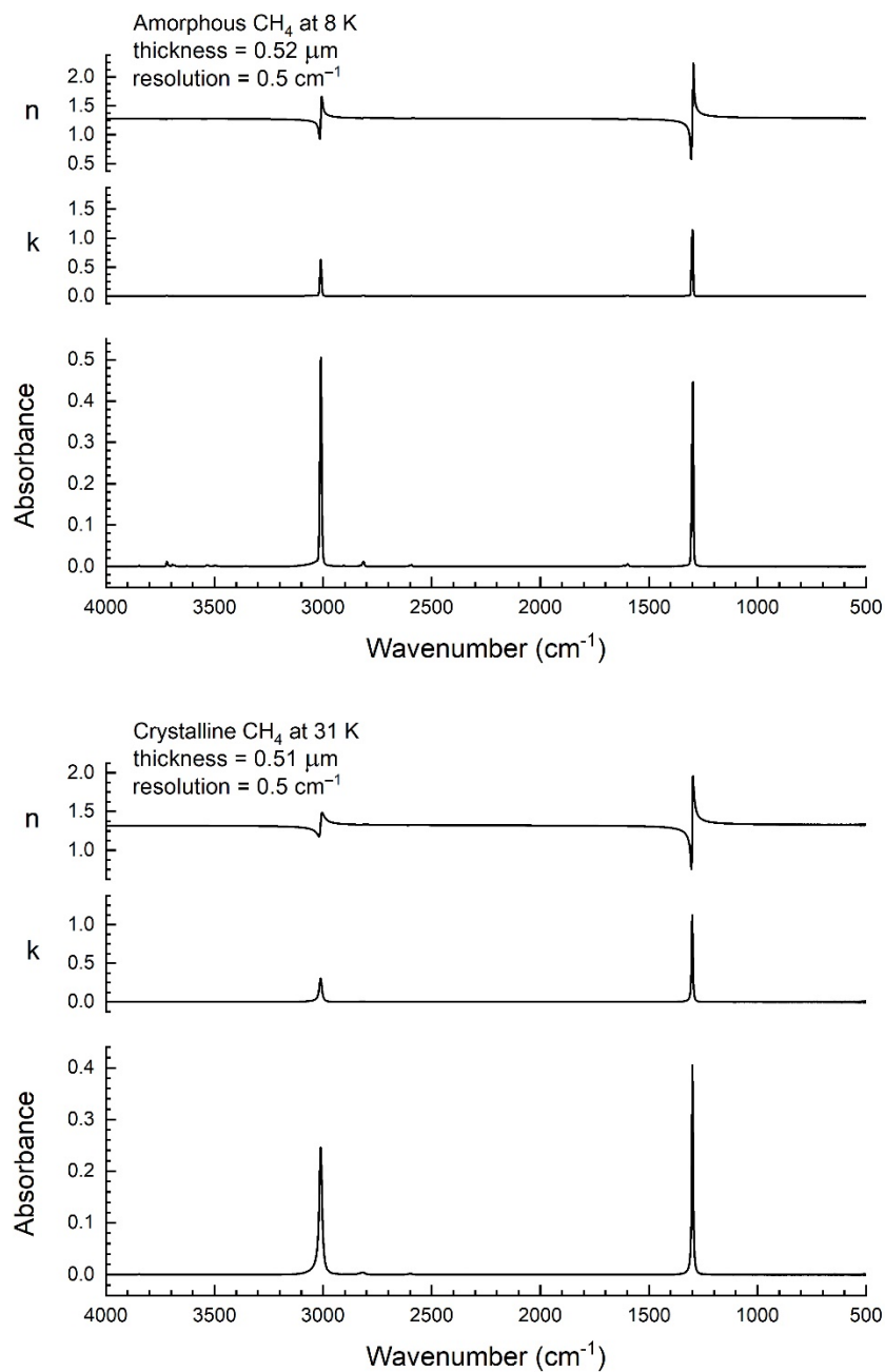
Figure 8. Top panel: Measured IR absorbance, and calculated values of n and k for amorphous \text{CH}_4 at 8 K. Absorbance shown is for a sample thickness of 0.52 \mu\text{m} , measured with a resolution of 0.5 \text{ cm}^{-1} from 4000 to 500 \text{ cm}^{-1} . Bottom panel: Crystalline \text{CH}_4 at 31 K, with a thickness of 0.51 \mu\text{m} , measured with a resolution of 0.5 \text{ cm}^{-1} from 4000 to 500 \text{ cm}^{-1}
