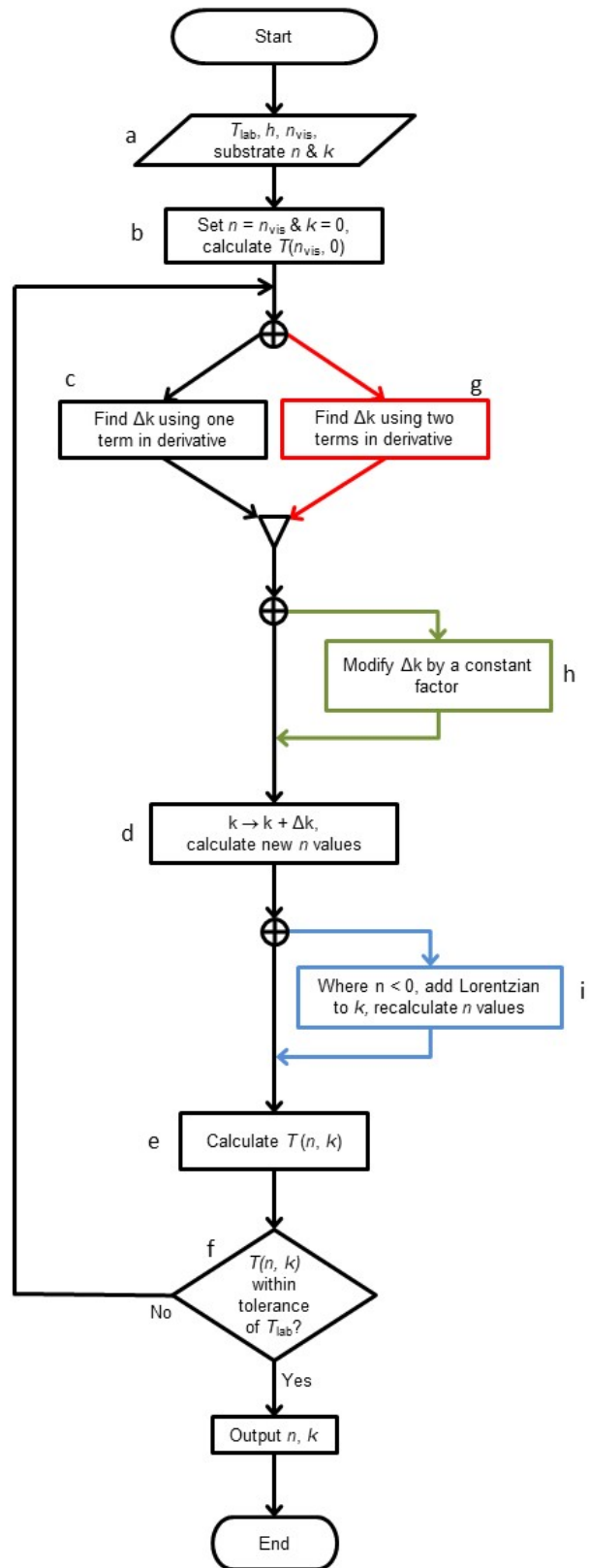
Figure 1. Flow chart of the algorithm used to extract the optical constants n and k from the infrared transmission spectrum of an ice film. The path in black represents the algorithm presented by previous authors. The side paths in red, green, and blue represent optional subroutines in our code that overcome conditions that could cause the standard path to fail. The details of each step are described in the text.
