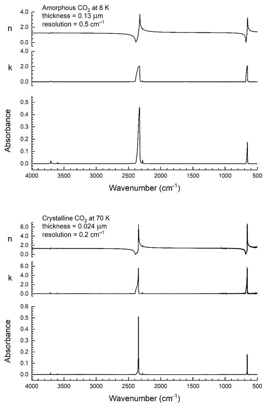
Figure 4. Top panel: Measured IR absorbance, and calculated values of n and k for amorphous CO 2 at 8 K. Absorbance shown for a sample thickness of 0.13 \mu\text{m} , measured with a resolution of 0.5 \text{cm}^{-1} from 4000 to 500 \text{cm}^{-1} . Bottom panel: Crystalline CO 2 at 70 K, with a thickness of 0.024 \mu\text{m} , measured with a resolution of 0.2 \text{cm}^{-1} from 4000 to 500 \text{cm}^{-1} .
