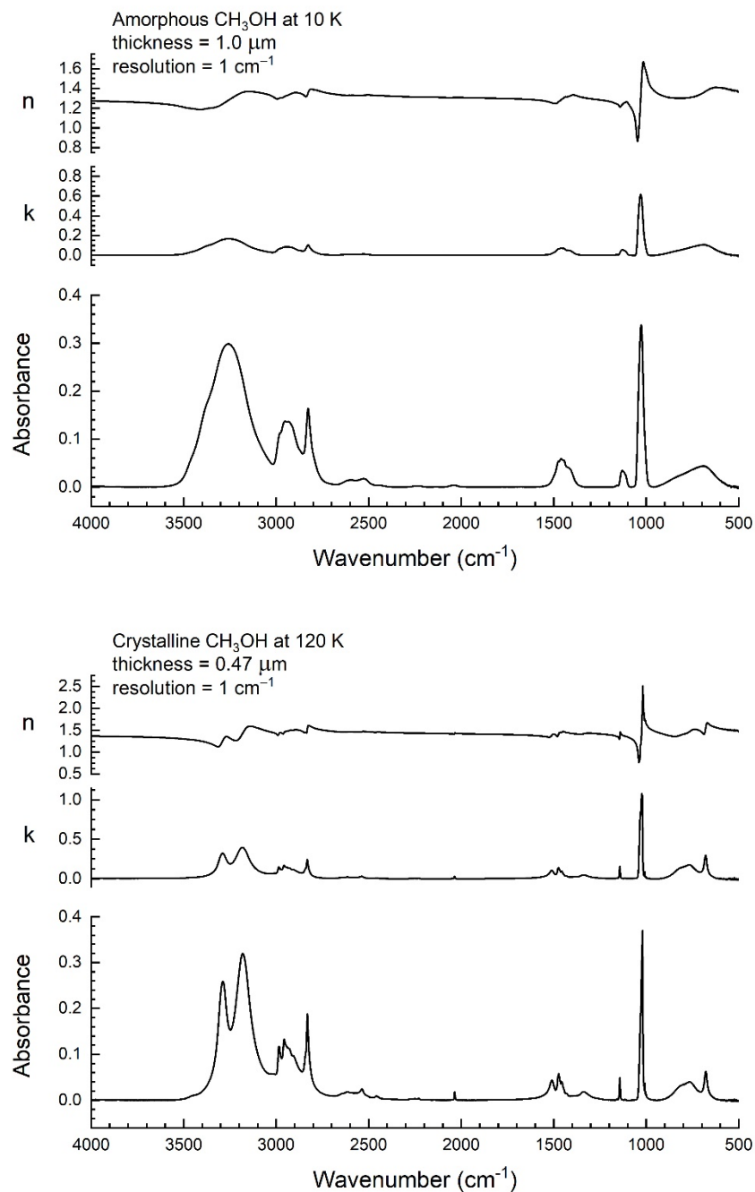
Figure 2. Top panel: Measured IR absorbance, and calculated values of n and k for amorphous CH 3 OH at 10 K. Absorbance shown for a sample thickness of 1.0 \mu\text{m} , measured with a resolution of 1 \text{cm}^{-1} from 4000 to 500 \text{cm}^{-1} . Bottom panel: Crystalline CH 3 OH at 120 K, with a thickness of 0.47 \mu\text{m} , measured with a resolution of 1 \text{cm}^{-1} from 4000 to 500 \text{cm}^{-1} .
