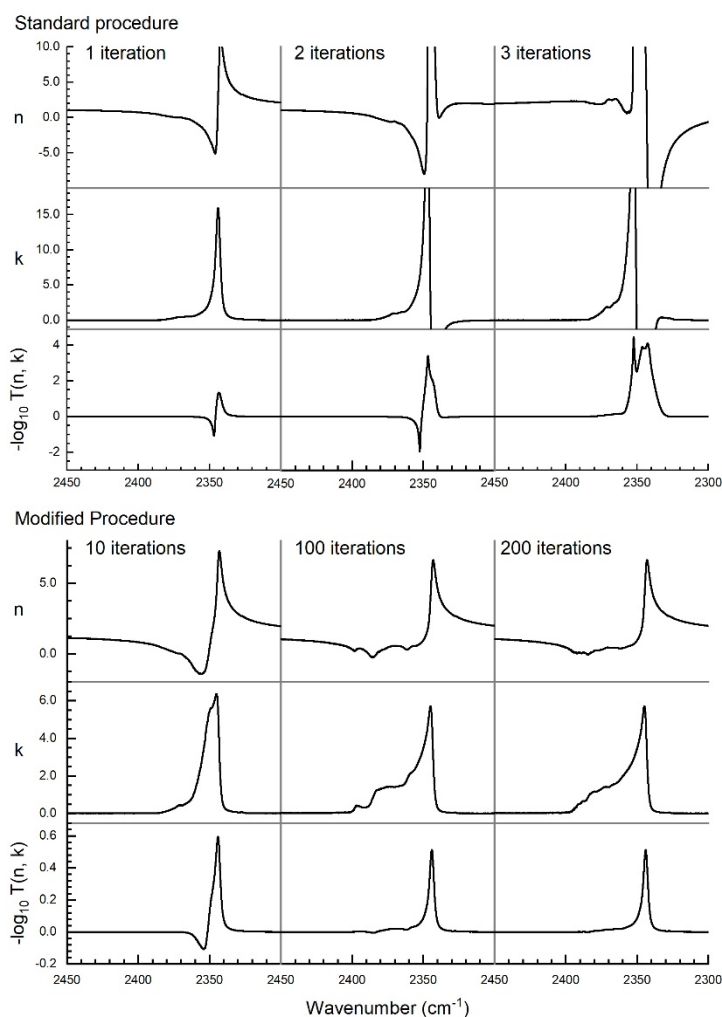
Figure 5. Iteration results using the standard (top panels) and our modified (bottom panels) procedures for determining optical constants, using the case of the IR spectrum of crystalline CO 2 as an example and shown in the range \tilde{\nu} = 2450\text{--}2300\text{ cm}^{-1} . In the upper set of panels, the standard procedure from the literature was used. In the lower panels, the modified procedure was used, allowing the step size to vary and adding a correction term when negative n values were encountered. Details are described in the text. In the standard case, the code aborted with errors after 8 iterations, whereas the modified case proceeded until convergence.
