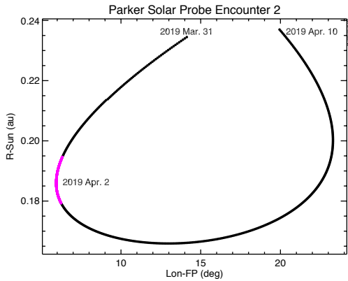
Figure 1. Parker Solar Probe solar radius vs. the spacecraft’s magnetic solar footpoint Carrington longitude, assuming a nominal Parker spiral with a solar wind speed of 350 km/s through Encounter 2 (with 2019 April 2 highlighted in magenta). The narrow range of foot point longitudes on this day show that Parker Solar Probe is in co-rotation with Sun.
