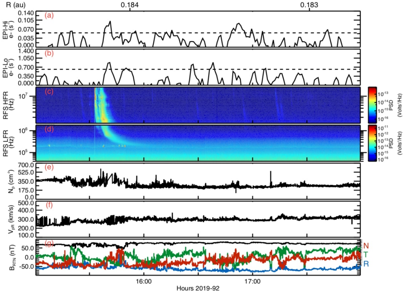
Figure 6. Overview of the time around the 2019 April 2 (DOY 92) 15:40 UTC radio and electron event. Increases in both EPI-Hi (panel a) and EPI-Lo (panel b) are observed that appear to be connected to the preceding radio burst visible in the high frequency radio data starting at 15:32 UTC (panel c), drifting down to the local plasma frequency line in the low frequency radio data (panel d). Nearly concurrent with the radio burst drifting to the local plasma frequency, a number of Langmuir waves are visible. A number of small depressions are visible in the magnetic field strength, most notably at \sim 15:47 UTC (panel g - note the use of higher cadence magnetic field data).
