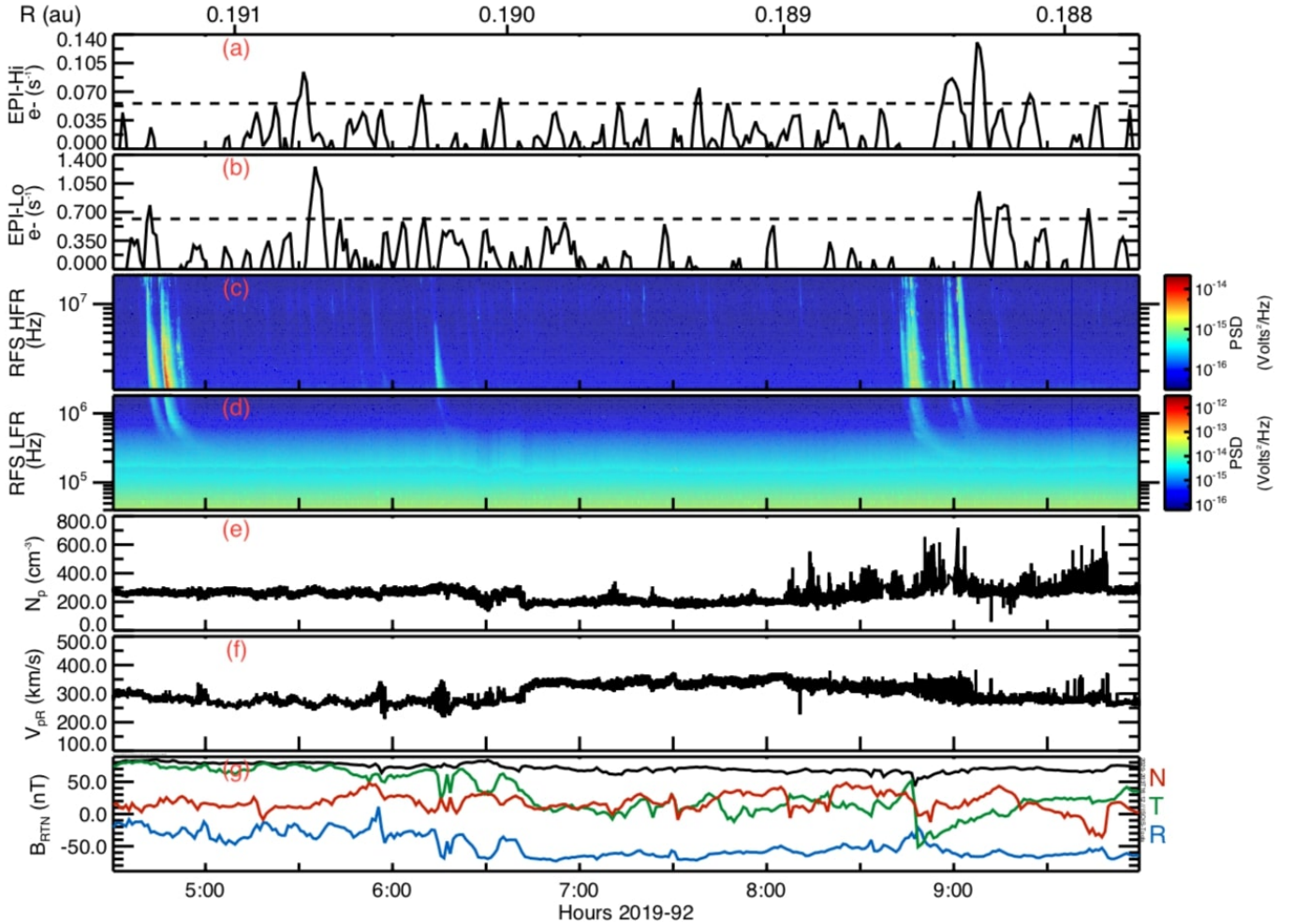
Figure 5. Overview of the time around the 2019 April 2 (DOY 92) \sim 05:40 and \sim 09:00 UTC radio and electron events. Sharp peaks in electron count rate are seen in both EPI-Hi (panel a) and EPI-Lo (panel b). Strong radio bursts are seen in the high frequency radio data (panel c) drifting down to the local plasma frequency, visible in the low frequency radio data (panel d). The tangential component of the magnetic field switches from strongly positive to strongly negative at \sim 08:50 UTC in panel g.
