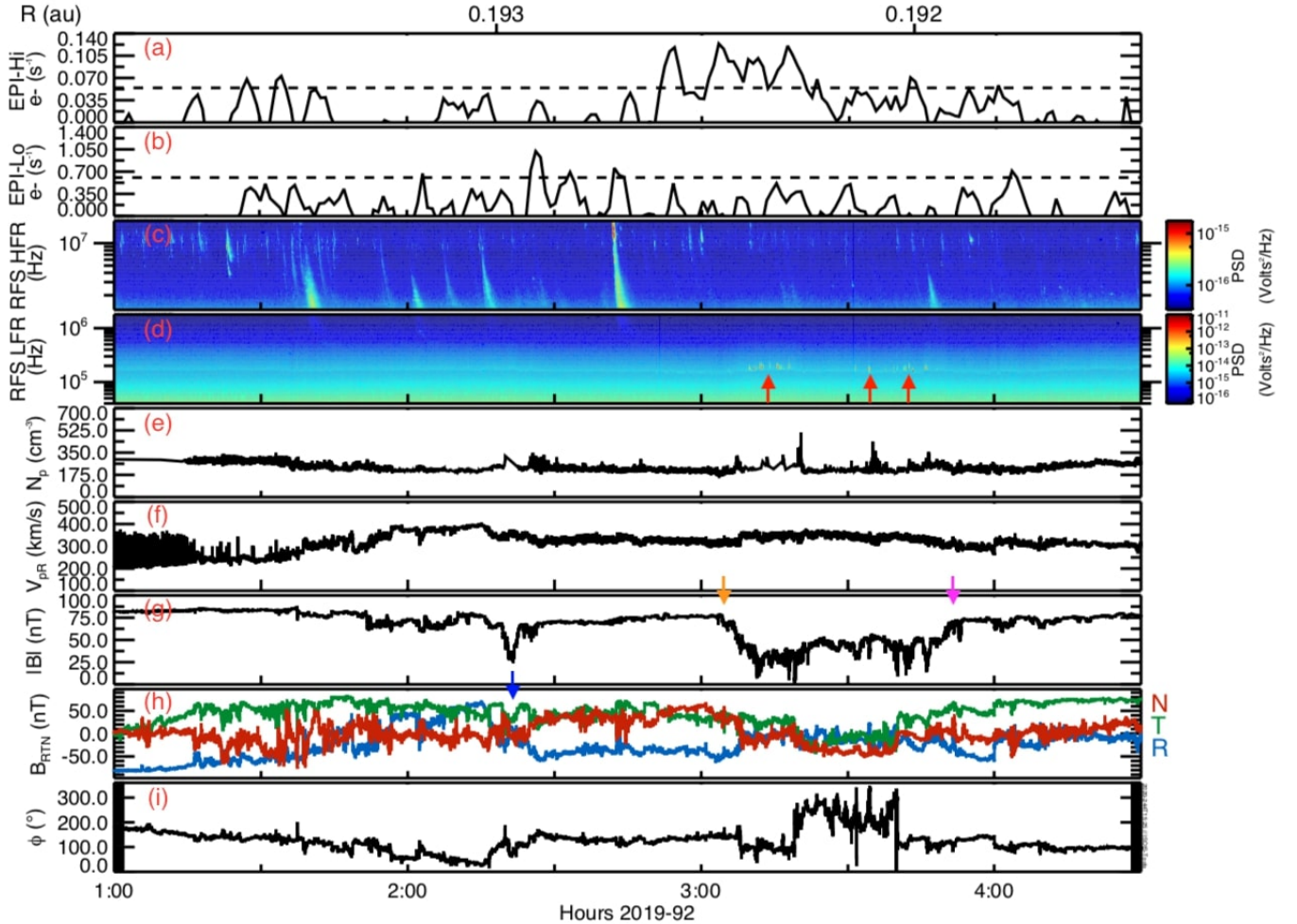
Figure 4. Overview of 01:00-04:30 UTC on 2019 April 2 (DOY 92). A prolonged increase in the EPI-Hi electron count rate is shown in panel a beginning at 02:50 UTC. No obvious accompanying increase in the EPI-Lo electron count rate is observed in panel b. Panel g shows several depressions in the magnetic field strength coupled to significant rotations in the magnetic field vector shown in panel h (Note - higher cadence magnetic field data is used in this plot to accurately portray the timing of these features). The azimuthal magnetic field angle is shown in panel i to show these rotations. Some of these magnetic depressions appear to have associated Langmuir waves visible in the low frequency radio data along the local plasma frequency (indicated with red arrows in panel d). A number of type III radio bursts are observed throughout this time period in the high frequency radio data (panel c).
