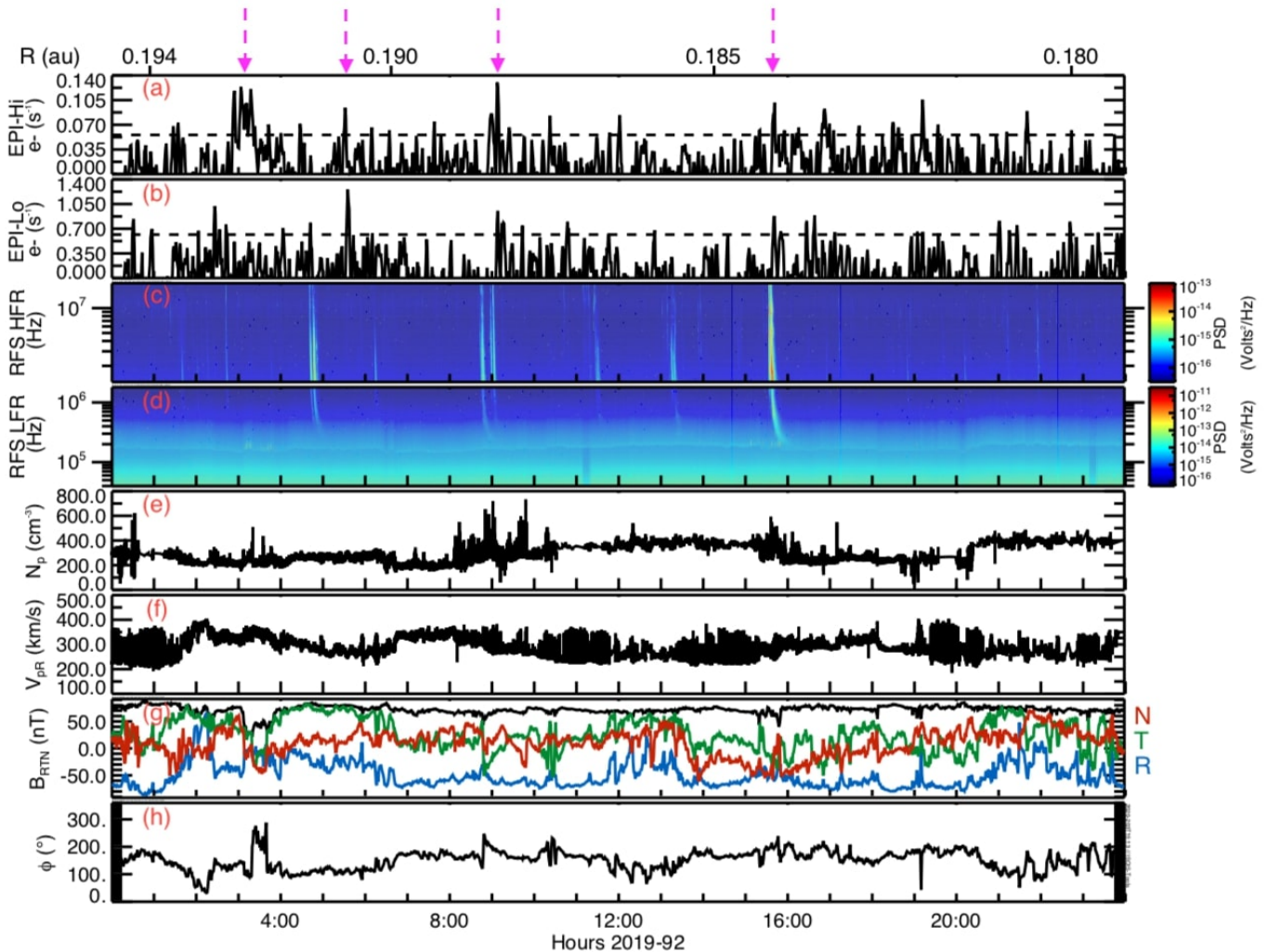
Figure 3. Overview of 2019 April 2 (DOY 92) following the format of Figure 2 but with the addition of the azimuthal magnetic field angle (in RTN coordinates) in panel h. Electron events of particular interest during this day occur at approximately 03:00, 05:00, 09:00, and 15:40 UTC in the top two panels. Arrows at the top of the figure indicate events that will be highlighted in this work.
