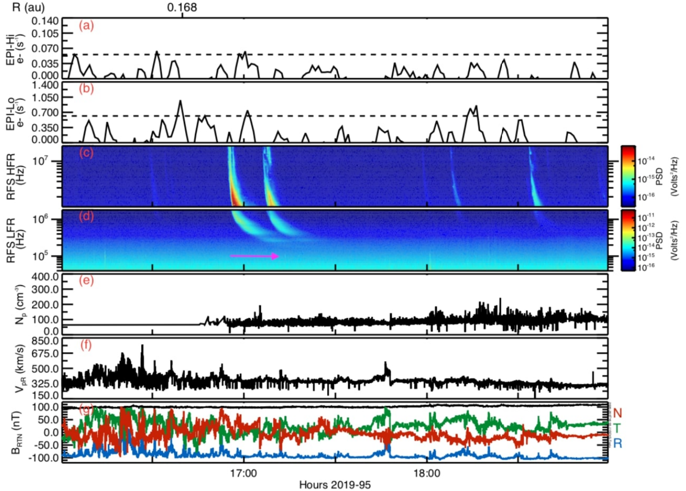
Figure 7. Overview of the time around the 2019 April 5 (DOY 95) 17:00 UTC radio and electron event. A strong radio burst is visible in the high frequency radio data starting at 16:55 UTC (panel c), drifting down to the local plasma frequency line in the low frequency radio data (marked by the magenta arrow in panel d). Marginal increases in both EPI-Hi (panel a) and EPI-Lo (panel b) at \sim 17:00 UTC are observed that may be connected to this radio burst.
