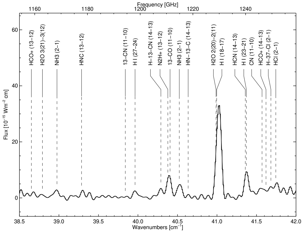
Figure A9. SPIRE spectrum 38.5 to 42.0 \text{cm}^{-1}
