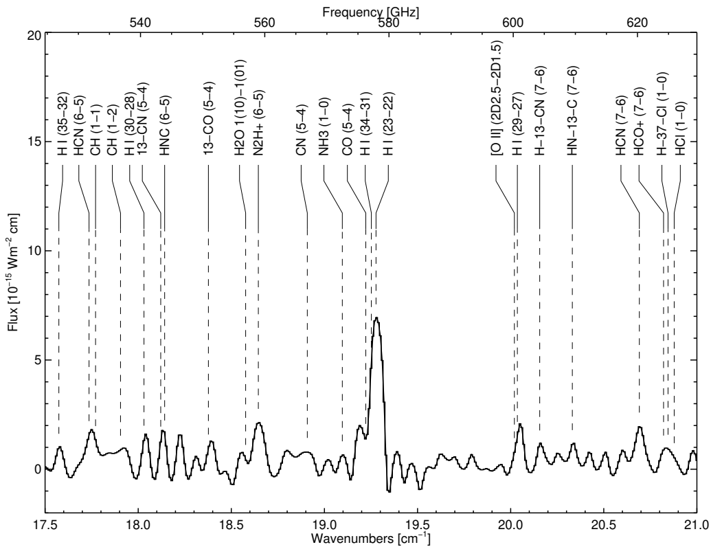
Figure A2. SPIRE spectrum 17.5 to 21.0 \text{cm}^{-1}
