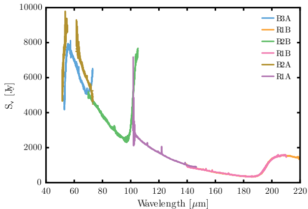
Figure 3. The SED of \eta Car as measured by the central spaxel (labeled 2,2 in figure 2). Wavelength ranges for each grating order are given in Sec. 2.1. \eta Car and its ejecta are the brightest extrasolar source at 25 \mu\text{m} . Hence short wavelength continuum dominates in this spectral region, inflicting saturation in B2A and filter leakage longward of 190 \mu\text{m} in the R2 spectral scan. Likewise a filter leak from third order into second order is present in B2B from 95 to 105 \mu\text{m} and leakage from fourth order is present in B3A longward of 70 \mu\text{m} . The very small peaks against the strong continuum, as seen in the R1A and R1B spectral segments, are the stronger emission lines studied in this paper with PACS.
