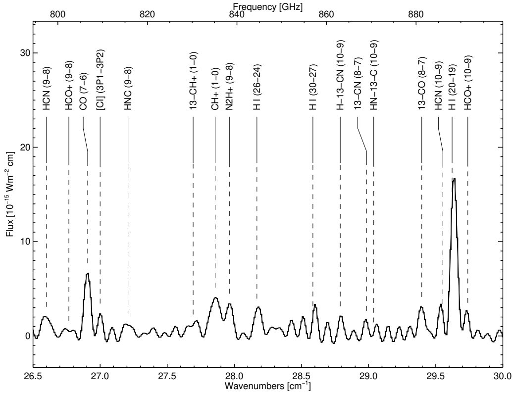
Figure A5. SPIRE spectrum 26.5 to 30.0 \text{cm}^{-1}
