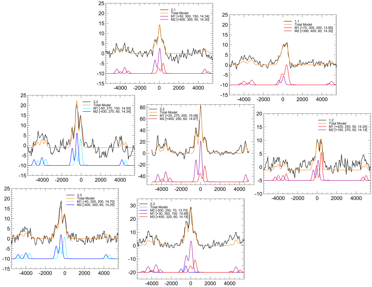
Figure 9. NH N = 2-1 profiles observed at seven positions on the Homunculus, with synthetic spectra comparisons. Each plot shows LSR velocity in \text{km s}^{-1} (referenced to the vacuum wavelength 153.450 \mu\text{m} of the highest transition probability J=3-2 , F_1=7/2-5/2 line) vs. line flux in Jy and are arranged to correspond schematically to the spaxel positions in Figure 2. All observed profiles are fitted with two velocity components, except for a 3-component model for spaxel (2,3). Total synthetic fits are shown in orange. Individual model components are offset for clarity and colored to indicate LSR velocity shift ranges of < -100 \text{ km s}^{-1} (blue), -100 to 0 \text{ km s}^{-1} (cyan), 0 to +100 \text{ km s}^{-1} (violet), and > +100 \text{ km s}^{-1} (red). For each model component, the LSR velocity (in \text{km s}^{-1} ), FWHM ( \text{km s}^{-1} ), excitation temperature (K), and log column density ( \text{cm}^{-2} ) are given in the legend. Details on the modeling are given in the text. Features not fitted near -1000 \text{ km s}^{-1} and +4000 \text{ km s}^{-1} are due to \text{NH}_2 and \text{H}18 \beta , respectively.
