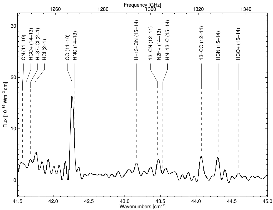
Figure A10. SPIRE spectrum 41.5 to 45.0 \text{cm}^{-1}
