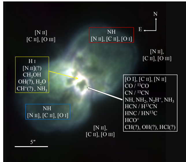
Figure 15. A false color mid-infrared 9.0 \mu\text{m} image of \eta Car with bulk locations of the atomic and molecular species detected in the PACS and SPIRE spectral survey as summarized in Sec. 4. The color scheme provides a good association of the white high contrast emission defining the Butterfly Nebula and species in the white box. Species surmised to originate within 1'' of the central source (i.e., 2'' across) are indicated in the yellow box. The red and blue boxes contain molecules associated with the expanding lobes (or break-out material of the equatorial skirt). Detected background species are indicated without boxes. The image was taken with the VLT/VISIR instrument through the [Ar III] filter (Mehner et al. 2019), sampling the T \geq 400 K continuum.
