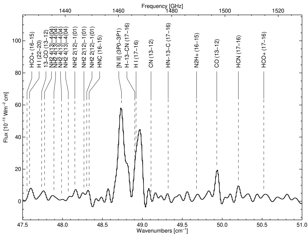
Figure A12. SPIRE spectrum 47.5 to 51.0 \text{cm}^{-1}
