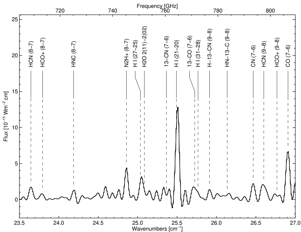
Figure A4. SPIRE spectrum 23.5 to 27.0 \text{cm}^{-1}
