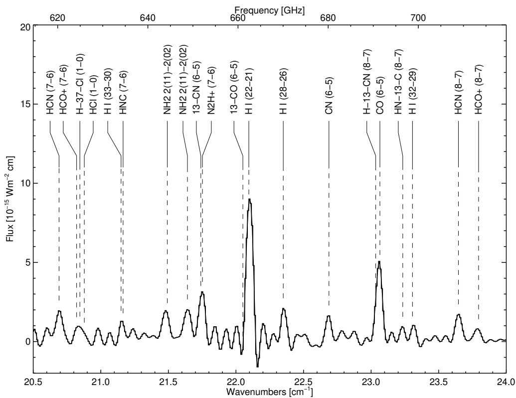
Figure A3. SPIRE spectrum 20.5 to 24.0 \text{cm}^{-1}
