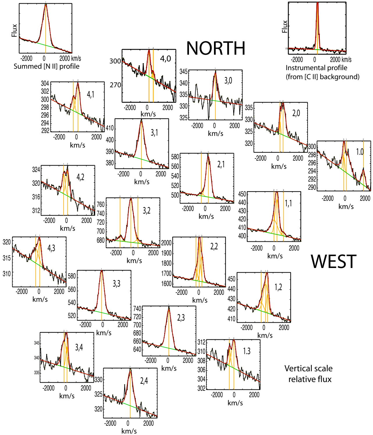
Figure 6. [N II] line profiles on the Homuculus. In the top left corner is shown the [N II] profile summed over the entire PACS array. The top right shows the PACS spectrometer profile of the unresolved background line of [C II] 157.736 \mu\text{m} . The spectral resolution at 121 \mu\text{m} is \sim 30\% lower. In the centre is shown the mosaic of [N II] velocity profiles. The profiles, labeled with spaxel number, are arranged to reflect the spaxel positions shown in Figure 2. The summed profile, centered on 3 \text{ km s}^{-1} has a FWHM of 804 \text{ km s}^{-1} . However the peak flux, velocity FWHM and central velocity change from spaxel to spaxel. Profile variations are consistent with [N II] emission from the Homunculus and the external, fast-moving ejecta.
