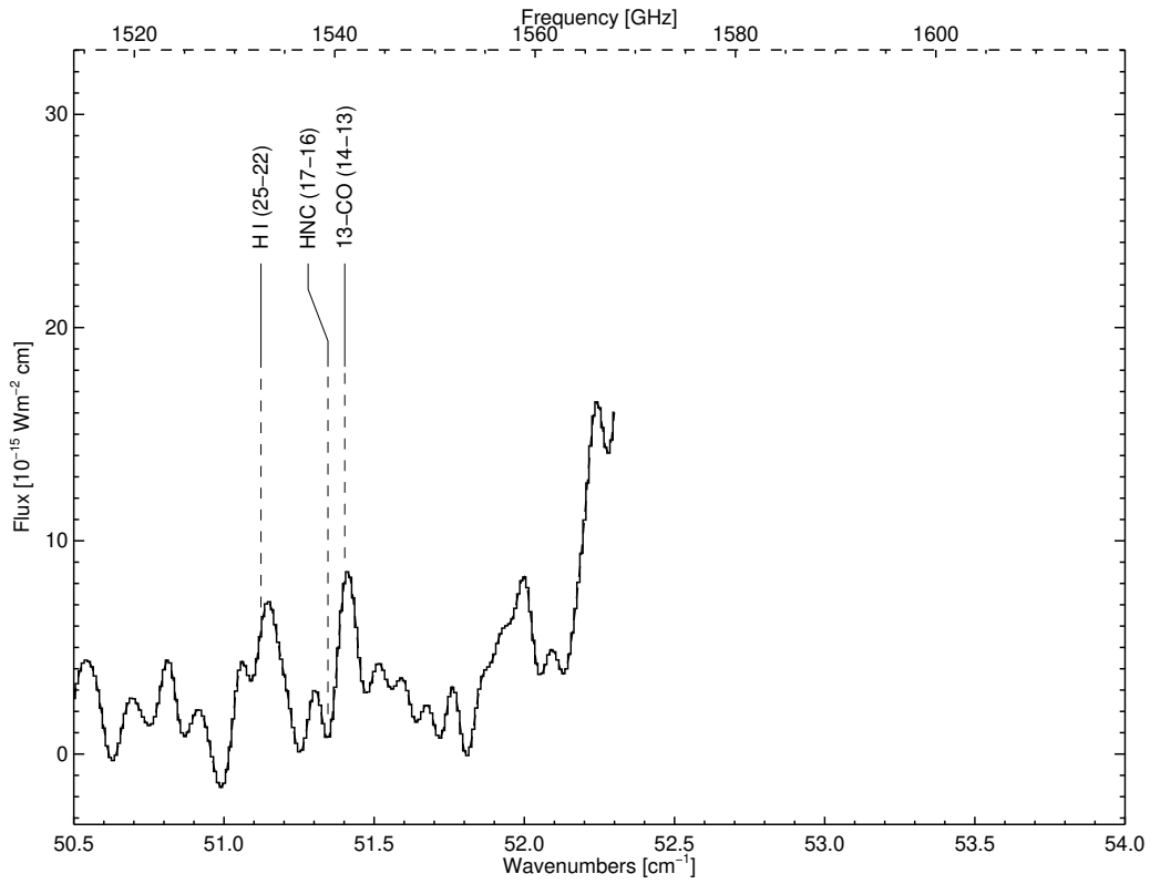
Figure A13. SPIRE spectrum 50.5 to 54.0 \text{cm}^{-1} . Note that while the plot extends out to 52.3 \text{cm}^{-1} , the spectrum is not reliable beyond 51.5 \text{cm}^{-1} with the last line tabulated in Table A1 at 51.4 \text{cm}^{-1} .
