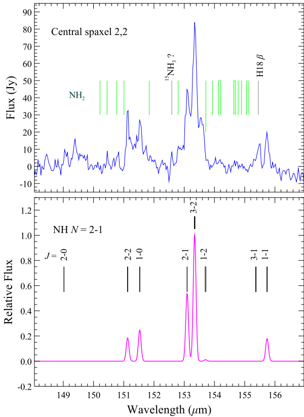
Figure 8. NH N = 2-1 complex between 151 to 156 \mu\text{m} . Top: continuum-subtracted spectrum centered on \eta Car with vacuum wavelengths shown for H18 \beta , a weak, low significance identification of ^{15}\text{NH}_3 , and \text{NH}_2 transitions all with upper level energies below 1000 K. The spatial extent of NH coincides with the Homunculus lobes and skirt as demonstrated in Figure 9. Bottom: A reference non-LTE model of NH over the full range of full range of spin-rotation-hyperfine components, computed at 100 K and zero LSR velocity, convolved with the PACS resolution of 0.05 \mu\text{m} at 150 \mu\text{m} . The width of fiducial lines at each J state indicates the range of hyperfine transitions. Note that three of the eight spin rotation components contribute practically no measurable emission, consistent with their low transition probabilities.
