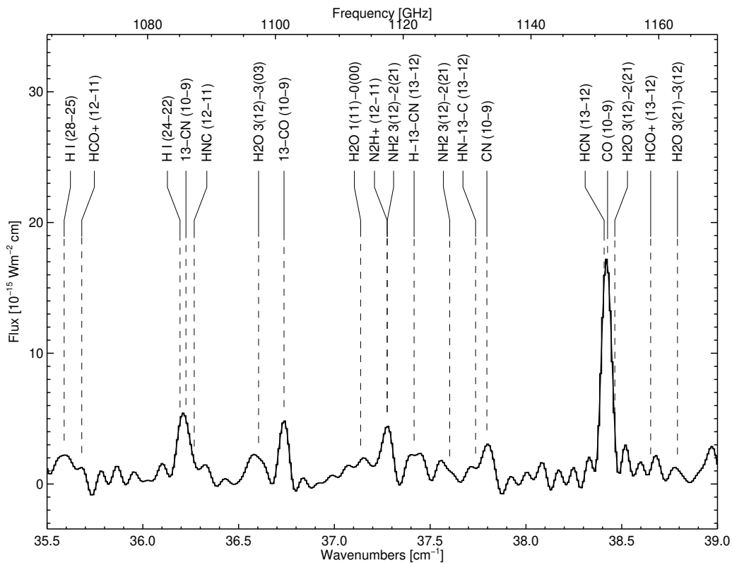
Figure A8. SPIRE spectrum 35.5 to 39.0 \text{cm}^{-1}
