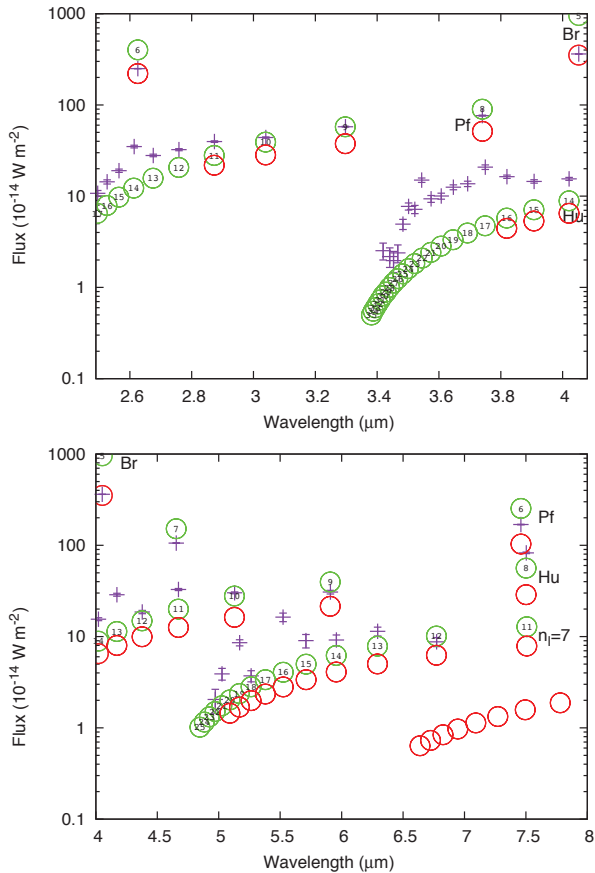
Figure 14. Excitation diagram for the mid-infrared hydrogen lines observed with ISO/SWS . The integrated fluxes of the H I Br, Pf, Hu, and n_l = 7 series are shown as violet crosses as a function of wavelength. The upper-state quantum numbers are indicated inside the green circles, which show fluxes expected in LTE at T_e = 10^4 K when reddened by an interstellar extinction curve with A_V = 5 mag. The red circles show the predicted fluxes of the non-LTE capture-cascade model used to analyze the far-infrared Herschel spectra.
