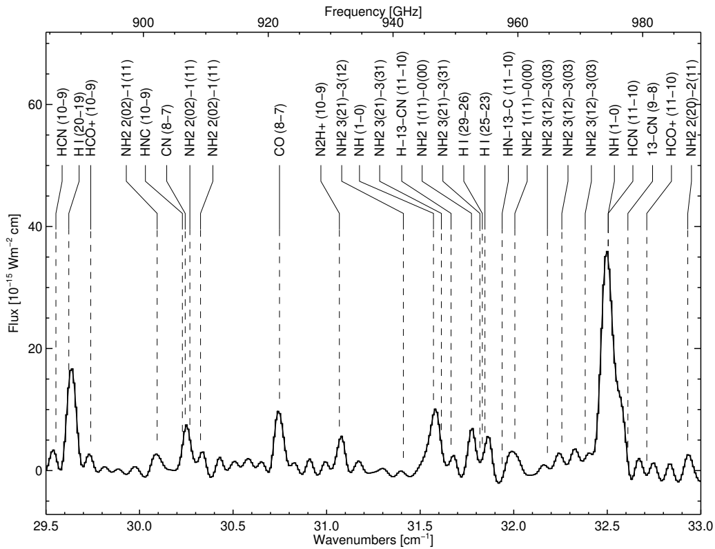
Figure A6. SPIRE spectrum 29.5 to 33.0 \text{cm}^{-1}
