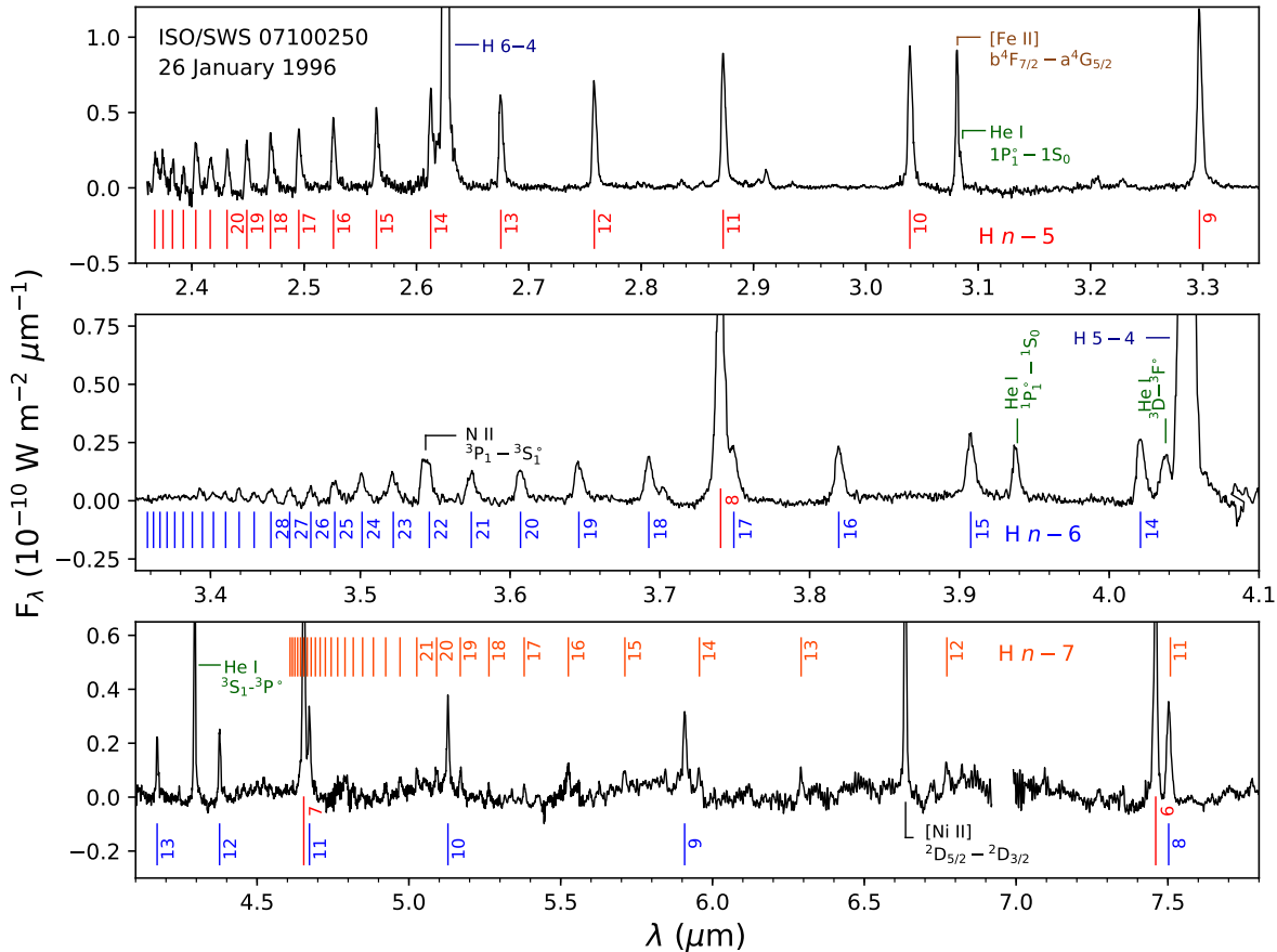
Figure 12. The continuum-subtracted ISO/SWS spectrum of \eta Car over the first 5 grating sub-bands of the S01 spectral scan obtained in 1996. The continuum rises from 2.5 \times 10^{-10} to 6.2 \times 10^{-10} \text{W m}^{-2} \mu\text{m}^{-1} (500 to 2050 Jy) over this range. The H I lower quantum state n_l = 5 (Pfund), 6 (Humphreys), and 7 series are indicated, along with the Brackett \alpha (5 – 4) line and identifications for leading lines of other atomic species. The spectral resolution R = 1500 - 2000 , or 200 \text{ km s}^{-1} at 3.0 \mu\text{m} .
