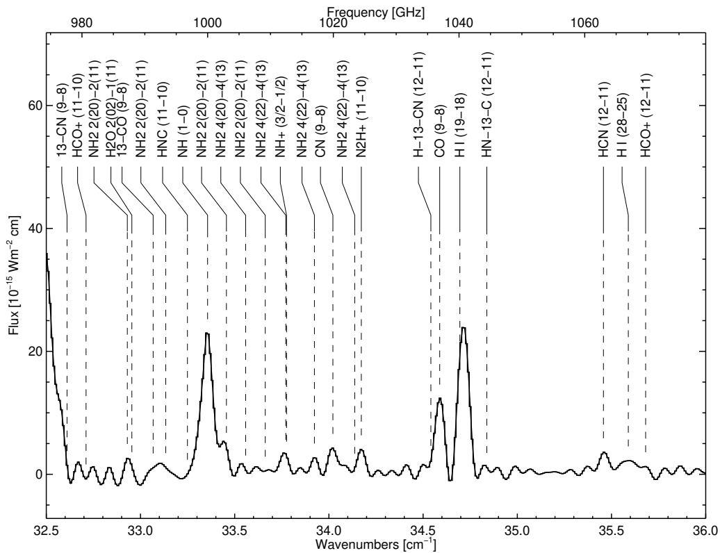
Figure A7. SPIRE spectrum 32.5 to 36.0 \text{cm}^{-1}
