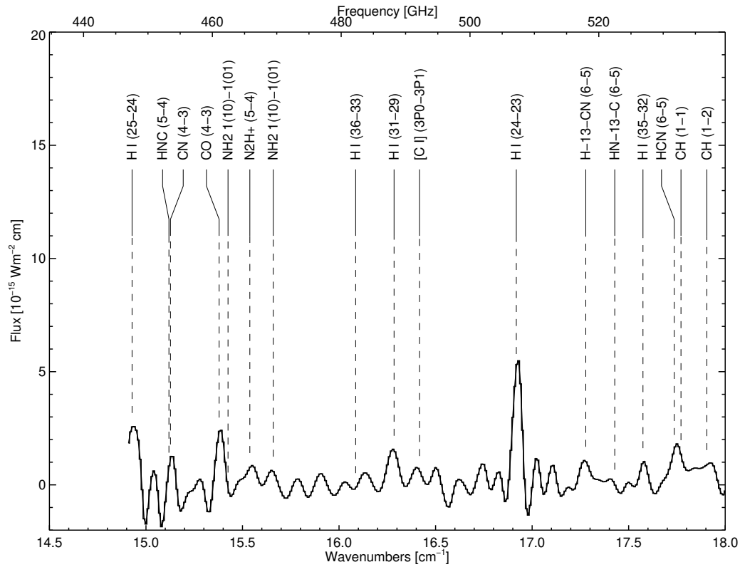
Figure A1. SPIRE spectrum 14.5 to 18.0 \text{cm}^{-1} . As commented in section 2.2, the S/N exceeds 100 over most of the spectrum depicted in Figures A1 through A13. Most of the features in these spectra are real and promise to reveal even more line identifications. Note that, for all of the following spectral plots, the strong continuum has been subtracted to provide an optimized baseline for line identification.
