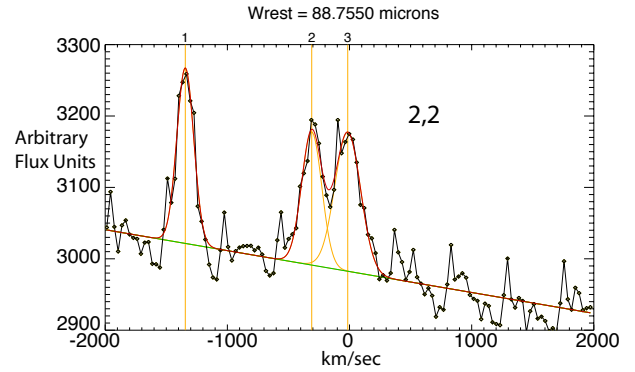
Figure 5. H I 13-12 ( 88.755 \mu\text{m} ) line profile measured by PACS, centered on \eta Car. The line labeled '1' corresponds to background [O III] 88.36 \mu\text{m} . The H I emission feature labeled '3' is blended with an unidentified transition, labeled '2'. LSR velocities are referenced to the H I 13-12 rest wavelength. The line is detectable within only four spaxels, strong on spaxel 2,2, and weak in three nearby spaxels which is consistent with a nearly point-like source compared to the PACS spatial response. The width of the [O III] emission line is close to the instrumental profile, with a FWHM measuring 150 \text{ km s}^{-1} .
