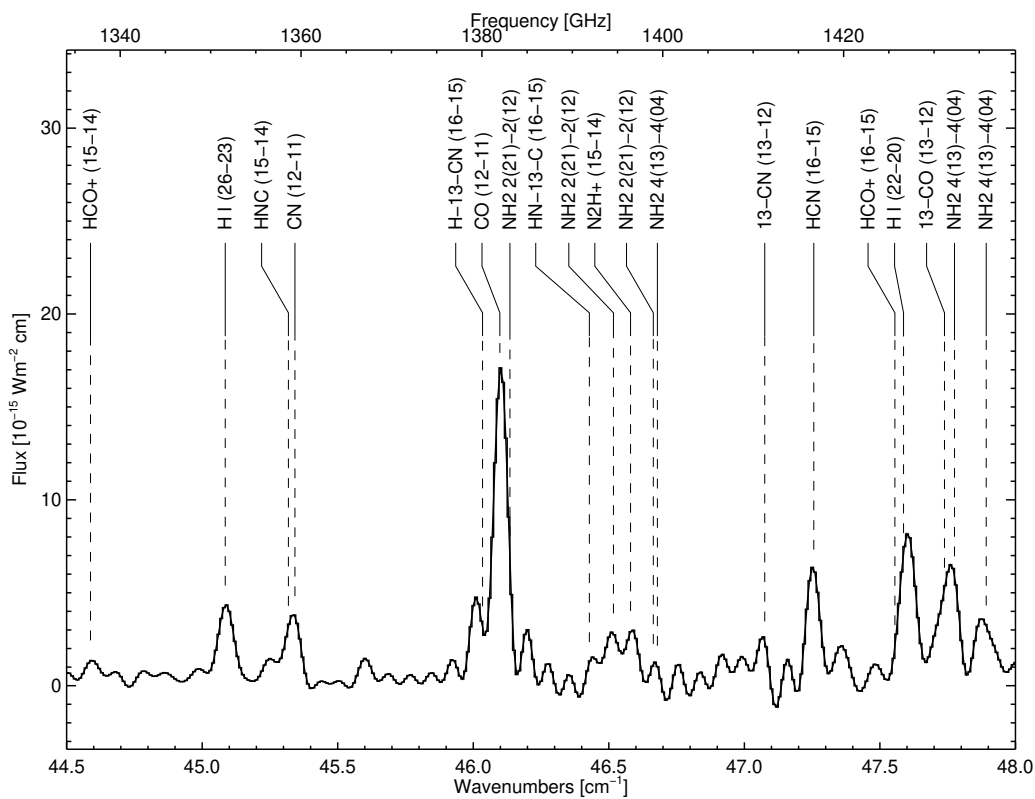
Figure A11. SPIRE spectrum 44.5 to 48.0 \text{cm}^{-1}
