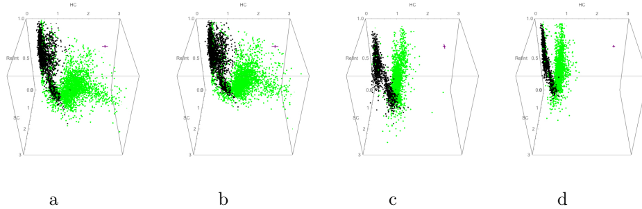
Figure 4: Color-Color-Intensity plots using MAXI/GSC data extracted in four of the X-ray colors listed in Table 2. The HMBHs are plotted in black and the LMBHs in green. The average error bar is plotted as purple cross on each plot. (a) : Using CR1; (b) : Using CR2; (c) : Using CR3; (d) : Using CR4. LMBHs are separated from HMBHs by all four colors. CR1 and CR2 capture the soft states whereas CR3 and CR4 do not.
