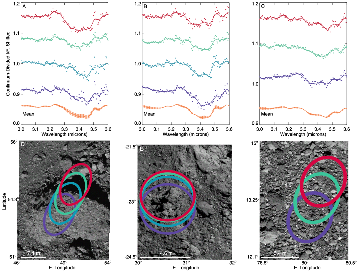
Fig. 4. Individual high-areal-resolution ( \sim 60 \text{ m}^2 ) local spectra, and their corresponding OVIRS footprints. (A-C) Spectra of selected locations and their means. (D-F) The corresponding OVIRS footprints (ellipses, elongated by along-track motion) overlain on OCAMS panchromatic images acquired at the same time. In (A), a deep absorption feature changes spectral shape and depth as the field of view moves off a large boulder and onto smaller boulders (D), which could have different composition, and the mean shows variation over the full band. In (B), a cluster of spectra over a rock pile (E) shows consistent shapes with less variation in the mean than in (A). In (C), a region with little absorption shows few large boulders in the field of view (F) and similar variation in the mean as (B).
