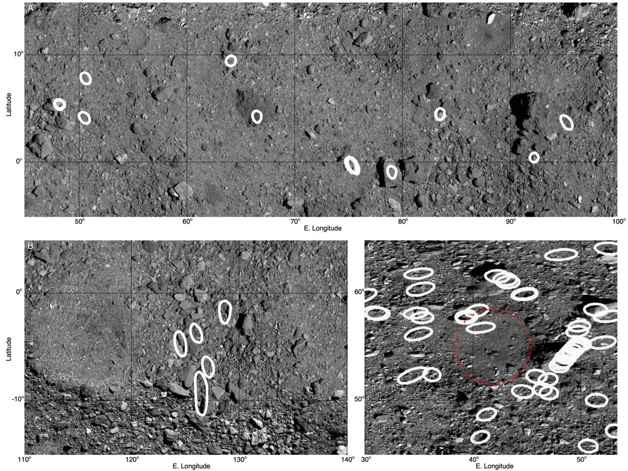
Fig. 5. The locations and sizes of OVIRS footprints (white outlines) of spectra with single-channel absorptions >5% at either 3.42, 3.45 or 3.47 \mu\text{m} . The footprints are overlaid on the 5-cm-resolution base map (26, 27); they are elongated by surface projection effects but neglect along-track smear. Footprint coverage over the images is sparse, primarily in separated north-south scans. (A) Low latitudes show a number of deep absorptions, primarily over boulders. (B) An adjacent equatorial region shows that the boulders between two craters also have deep absorptions. (C) The environs around the OSIRIS-REx primary sample site, Nightingale crater (dashed circle), also show locally deeper absorptions.
