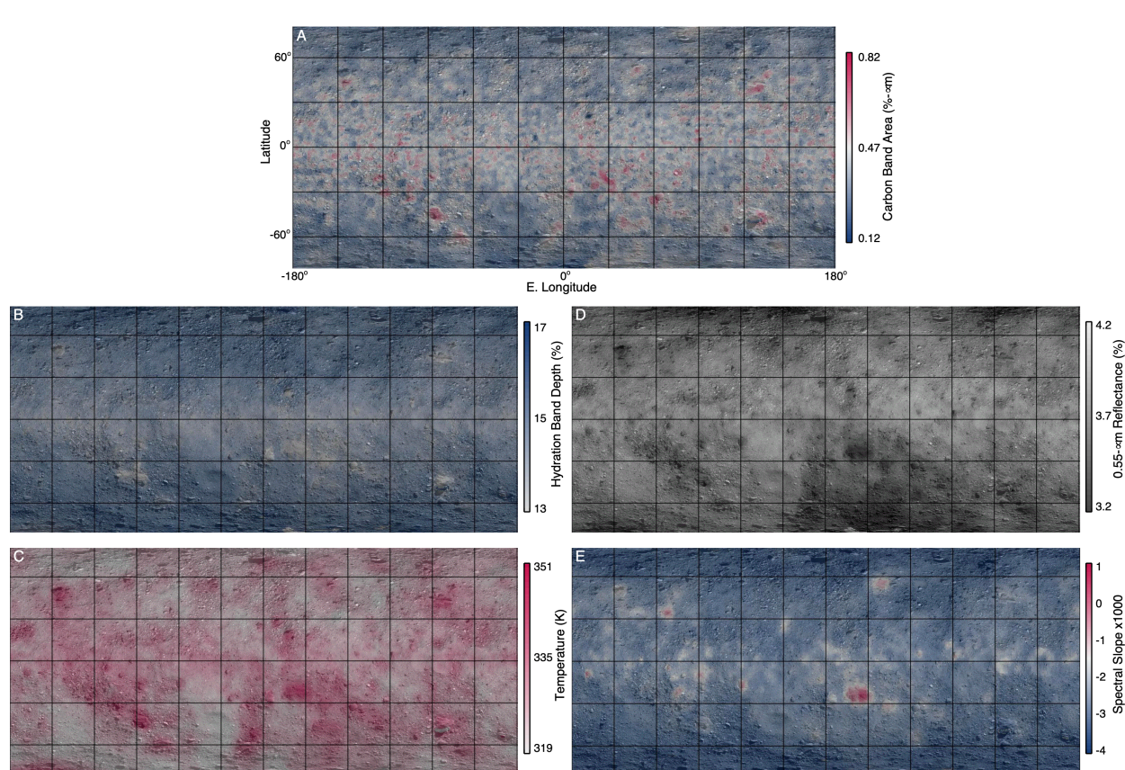
10 Fig. 3. Global spectral maps of Bennu from the OVIRS observations taken at the 12:30 pm Equatorial Station. (A) Band area from 3.2 to 3.6 µm, showing absorption due to carbon-bearing materials. (B) 2.74-µm hydration band depth, (C) effective surface temperature, (D) 0.55-µm reflectance, and (E) spectral slope from 0.5 to 1.5 µm. The latitude and longitude grid shown in A is overlain on the other panels. 15
