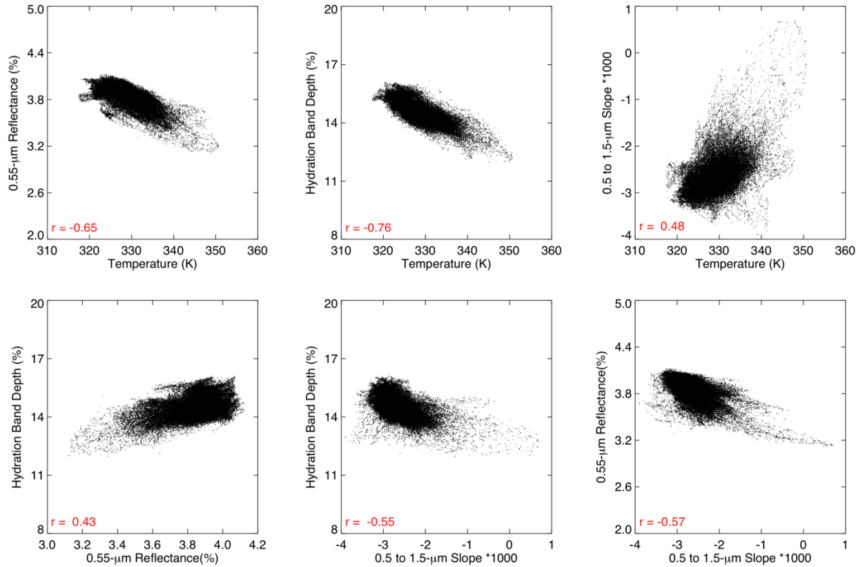
Fig. S3. Correlation plots for the map pairs shown in Fig. 3. Map pairs of 0.55- \mu\text{m} reflectance (Fig. 3D) vs. surface temperature (Fig. 3C), hydration band (Fig. 3B) vs. surface temperature (Fig. 3C), spectral slope (Fig. 3E) vs. surface temperature (Fig. 3C), 2.74- \mu\text{m} hydration band (Fig 3B) vs. reflectance (Fig. 3D), 2.74- \mu\text{m} hydration band (Fig 3B) vs. spectral slope (Fig. 3E), and 0.55- \mu\text{m} reflectance (Fig. 3D) vs. spectral slope (Fig. 3E). The Spearman's rank correlation coefficient is listed for each pairing.
