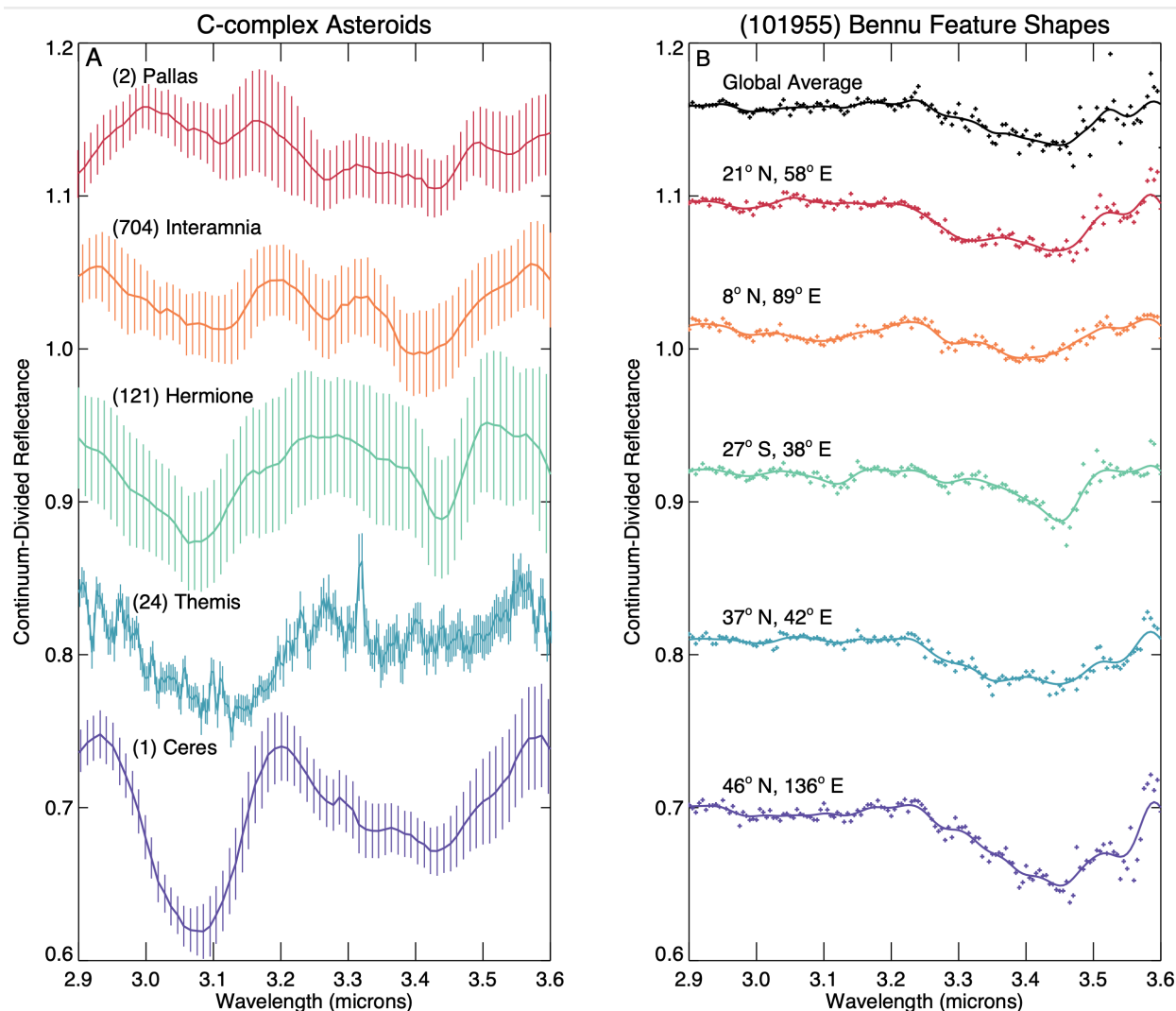
Fig. 1. Comparison of 3.4- \mu\text{m} absorption features on main belt asteroids and multiple locations on Benu. (A) C-complex asteroid spectra obtained at 15^\circ to 30^\circ phase angle (22) - except the (24) Themis data from (18) - each plotted with 1\sigma uncertainties. Curves are offset from 1.0 for clarity. (B) The OVIRS globally averaged Benu spectrum at 9^\circ phase angle shows a broad absorption feature of \sim 2\% depth, extending from 3.2 to 3.6 \mu\text{m} . The solid line shows the spectrum smoothed with a 9-spectral channel width Gaussian. Spectra of individual locations on Benu are also shown, the coordinates of each location labelled, and curves are offset from 1.0 for clarity. Uncertainties are smaller than the symbol size.
