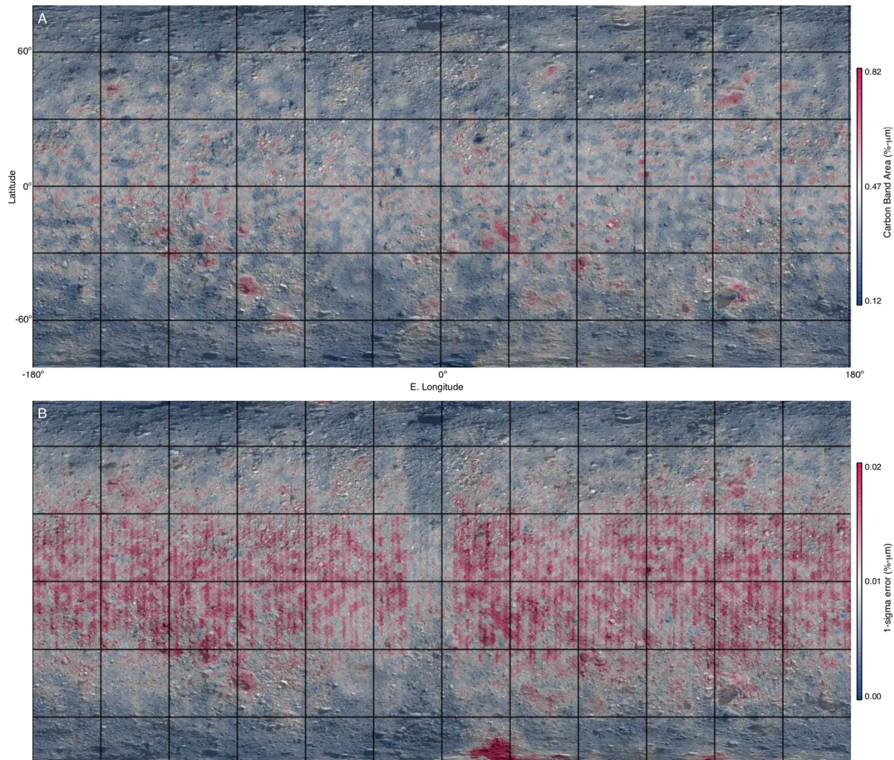
Fig S6. Carbon band area and error map for 3.2 to 3.6 μm at 12:30 pm. (A) Higher resolution version of the map shown in Fig. 3A. (B) The corresponding 1σ standard error map.
