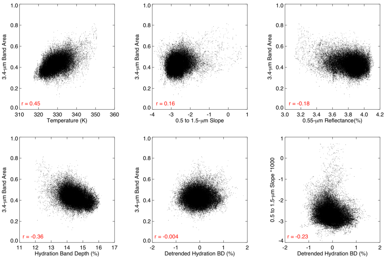
Fig. S5. Correlation plots for the 3.2 to 3.6- \mu\text{m} band area map. As in Fig. S3, but for map pairs of Fig. 3A vs. surface temperature (Fig. 3C), hydration band (Fig. 3B), reflectance (Fig. 3D), spectral slope (Fig. 3E), and temperature-detrended hydration band depth (Fig. S4) maps.
