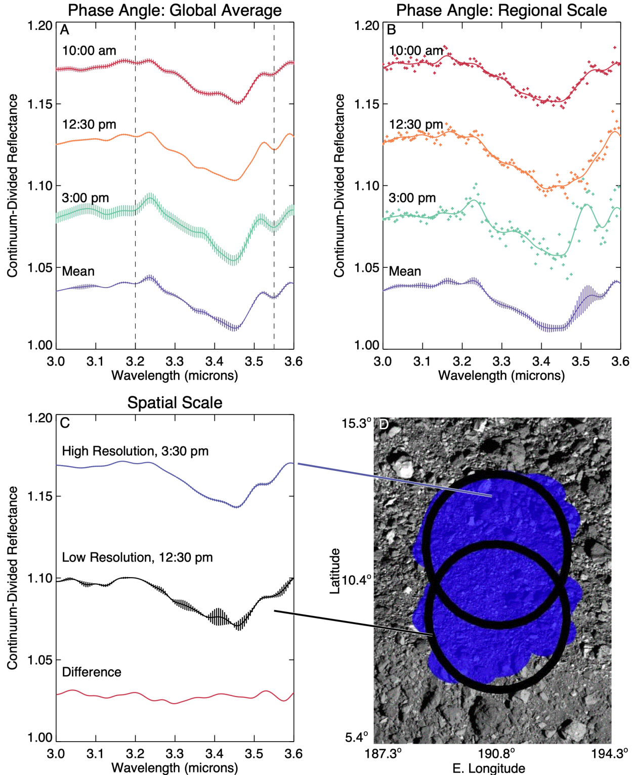
Fig. 2. Effect of local solar time (phase angle) and spatial scale on absorption feature shapes and depths. (A) Globally averaged spectra at 10:00 am ( \sim 30^\circ phase), 12:30 pm ( \sim 9^\circ ), and 3 pm ( 45^\circ ) local solar time, and the mean across all three phase angles; hatching indicates the standard
