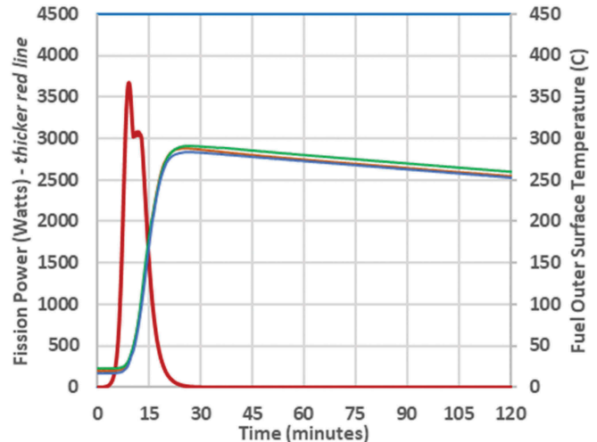
Fig. 11. Extended power and temperature data from 30 \phi run.
