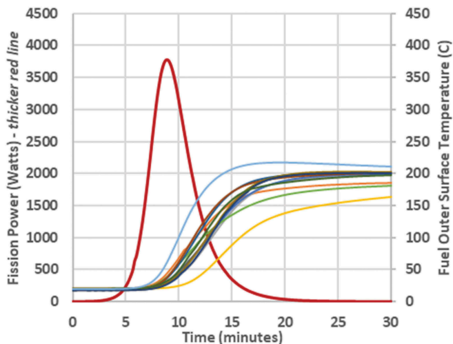
Fig. 7. Power and temperature data from 15 \phi run.
