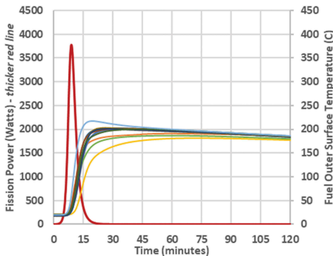
Fig. 9. Extended power and temperature data from 15 c run.
