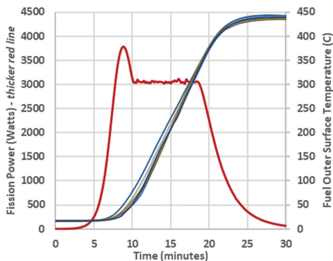
Fig. 12. Power and temperature data from 60 \phi run.
