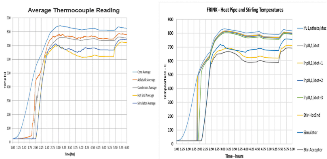
Fig. 3. Sample thermal benchmarking case from EHT results.
