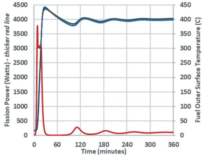
Fig. 13. Power and temperature data from 6-h, 60 \phi run.
