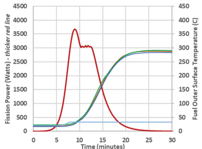
Fig. 10. Power and temperature data from 30 c run.
