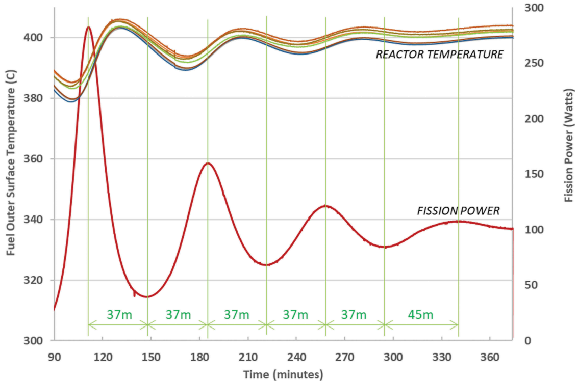
Fig. 15. Period of oscillation for the 6-h, 60 \phi run.
