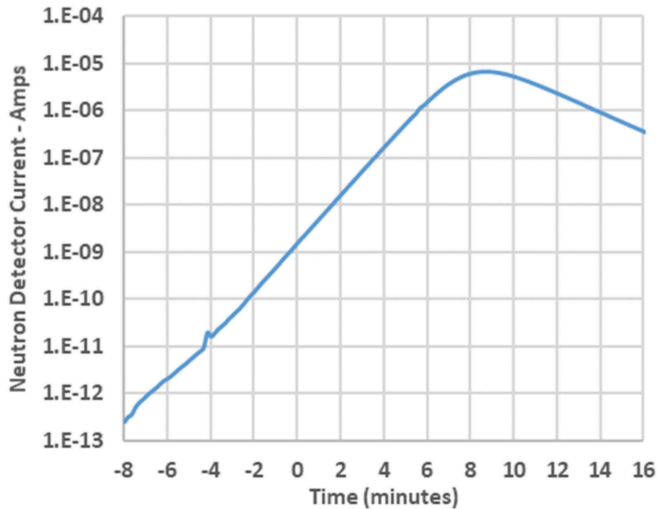
Fig. 6. Neutron detector current during 15 \phi run.
