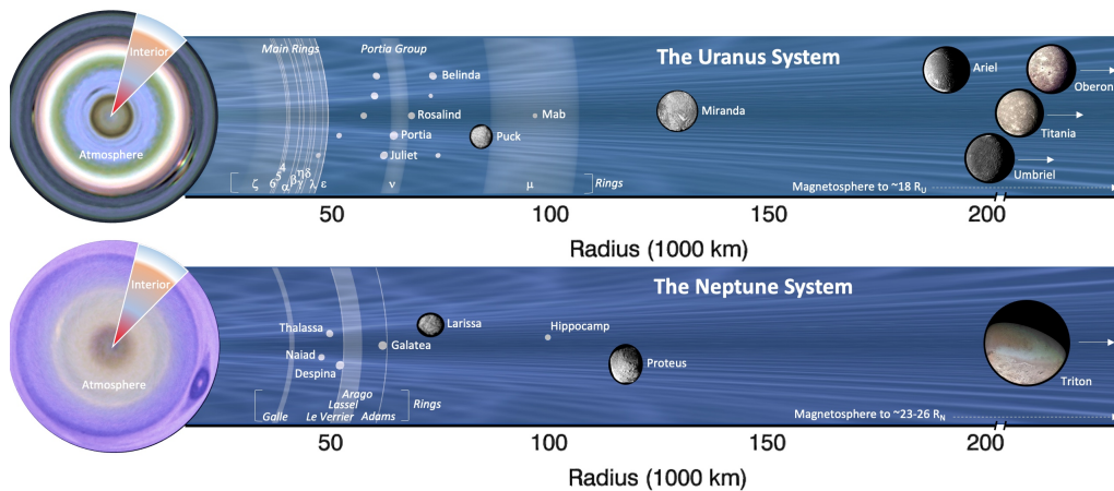
Figure 2. The Ice Giant Systems offer a rich potential for discovery, from the deep interiors, dynamic atmospheres and complex magnetospheres of the planets themselves, to the delicate rings and myriad satellites that accompany each world. The locations of rings and satellites in the inner systems are to scale with the planetary radii, with arrows next to major moons (right) indicating that they orbit at larger planetocentric distances. Relative sizes of the satellites are not to scale. Voyager images of Uranus and Neptune (left) are shown in false colour from a south-polar vantage point, with a cut-out representing the unknown density distribution of the interior. The magnetosphere and radiation belts would encompass the full area of the figure. Image modified from [14], Credit: L.N. Fletcher/M. Hedman/E. Karkoschka/Voyager-2.
