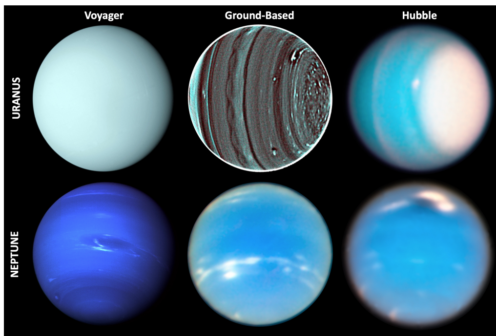
Figure 1. The evolution of Ice Giant imaging from Voyager to the present day. The left column represents our 20th-century views of Uranus (1986) and Neptune (1989) as observed by Voyager 2 (Credit: NASA/JPL-Caltech). The central column shows the best ground-based images of Uranus (near-IR from Keck in 2012, using high-contrast imaging to reveal the banded structure [13]) and Neptune (visible-light from VLT/MUSE in 2018, Credit: ESO/P. Weilbacher (AIP)). The right column shows the Ice Giants observed by the Hubble Space Telescope in 2018 (Credit: NASA, ESA, A. Simon, M.H. Wong and A. Hsu). Neptune's southern pole has been in view throughout this 30-year period, whereas Uranus was in southern summer in 1986 (left), and northern spring in 2018 (right).
