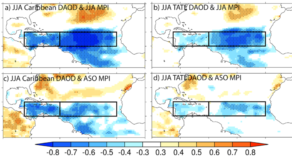
1005 Figure 9. Correlation between (a) MRC JJA regionally-averaged DAOD in the Caribbean and JJA Maximum Potential Intensity (MPI), (b) MRC JJA regionally-averaged DAOD in the tropical North Atlantic (TATL) and JJA MPI, (c) JJA Caribbean DAOD and ASO MPI and (d) JJA TATL DAOD and ASO MPI. Correlations over the black dotted areas are statistically significant.
