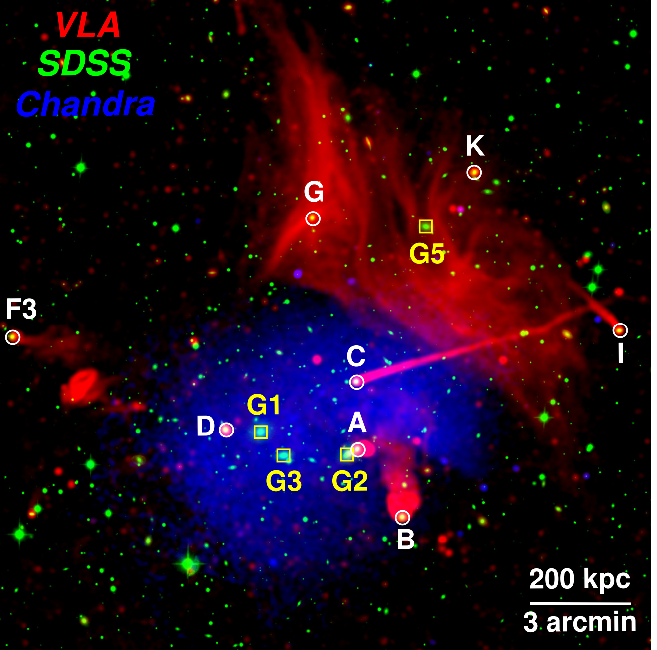
Figure 1. A three color image from red: VLA 1.4 GHz (Owen et al. 2014), green: SDSS r-band (Aguado et al. 2019), and blue: Chandra 0.7–2.0 keV including point sources. Some radio galaxies are marked with white circles and labelled with the same notation from Miller et al. (2003). Yellow boxes and labels mark the bright cluster galaxies discussed in Sec. 4.4. The bar at bottom right side shows 3 arcmin/200 kpc.
