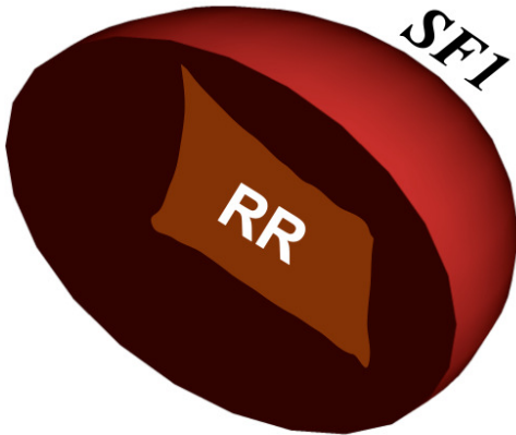
Figure 12. Sketch shows a possible geometry of SF1 and RR viewed in the plane of the sky. The SF1 is represented as a 3D spherical shell. The RR is represented as a thin layer sticking on the inner shell of SF1 that traces the underlying distribution of seed electrons. After projecting this geometry on the plane of the sky, the SF1 and RR have a apparent offset.
