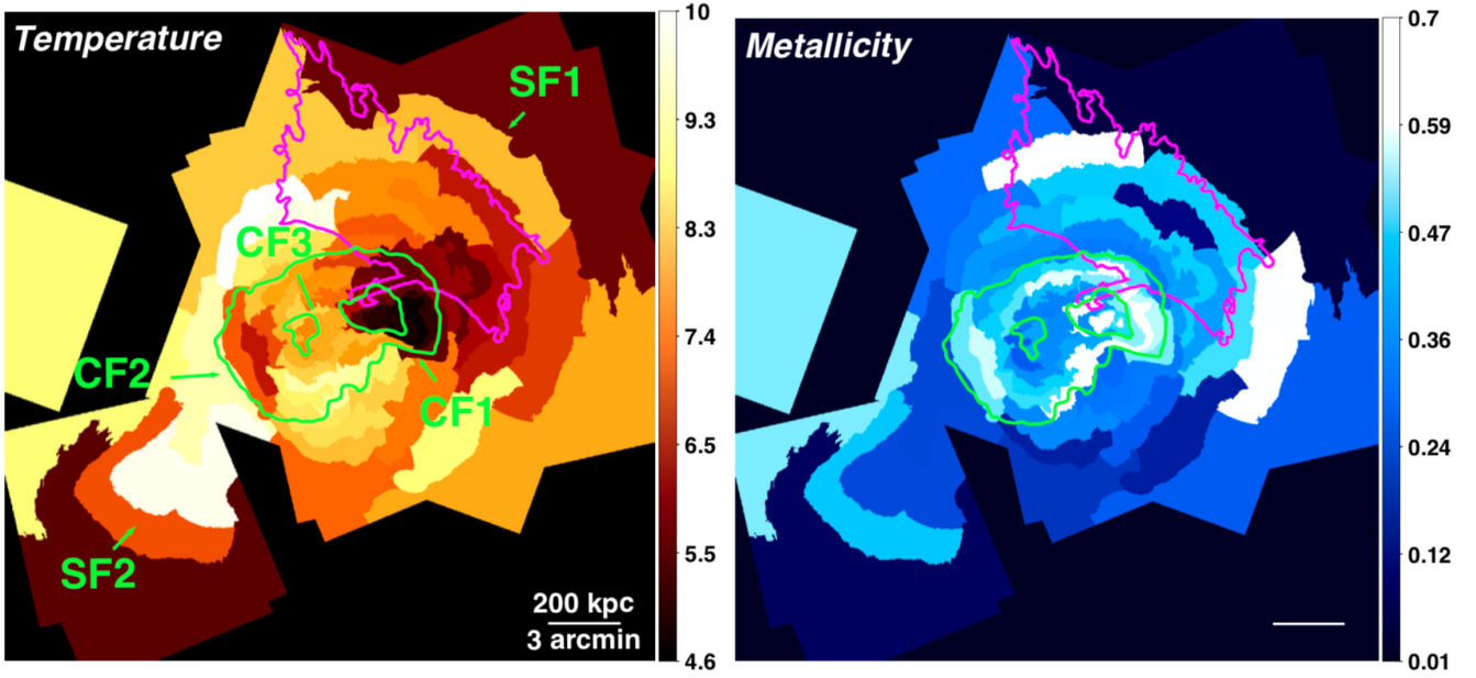
Figure 2. Left: Gas temperature map with a unit of keV. Green contours are from Chandra X-ray intensity to show two X-ray peaks in the cluster center. A magenta contour is from VLA radio intensity (Owen et al. 2014) to show an outline of the RR. Right: Gas metallicity map with a unit of Z_{\odot} .
