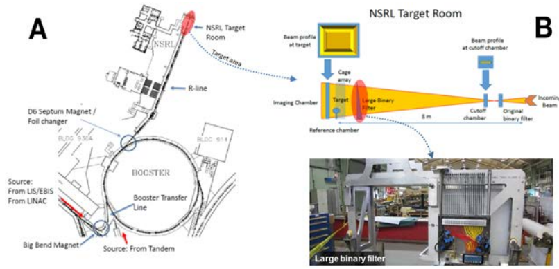
Fig 9. Facility layout of NSRL at BNL. (A) Tools to reliably control system hardware settings, from ion production by the LIS through booster injection, acceleration, extraction and delivery to the NSRL target room were developed to sequentially deliver the GCR simulator ion-energy beam combinations. (B) Position of imaging chamber behind target (top, left hand side), cut-off chamber (top, right hand side) near beam entrance to target room, and photo of large area degrader (binary filter) system (bottom) in NSRL beam line to maintain control and uniformity of 60 \times 60 cm 2 beam.
