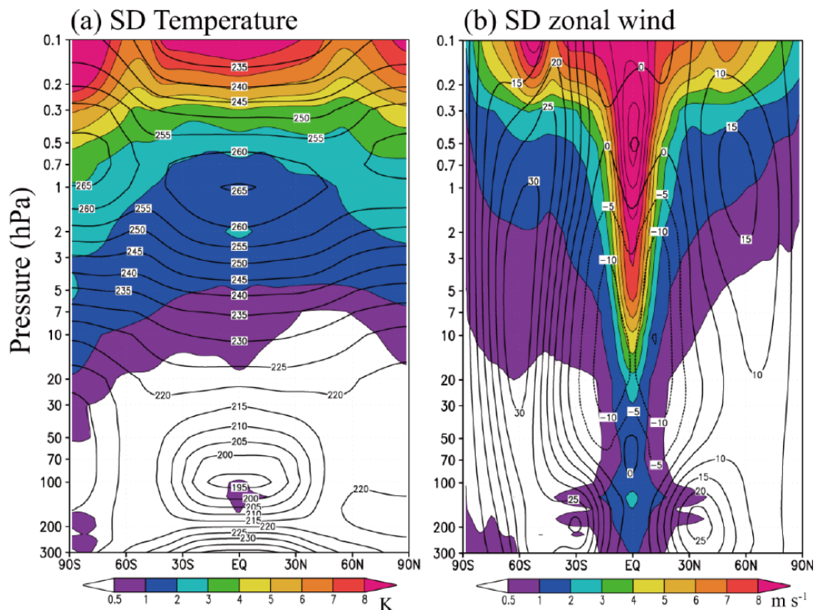
Figure 11: Latitude-altitude distribution of zonal mean and time mean (1980–2012) standard deviations (colors) of (a) temperature and (b) zonal winds for ERA-Interim, JRA-55, MERRA, and MERRA-2. Overlays are annually averaged (a) zonal-mean temperatures and (b) zonal winds (westerlies solid, easterlies dotted). See also Kawatani et al. (2016).
