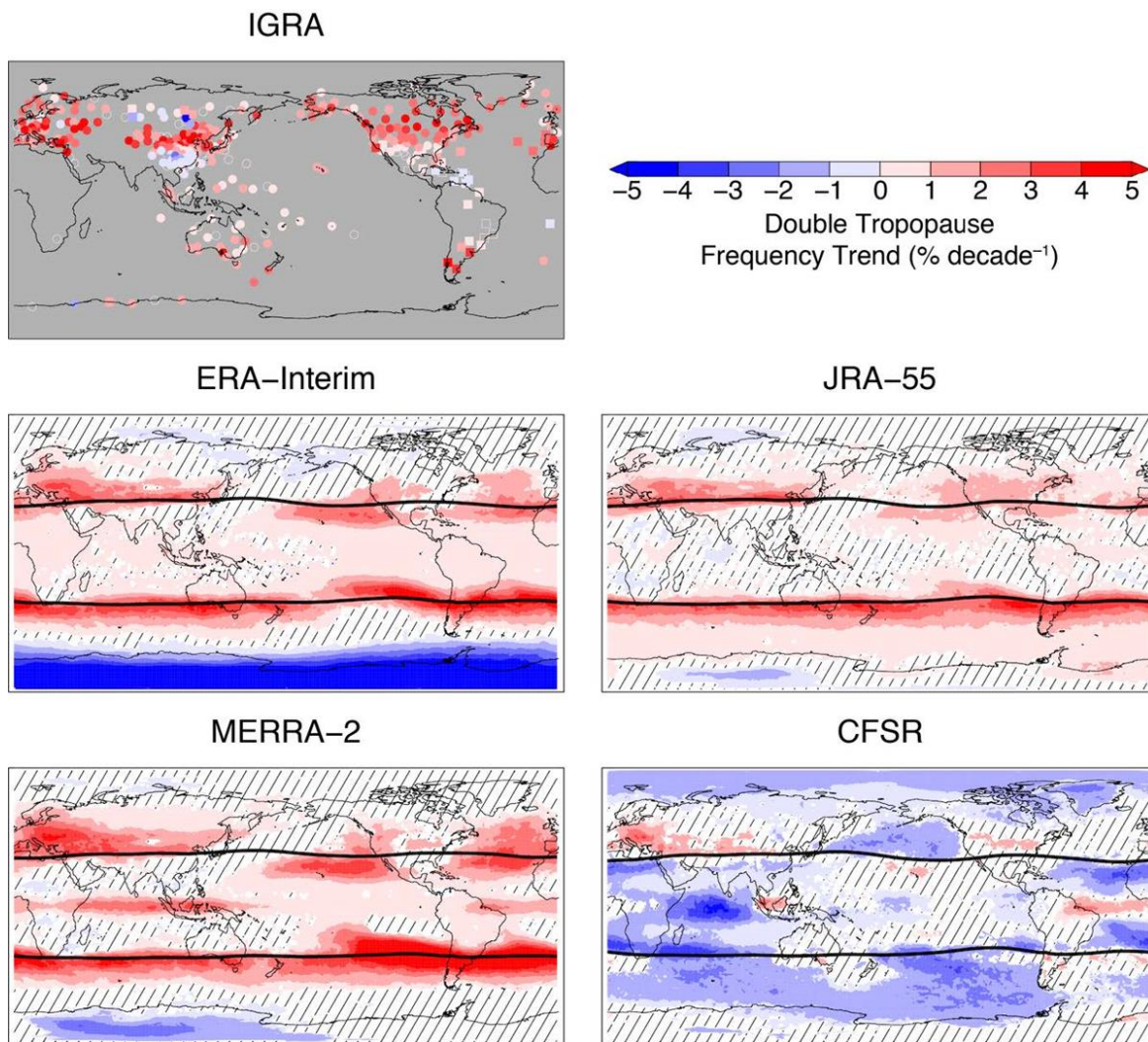
Figure 7: Double tropopause tendencies from radiosonde data and four reanalyses for 1980 through 2015 (Xian & Homeyer, 2018).
