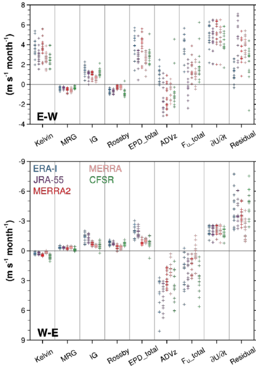
Figure 9: Terms in the QBO zonal-mean zonal momentum budget from 5N to 5S at 30 hPa, averaged over the easterly-to-westerly and westerly-to-easterly transitions during 1981-2010. Note that the y-axis direction is reversed in the bottom panel. See also Kim & Chun (2015).
