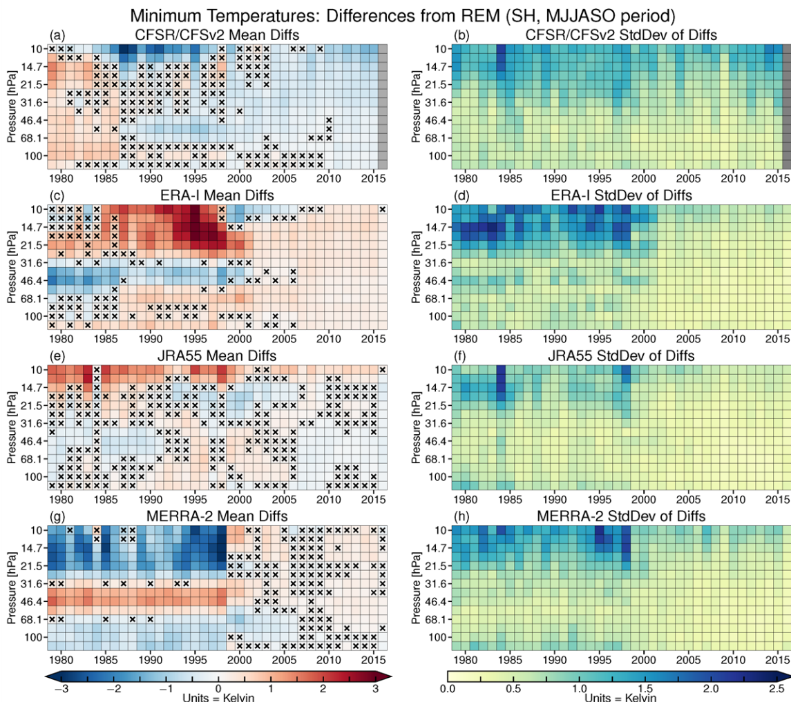
Figure 10: Averages (left) and standard deviations (right) of polar minimum temperature differences for each reanalysis from an REM for the 1979–2015 SH winters. X's indicate differences that are insignificant according to a bootstrapping analysis. See Lawrence et al. (2018).
