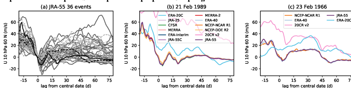
Figure 6: Pre- and post-satellite era Sudden Stratospheric Warmings. (a) Winds from JRA-55 for 36 sudden warmings in satellite era (dark grey) and radiosonde era (light grey, dashed lines) and for one (b) satellite-era and one (c) radiosonde era event for all reanalyses (shown as black line solid and dashed lines, respectively, in (a)).
