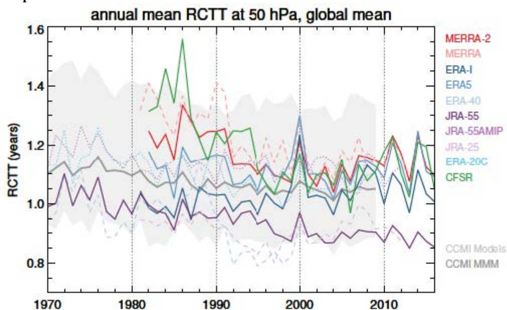
Figure 5: Residual circulation transit time (RCTT) at 50 hPa from reanalyses compared with range from Chemistry Climate Model Initiative models.
