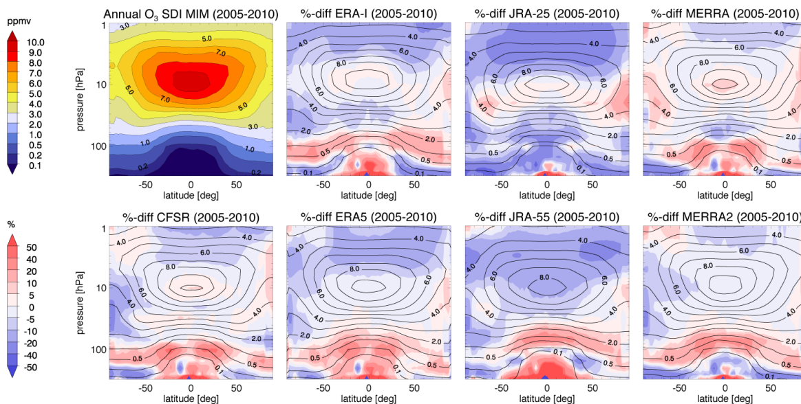
Figure 4: Reanalysis ozone compared with SPARC Data Initiative Climatology.
