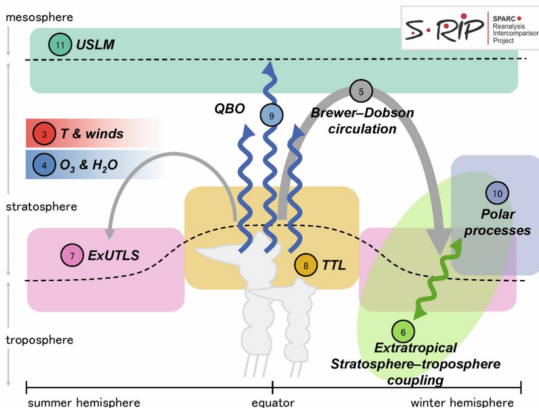
Figure 1: S-RIP chapter schematic.
