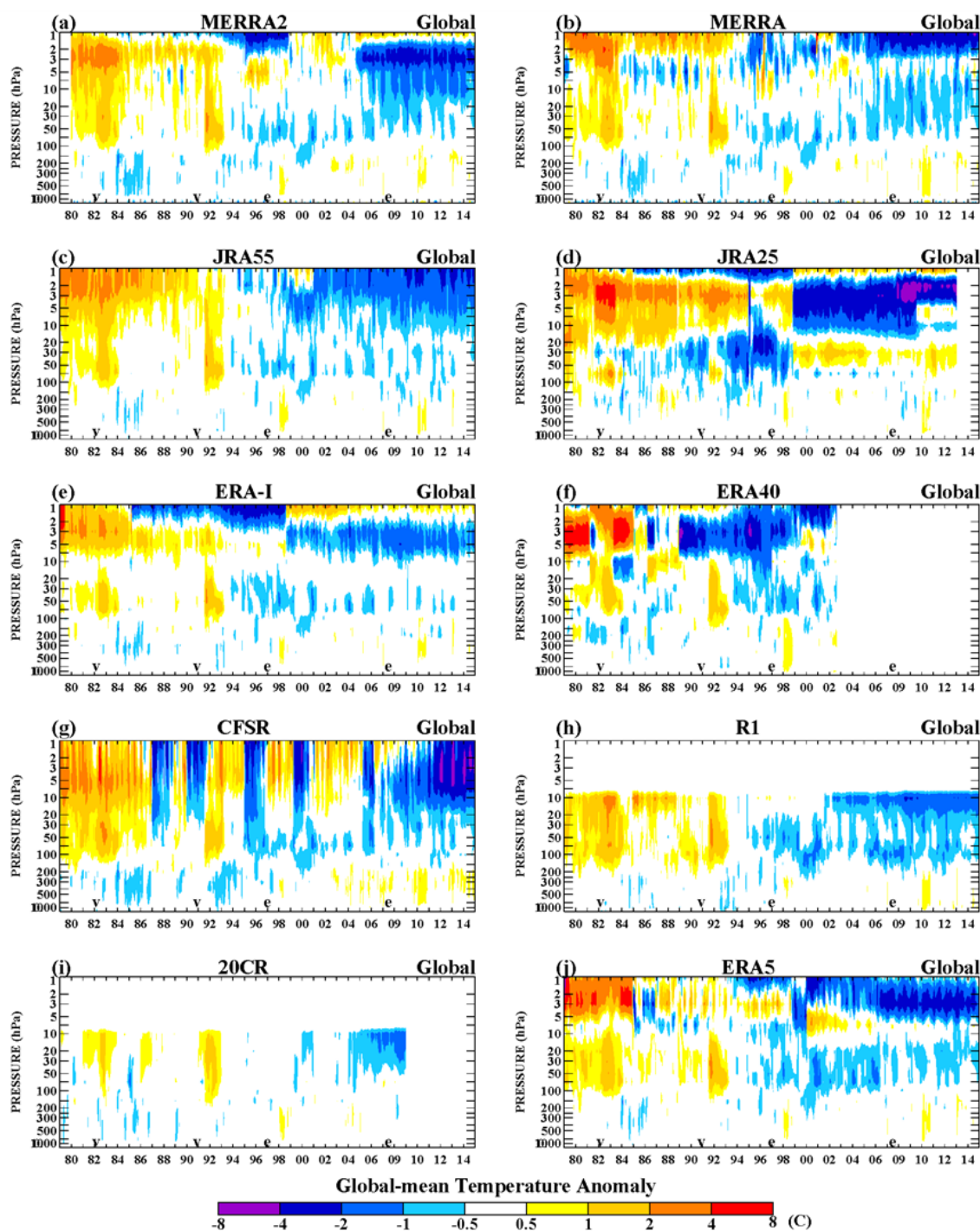
Figure 3: Zonal mean reanalysis temperature differences from a reanalysis ensemble mean (REM).
