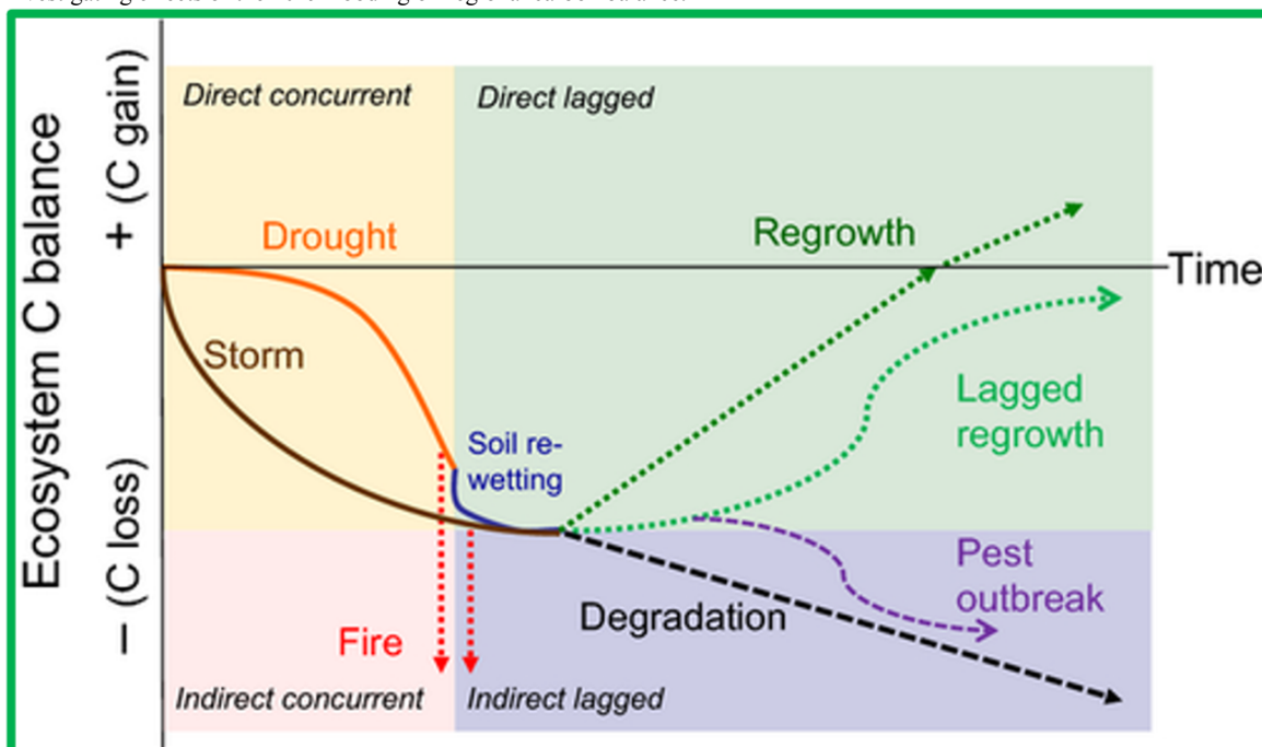
Figure 2. Climate extremes affect ecosystem carbon emissions directly and indirectly. Those effects may be concurrent or lagged. In the case of flooding we could reasonably expect direct concurrent influence on carbon; however, the case studies to support this are lacking and require further investigation. Source: Frank et. al. 2014 ( https://onlinelibrary.wiley.com/doi/full/10.1111/gcb.12916 ).
