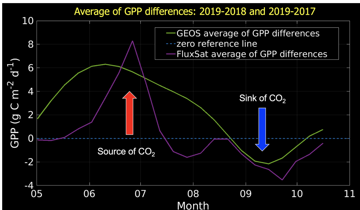
Figure 14. GEOS and FluxSat GPP differences between 2019 and 2018 as well as 2017.
