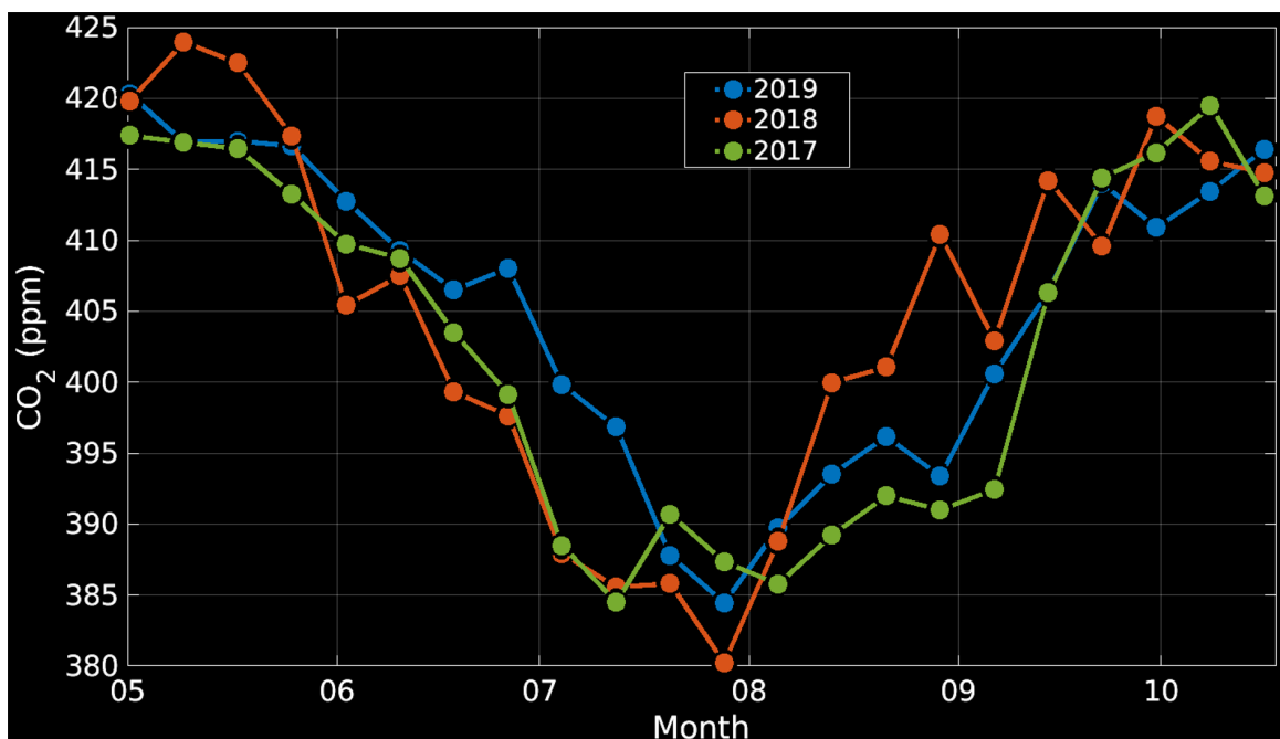
Figure 11. Trend-adjusted May-October weekly CO 2 at WBI tower for 2017-2019.
