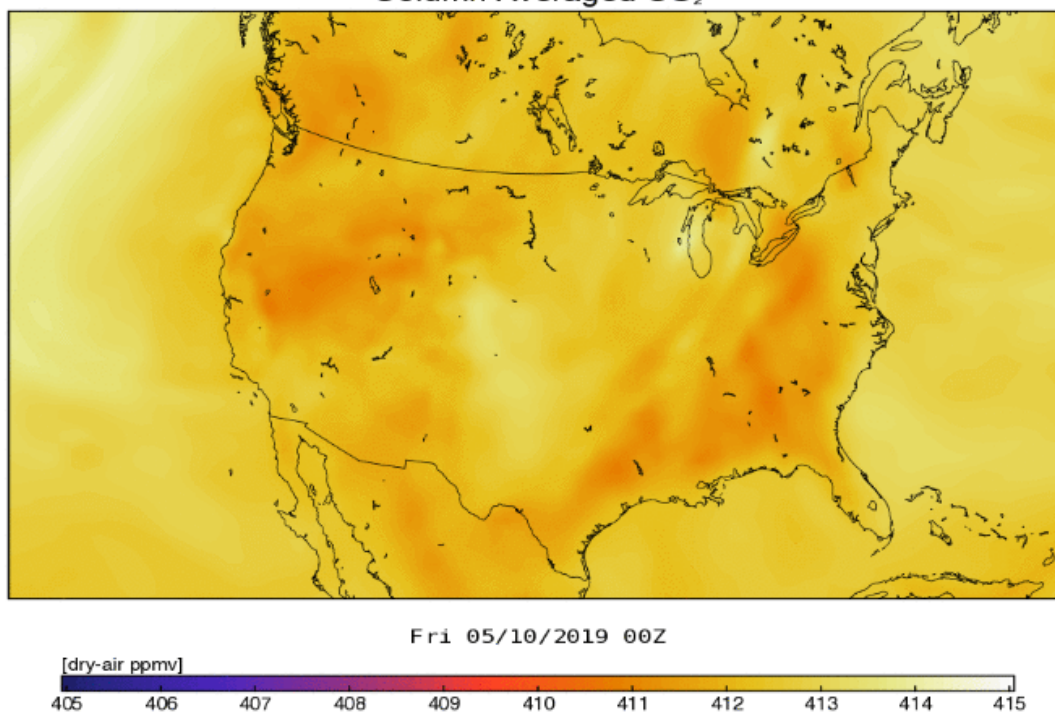
Figure 6. We utilize NASA GEOS model with low-order flux inversion (LOFI) module to simulate CO 2 over the region of interest (Weir et al., 2020 ( https://acp.copernicus.org/preprints/acp-2020-496/ )). The CO 2 forecasts are available at https://fluid.nccs.nasa.gov/carbon ( https://fluid.nccs.nasa.gov/carbon ).
