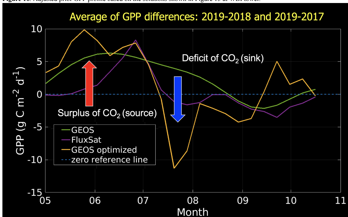
Figure 16. Adjusted prior GPP profile based on the solutions shown in Figure 15 at WBI tower.
