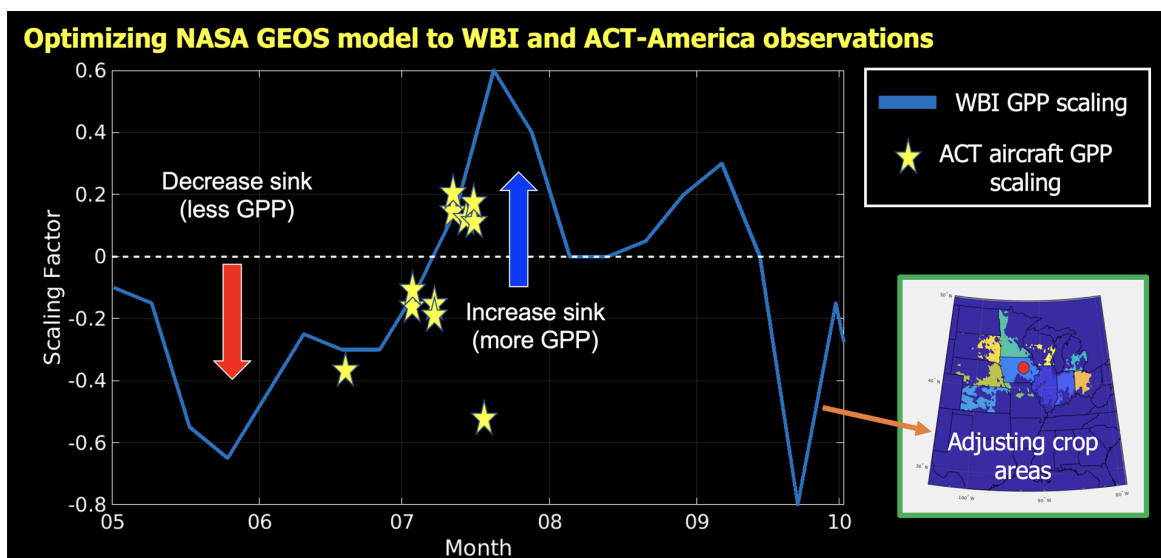
Figure 15. Optimization solutions for GEOS model crop GPP tracer (crop areas are shown on the map) for WBI tower and ACT-America flights indicated as percentage (or scaling factor) of the prior GPP profile.
