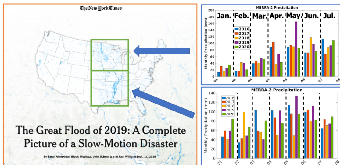
Figure 1. A major flooding of midwestern and southern US in 2019 lead to a widespread damage to property and local ecosystem. The MERRA-2 monthly precipitation plots indicate that majority of flooding in the region occurred in the month of May, where the US Midwest received close to twice its regular monthly amount of precipitation. The flood was so dramatic that it generated a lot of press.
