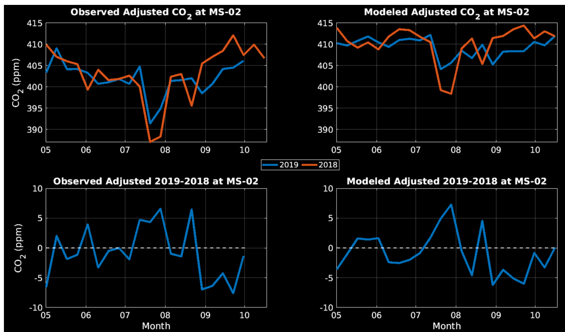
Figure 18. Preliminary results from the MS-02 tower in Mississippi indicates lesser influence of 2019 flood on May-June CO 2 in both observations and model. However, there seems to be slightly decreased uptake in July, perhaps continued rains in June in the South did have some effect on non-crop vegetation.
