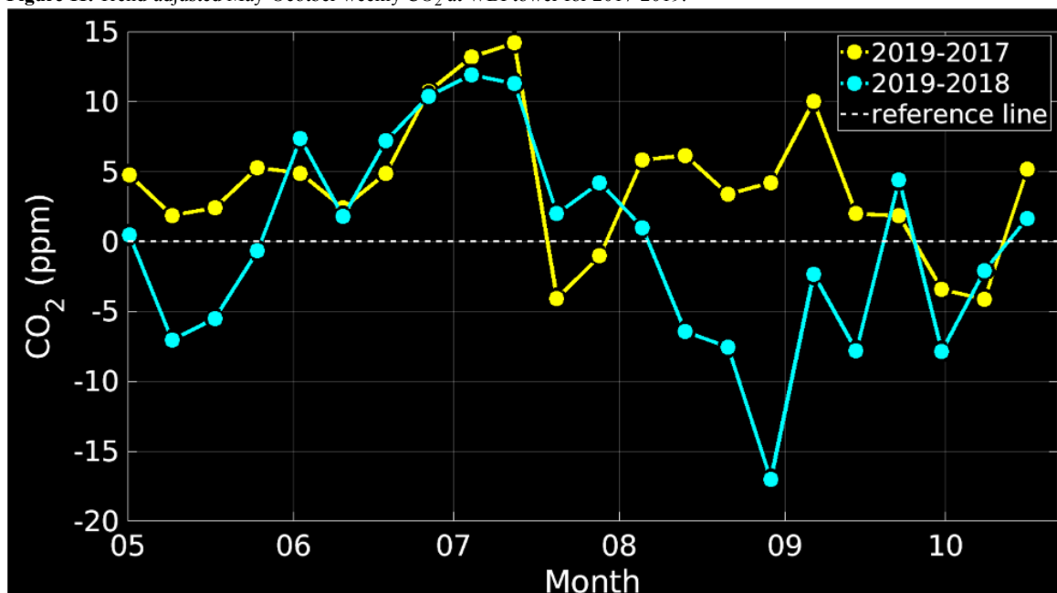
Figure 12. Differences between the CO 2 cycles at WBI shown in the Figure 11. Note that the post flooding period indicates surplus of atmospheric CO 2 in 2019 from mid-June until about mid-July.
