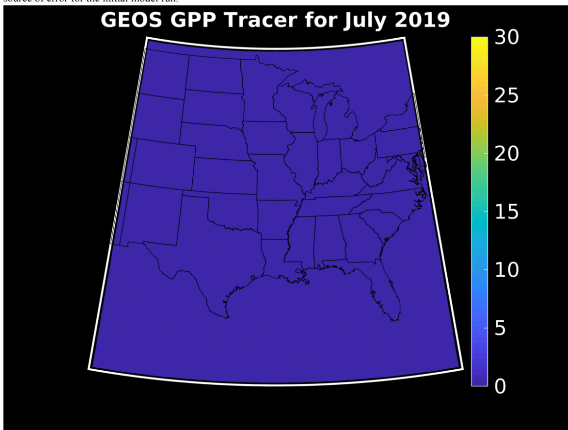
Figure 8. Crop areas that significantly affect WBI are used to derive GPP tracer from the model. The tracer then is used to optimize the model. Crop data from (USDA) indicates that it was significantly affected by the flooding and therefore is a primary source of error for the initial model run.
