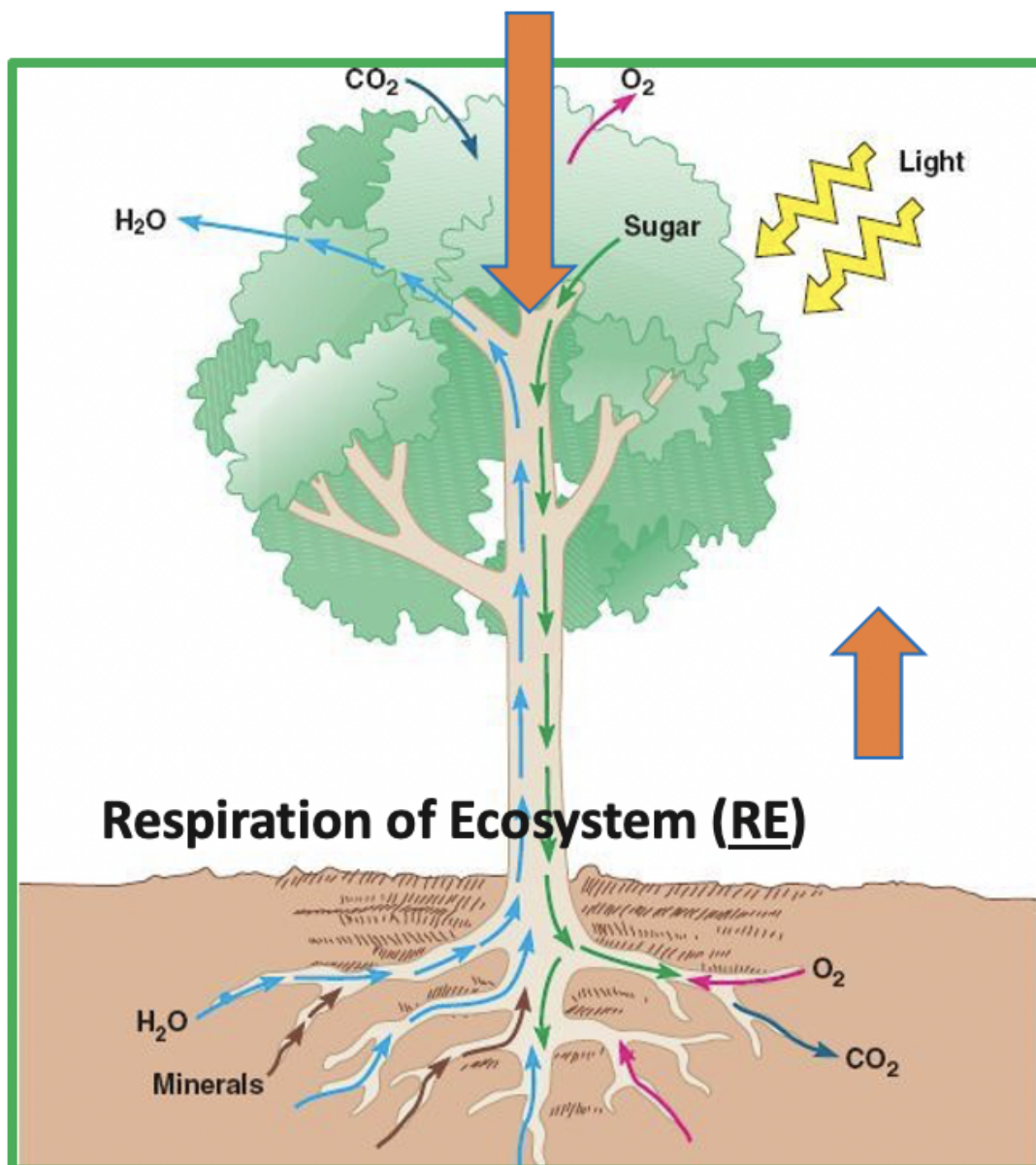
Figure 4. Land sink is mainly determined by a balance between gross primary production (GPP) and ecosystem respiration (RE). GPP is the carbon assimilated by plants in the presence of light and it is an atmospheric \text{CO}_2 sink term. RE is a source of \text{CO}_2 from plants and tends to vary much less between day and night in comparison to GPP. The difference between RE and GPP is known as net ecosystem exchange (NEE).
