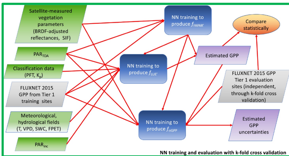
Figure 7. Additionally we use FluxSat GPP product, which utilizes parameters derived from MODIS combined with FLUXNET data and machine learning to estimate GPP (Joiner et al., 2020 ( https://www.sciencedirect.com/science/article/pii/S0168192320301945#bib0094 )).
