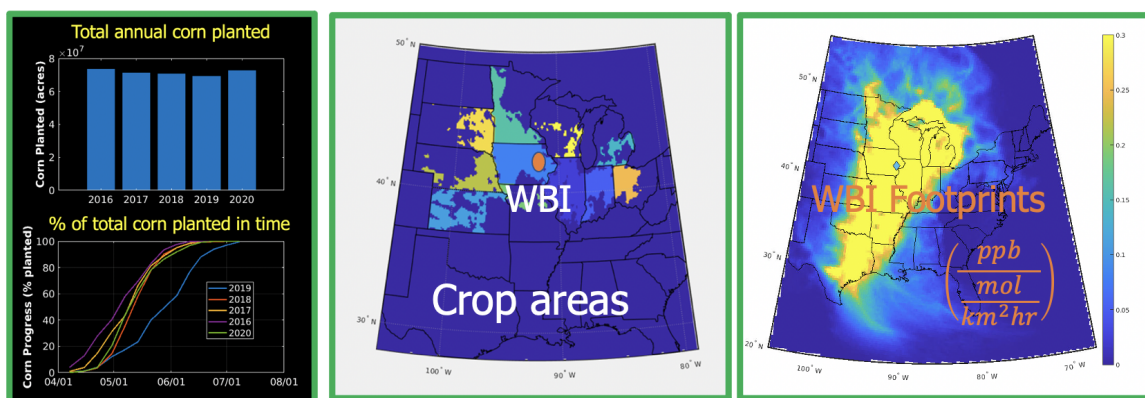
Figure 8. Crop areas that significantly affect WBI are used to derive GPP tracer from the model. The tracer then is used to optimize the model. Crop data from (USDA) indicates that it was significantly affected by the flooding and therefore is a primary source of error for the initial model run.
