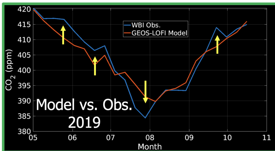
Figure 10. Schematic of the model-to-observation optimization step at WBI tower. Similar principle is used for the ACT-America 2019 flights over the Midwest.
