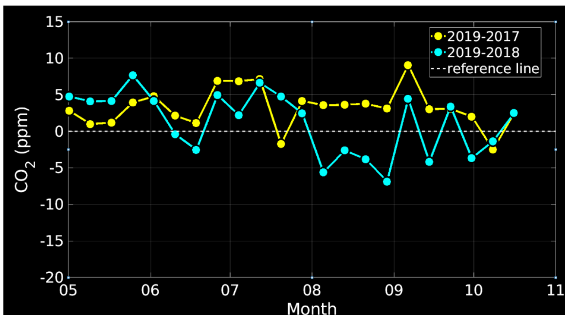
Figure 13. This figure is the same as Figure 12 only using NASA GEOS model simulations at WBI. Overall it has similar messages as Figure 12, but its magnitude and timing are noticeably off.
