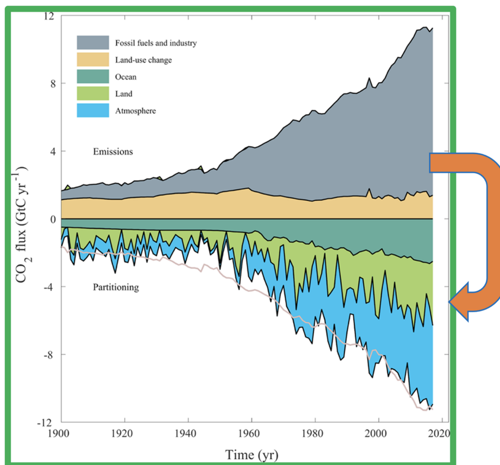
Figure 3. Large orange arrow on the right side indicates transfer of carbon from fossil fuels and land use change into 3 distinct pools: 1) ocean, 2) land, and 3) atmosphere. Rapid increase of CO 2 in the atmosphere “pool” over the past 100 years is of great concern as this process significantly affects Earth's radiation balance.
