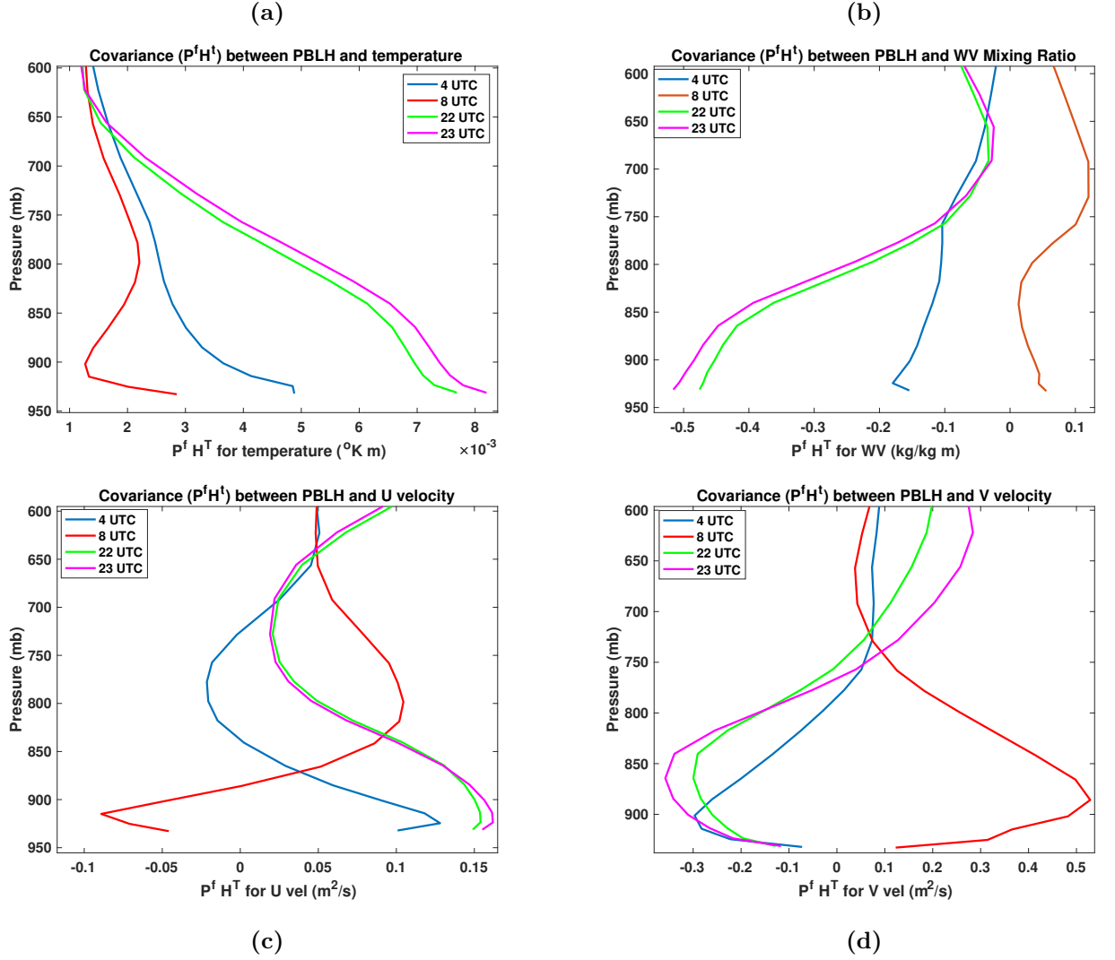
Figure 8. Covariance \mathbf{P}^f \mathbf{H}^T between PBLH and temperature (a), water vapor (b), U velocity (c) and V velocity (d), at times 4, 8, 22 and 23 UTC, for PBL physics model MYHH.
