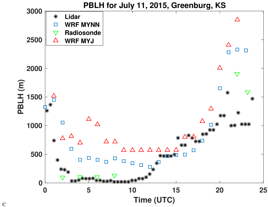
Figure 1. PBLH vs UTC time for July 11, 2015 for lidar backscatter (black *), WRF model - MYJ (red triangles), WRF model - MYNN (blue squares), and radiosonde observations using parcel method (green triangles).
